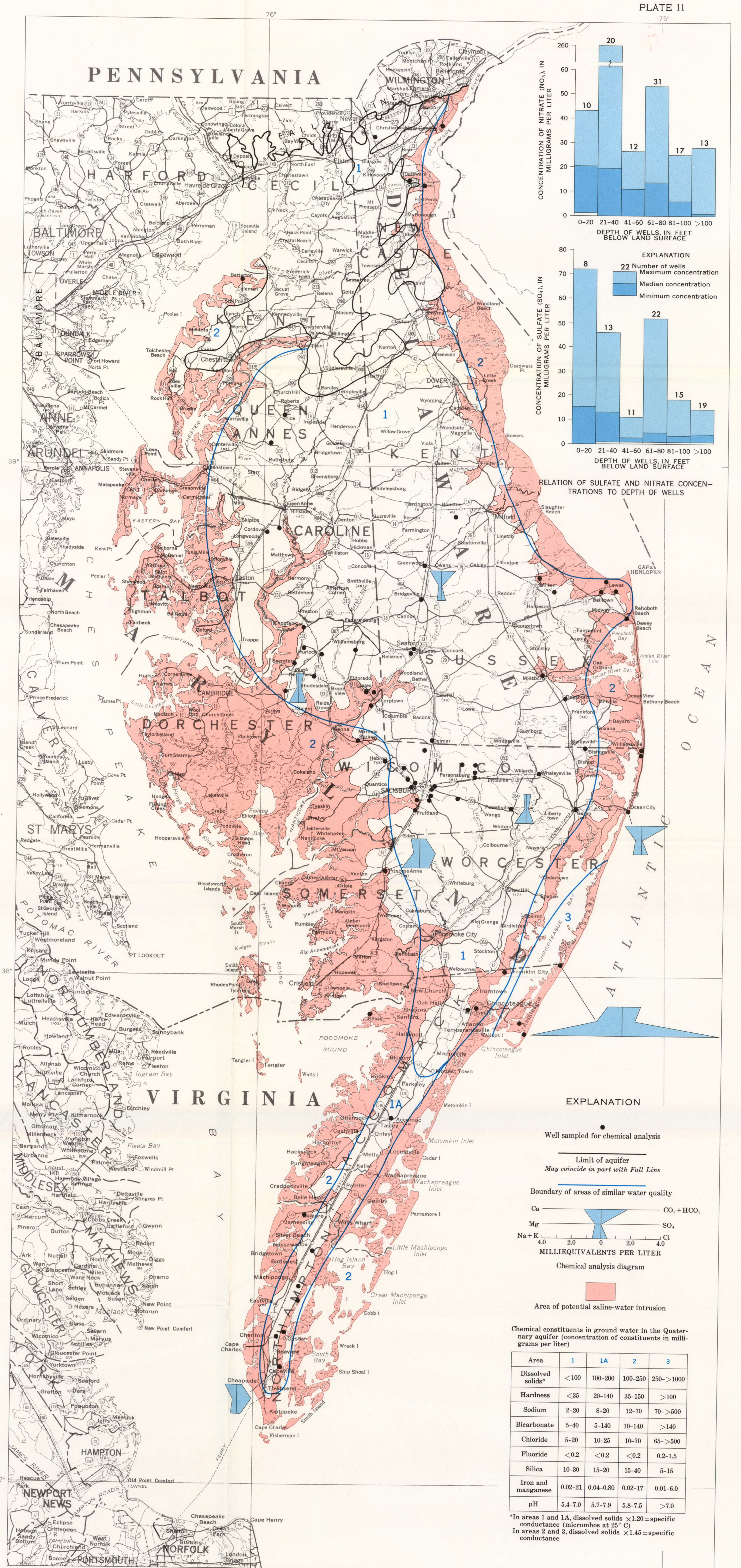
CHEMICAL QUALITY OF GROUND WATER AND AREA OF POTENTIAL SALINE-WATER INTRUSION IN THE QUATERNARY AQUIFER
