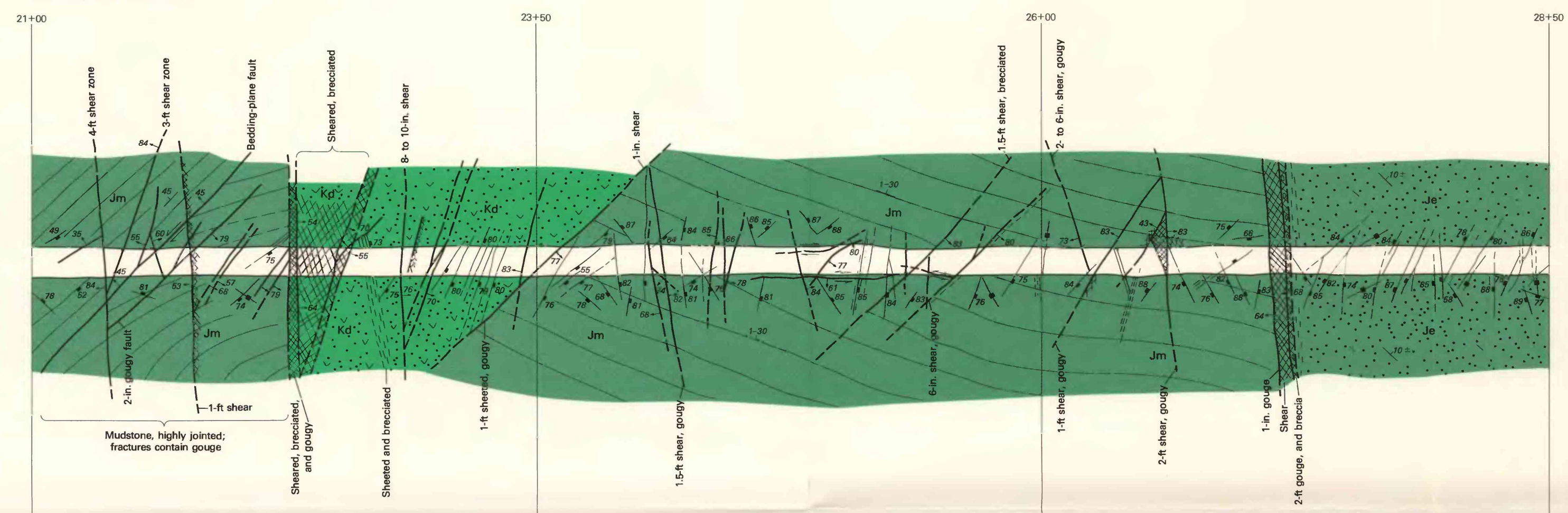
GEOLOGIC PLAN AT SPRING-LINE ELEVATION
