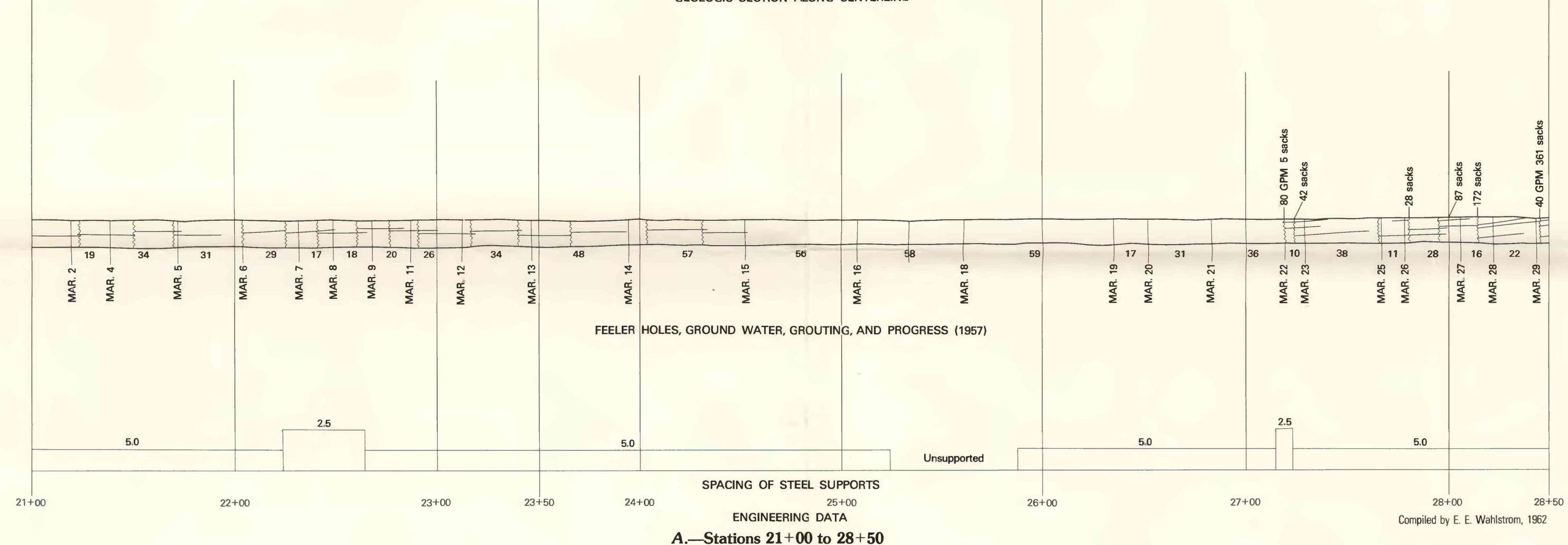
A.—Stations 21+00 to 28+50
