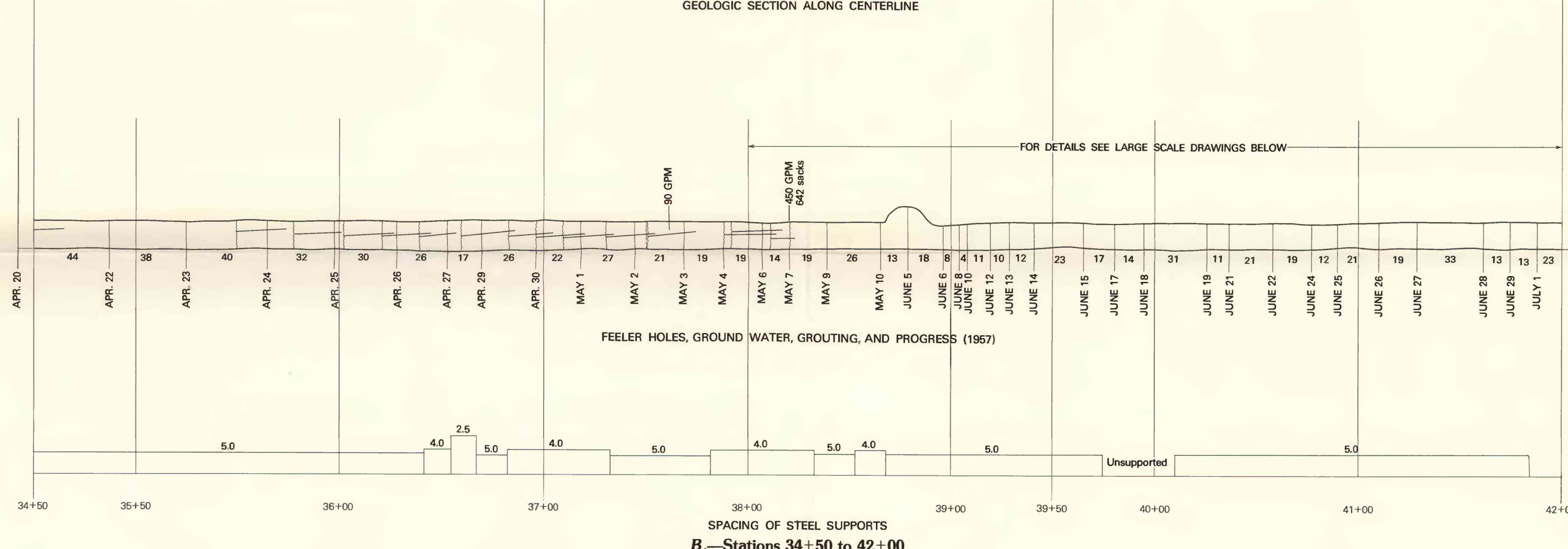
B.—Stations 34+50 to 42+00
