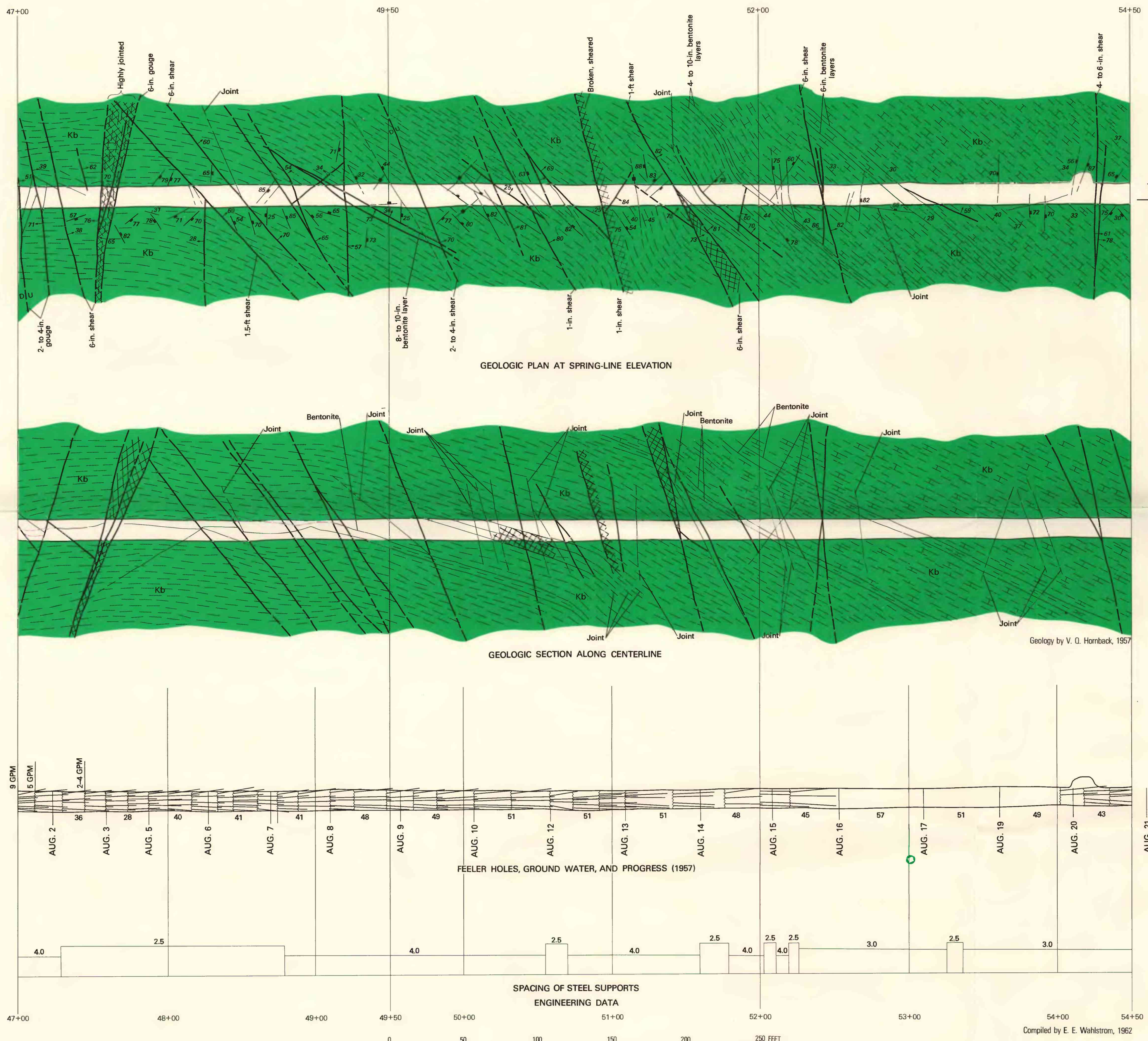
A.—Stations 47+00 to 54+50
