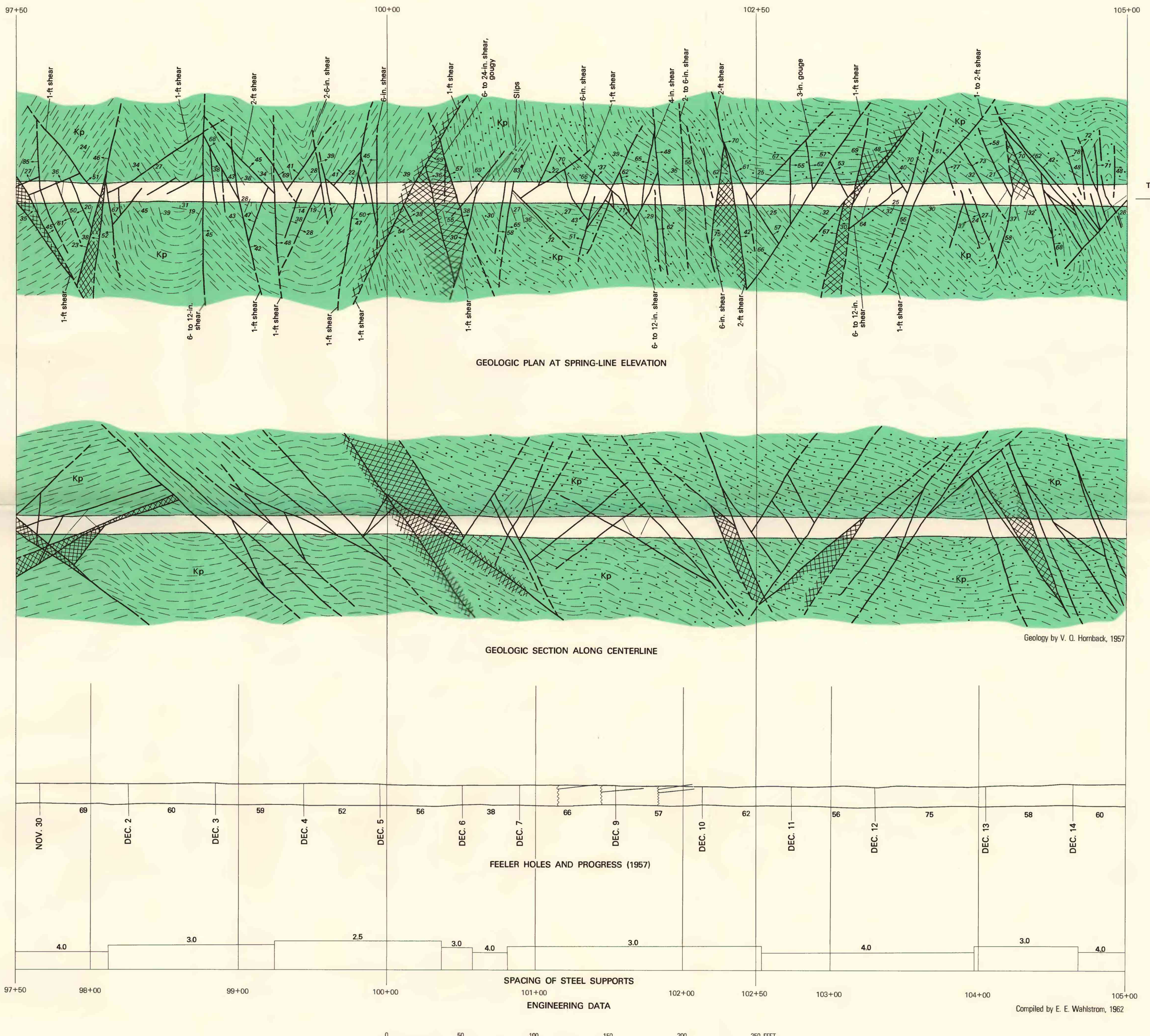
B.—Stations 97+50 to 105+00
