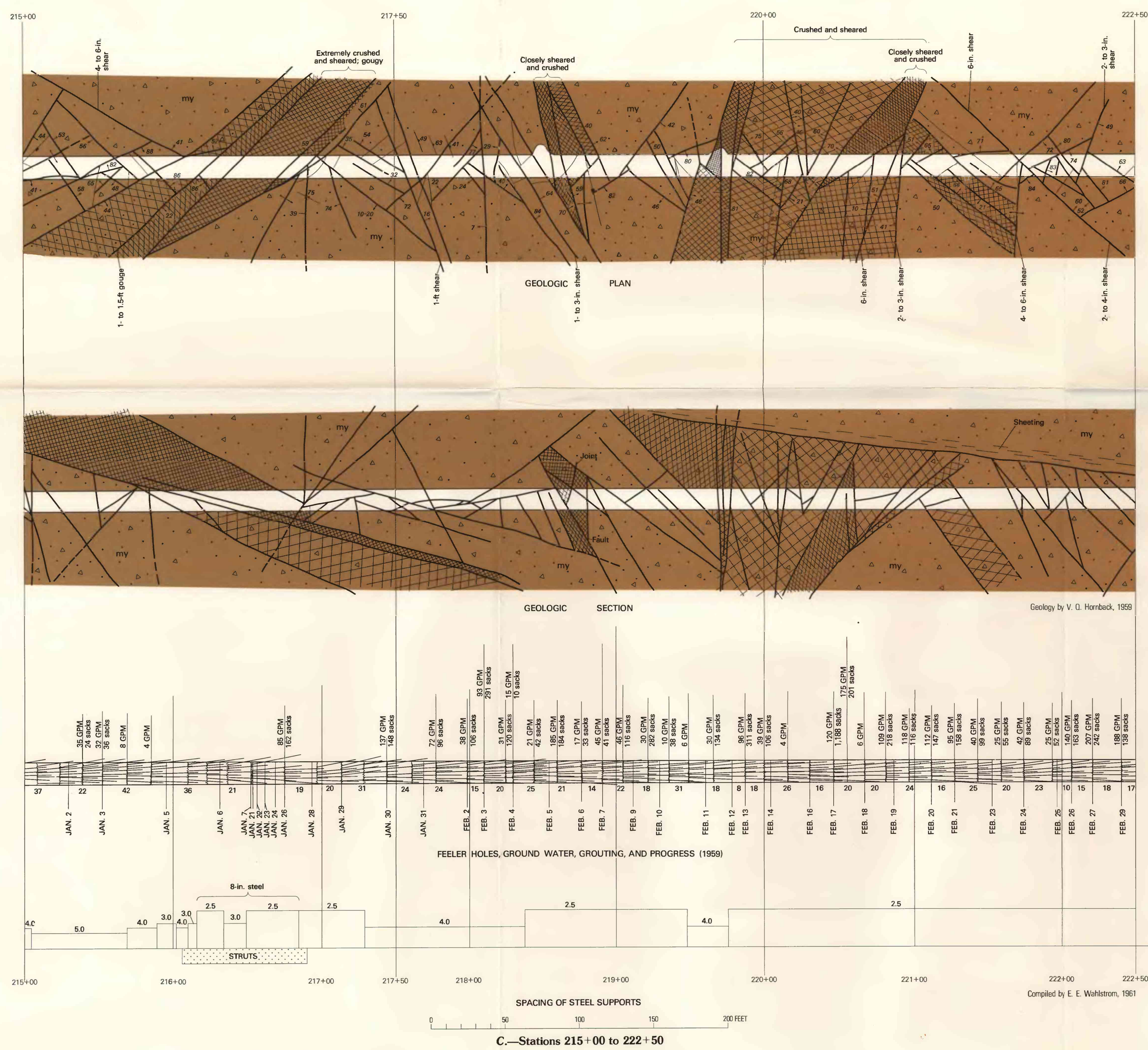
DETAILED GEOLOGIC PLANS AND SECTIONS, AND ENGINEERING DATA, STATIONS 180+00 TO 187+50, STATIONS 200+00 TO 207+50, STATIONS 215+00 TO 222+50, AND STATIONS 240+00 TO 247+50, ROBERTS TUNNEL, SUMMIT COUNTY, COLORADO
