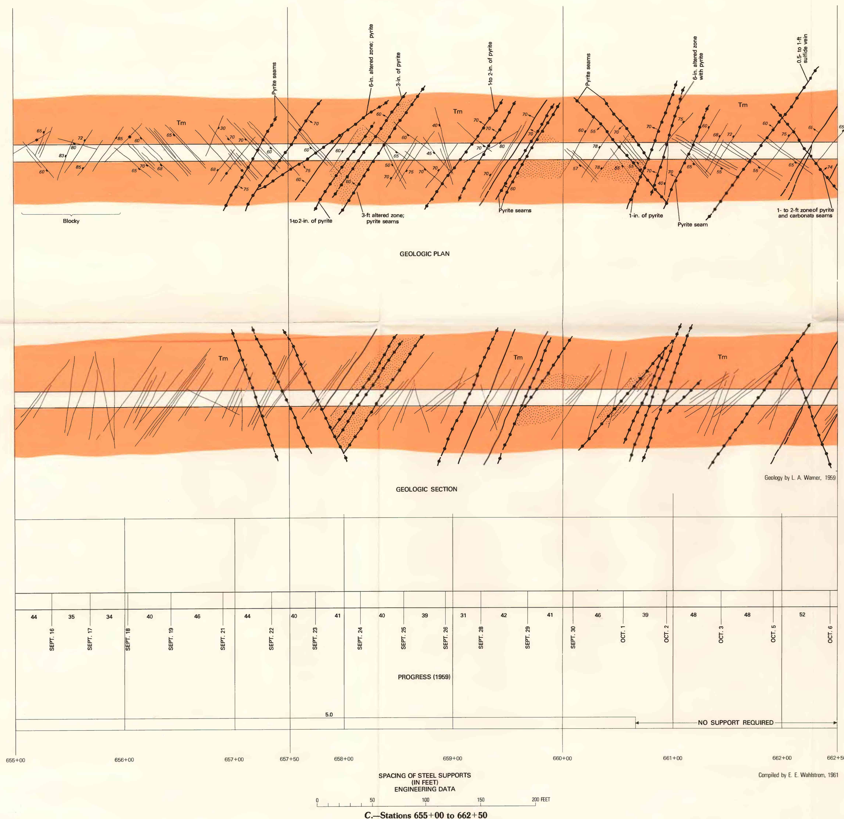
DETAILED GEOLOGIC PLANS AND SECTIONS, AND ENGINEERING DATA, STATIONS 527+50 TO 535+00, STATIONS 632+50 TO 640+00, STATIONS 655+00 TO 662+50 AND STATIONS 685+00 TO 692+50 ROBERTS TUNNEL SUMMIT COUNTY COLORADO
