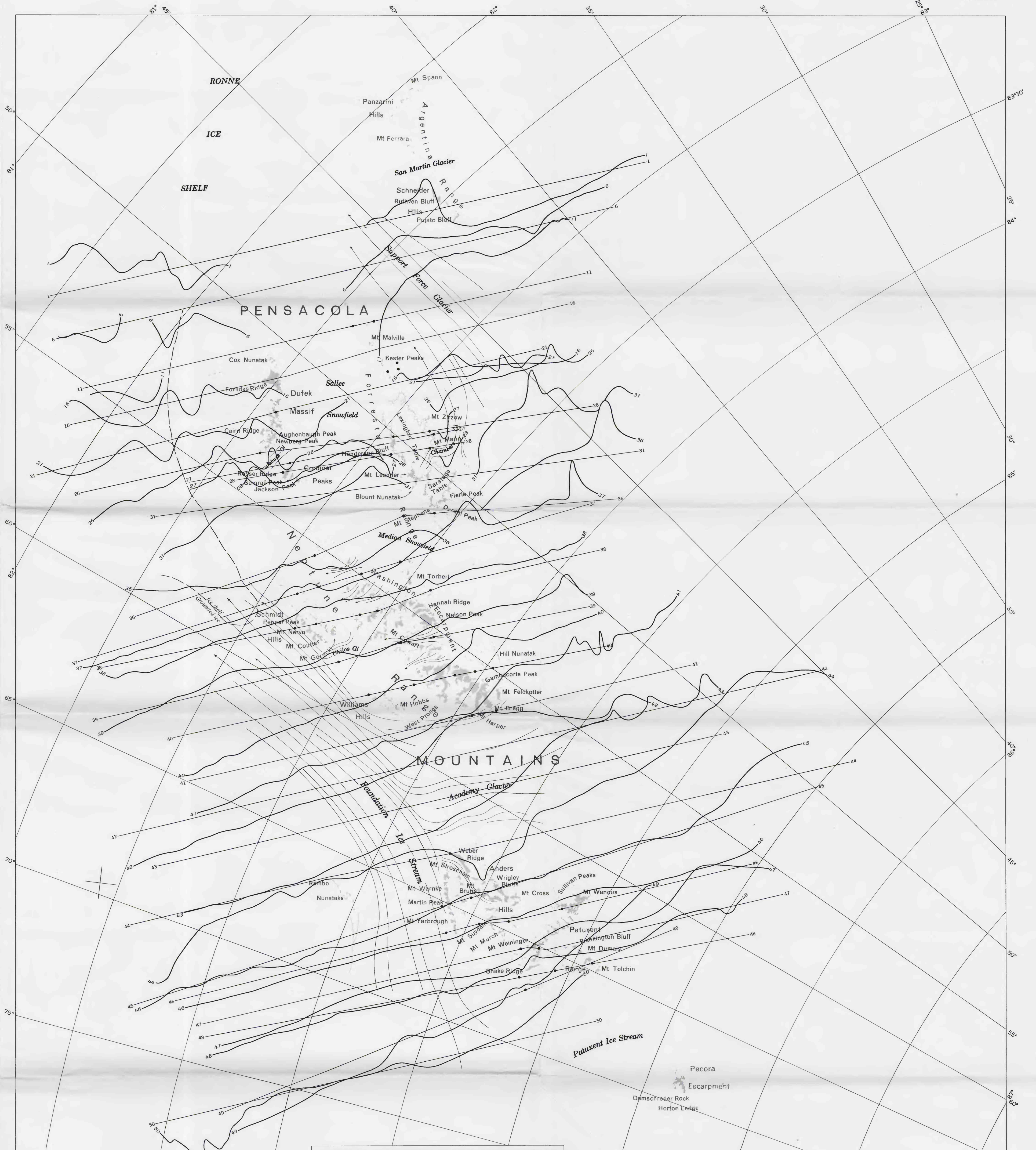
A. TOTAL MAGNETIC INTENSITY PROFILES
