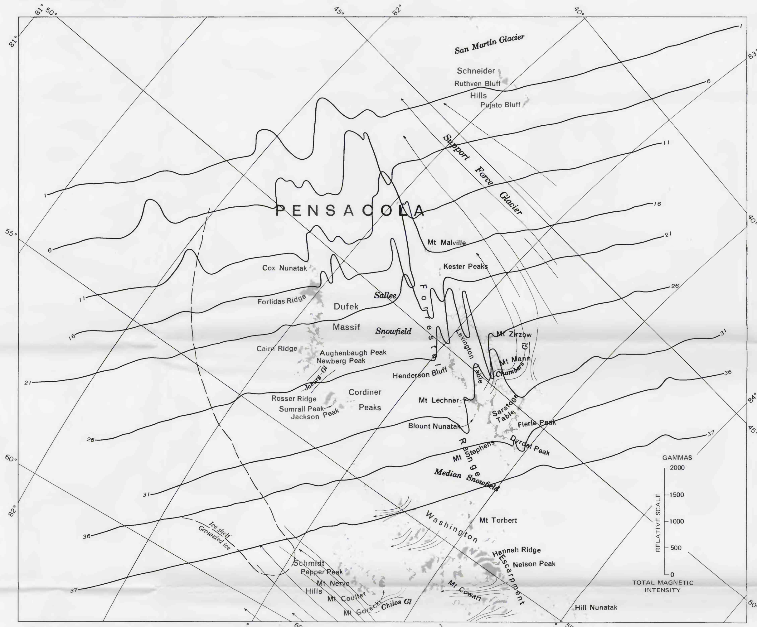
B. TOTAL MAGNETIC INTENSITY PROFILES OVER THE DUFEK INTRUSION
