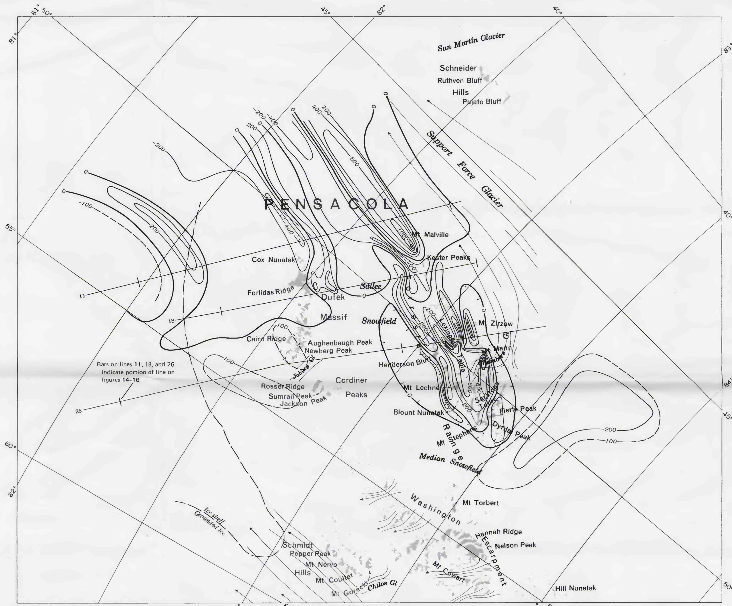
C. RESIDUAL TOTAL MAGNETIC INTENSITY OVER THE DUFEK INTRUSION
