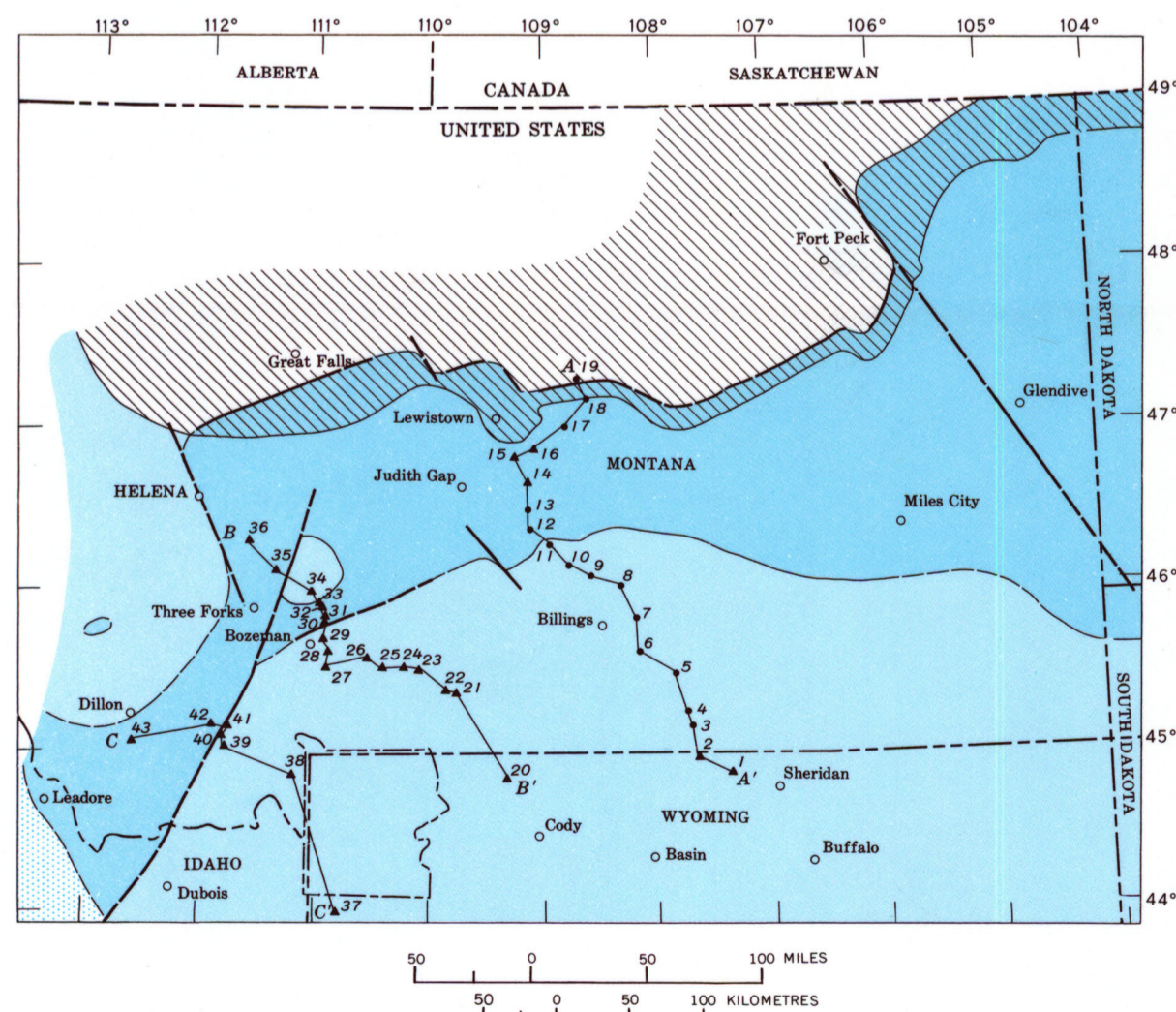
PALEOGEOLOGIC MAP OF ROCKS BENEATH AMSDEN GROUP SHOWING LOCATION OF STRATIGRAPHIC SECTIONS (FROM MAUGHAN AND ROBERTS, 1967, PL. 3)
