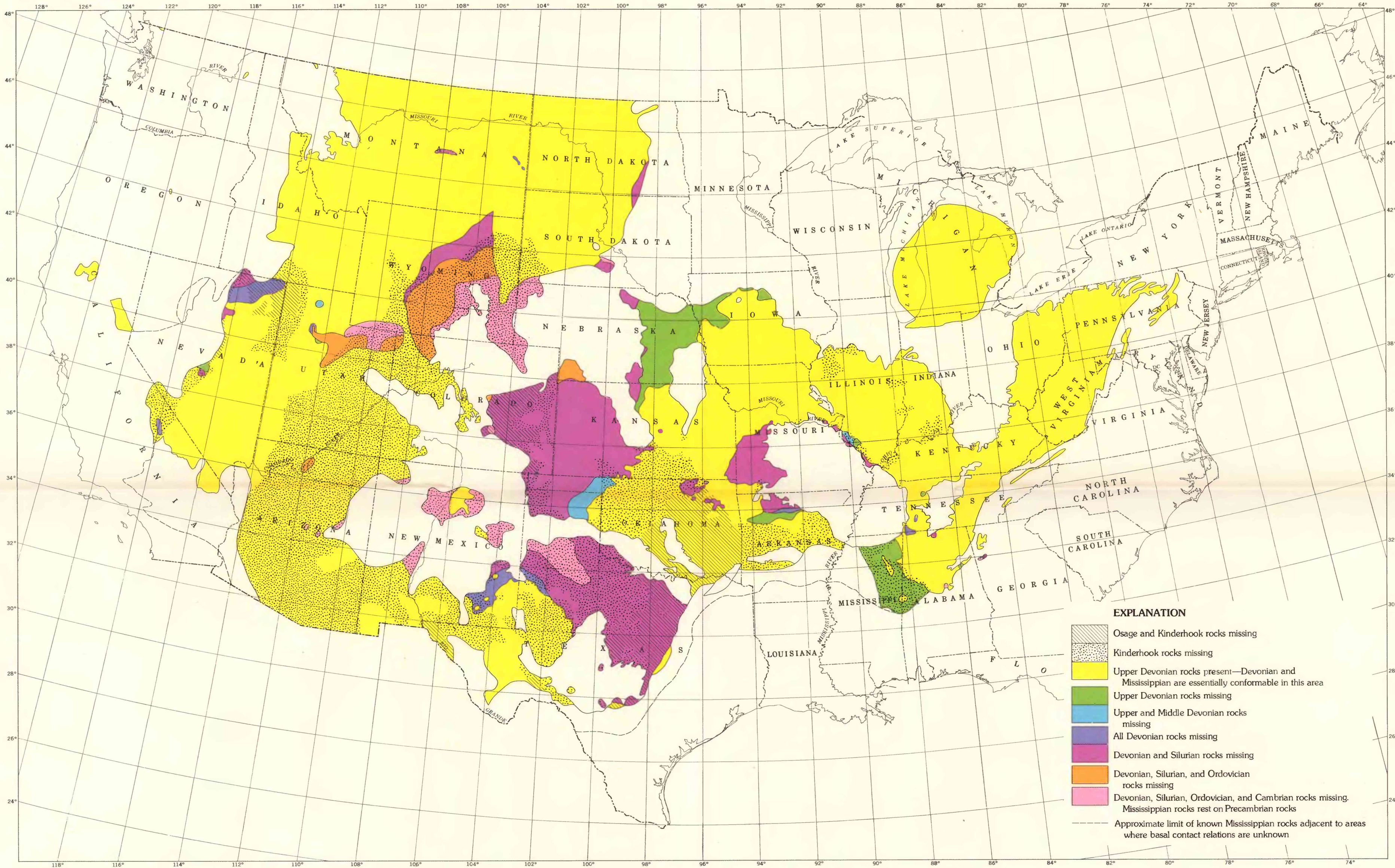
GENERALIZED MAP SHOWING TIME VALUE OF DISCONFORMITIES AT THE BASE OF THE MISSISSIPPIAN SYSTEM
