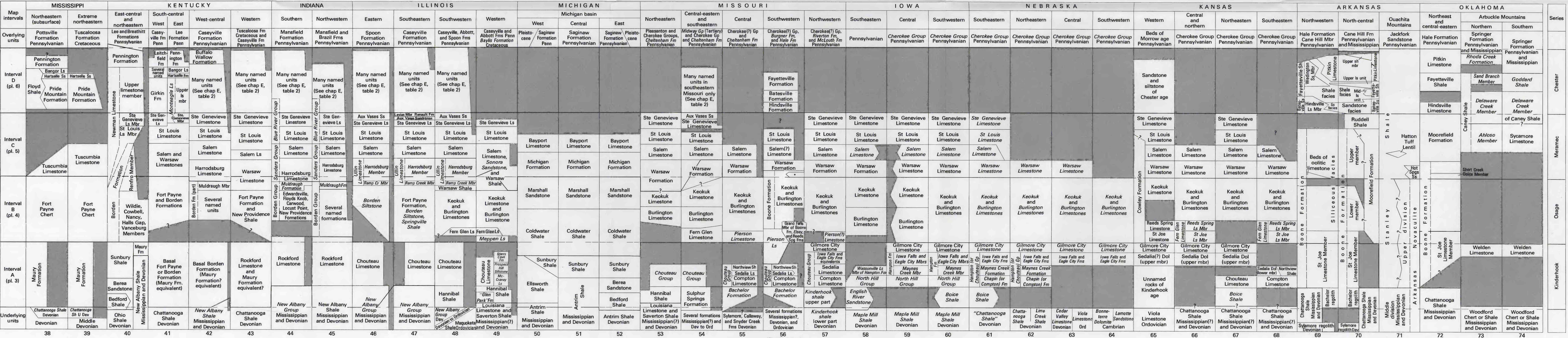
GENERALIZED CHART SHOWING STRATIGRAPHIC UNITS IN MAJOR MISSISSIPPIAN SUBDIVISIONS
