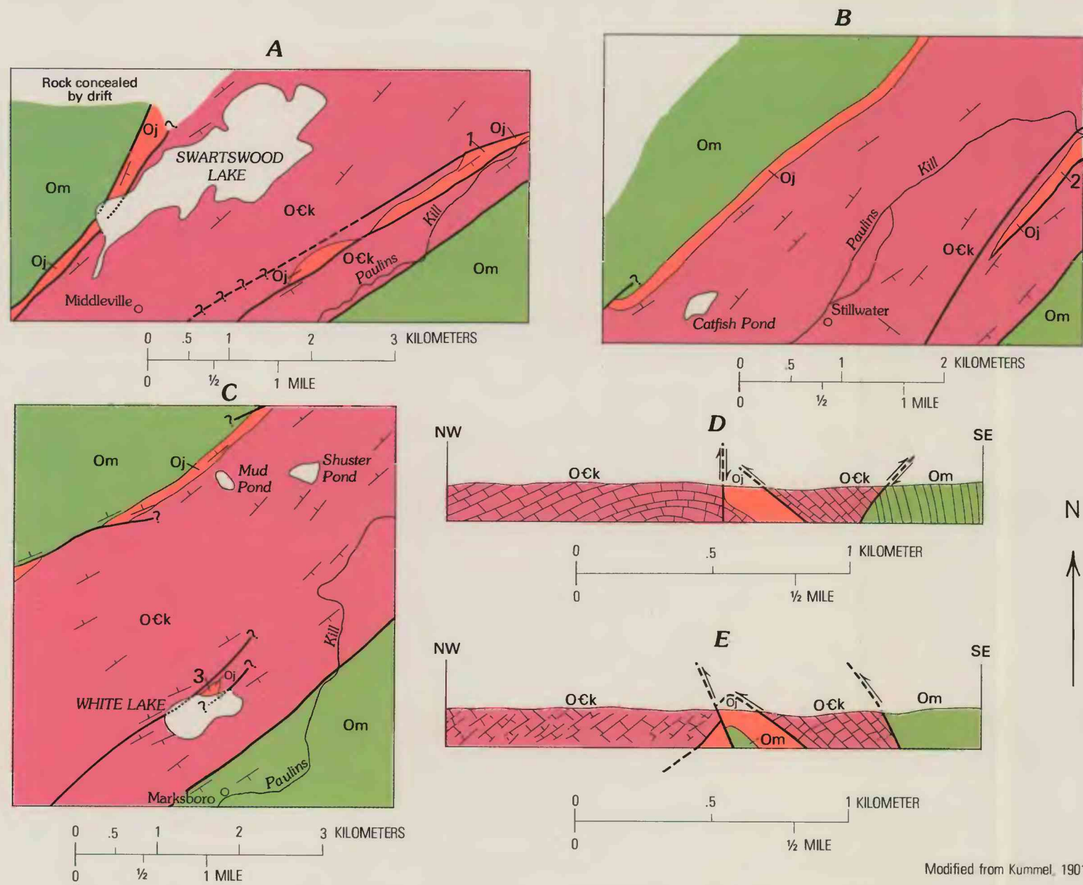
Note: A , Swartwood Lake area; B , Stillwater area; C , Marksboro or White Lake area; D , Diagrammatic section through Swartwood Lake area as interpreted by Kummel (1901); E , same section as D using nappe interpretation; 1, area of plate 2B; 2, area of plate 2C; and 3, area of plate 2D
