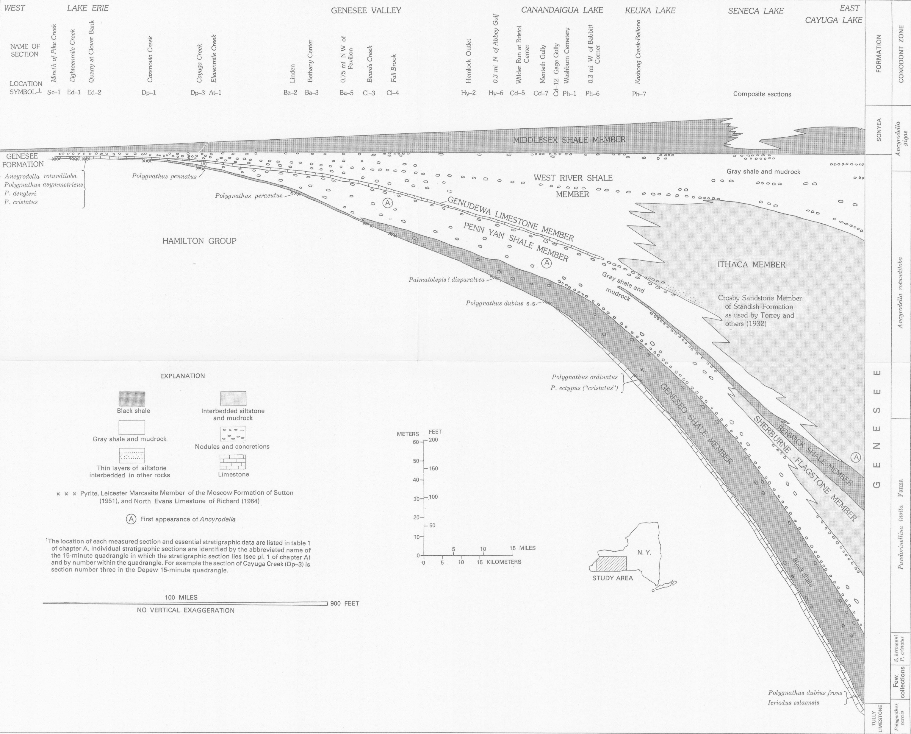
DIAGRAM SHOWING THE SEQUENTIAL APPEARANCE OF CONODONT SPECIES IN THE BASAL BEDS OF THE GENESEE FORMATION, IN WESTERN AND CENTRAL NEW YORK
