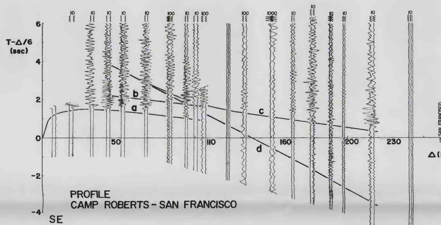
FIGURE 65.—Record section of the profile from Camp Roberts (2) to San Francisco (1). Data in table 94.
