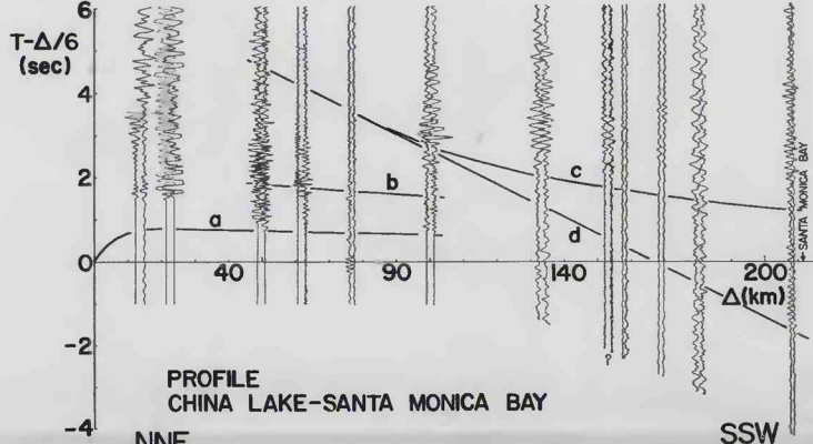
FIGURE 53.—Record section of the profile from China Lake (8) to Santa Monica Bay (4). Data in table 85.
