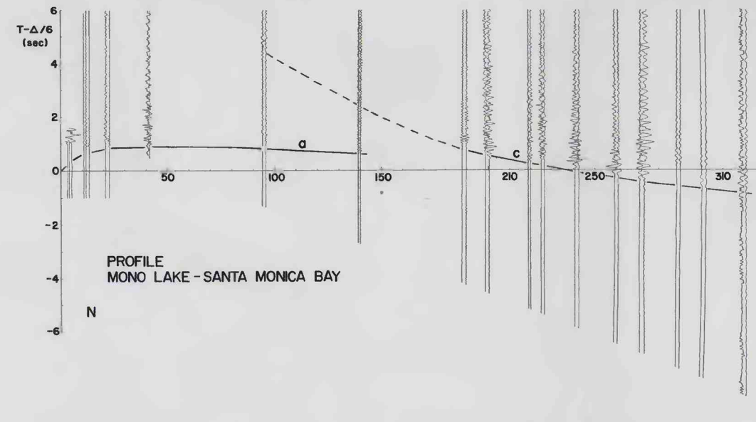
FIGURE 54.—Record section of the profile from Mono Lake (6) to Santa Monica Bay (4). Data in table 86.
