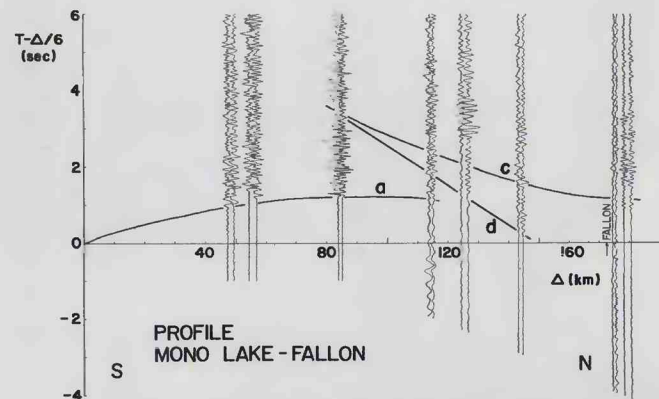
FIGURE 57.—Record section of the profile from Mono Lake (6) to Fallon (9). Data in table 89.
