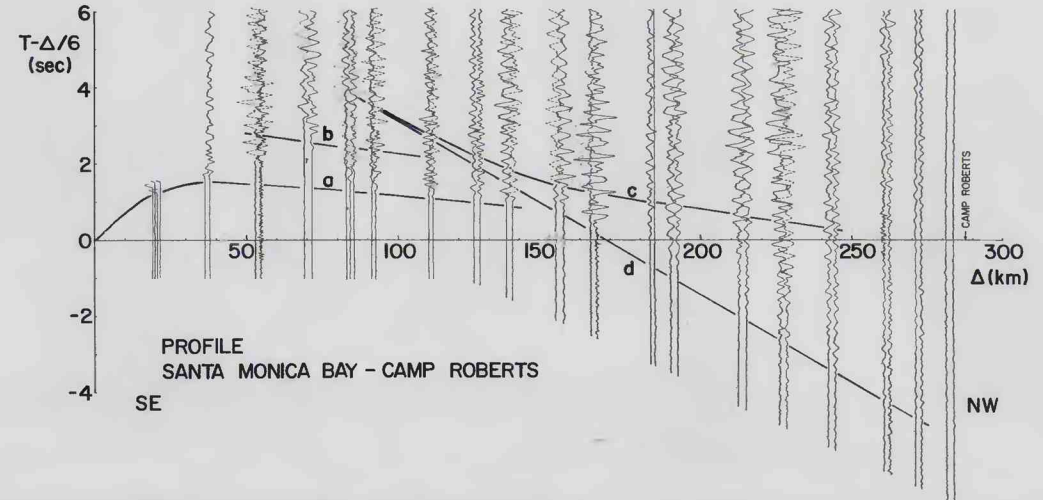
FIGURE 67.—Record section of the profile from Santa Monica Bay (4) to Camp Roberts (2). Data in table 96.
