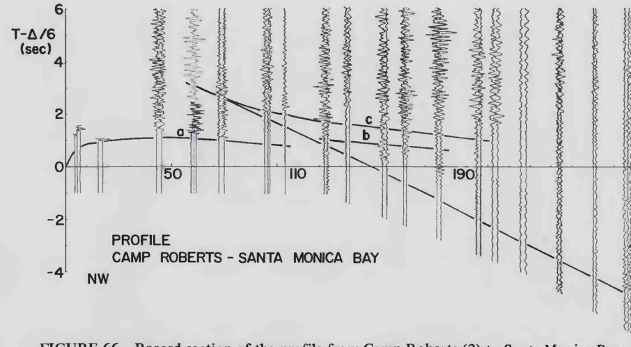
FIGURE 66.—Record section of the profile from Camp Roberts (2) to Santa Monica Bay (4). Data in table 95.
