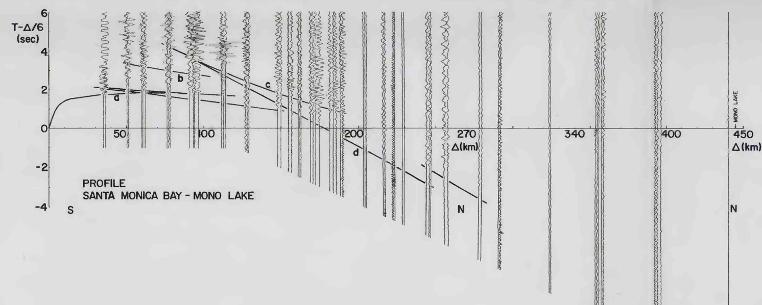
FIGURE 69.—Record section of the profile from Santa Monica Bay (4) to Mono Lake (6). Data in table 97.
