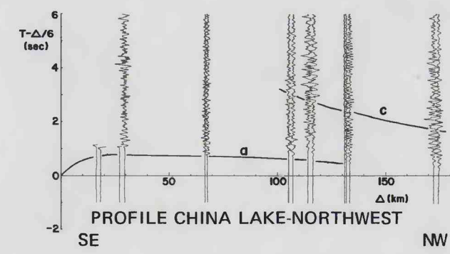
FIGURE 51.—Record section of the profile from China Lake (8) to Santa Monica Bay (4). Data in table 83.
