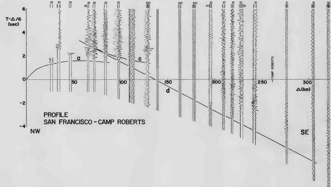
FIGURE 64.—Record section of the profile from San Francisco (1) to Camp Roberts (2). Data in table 93.
