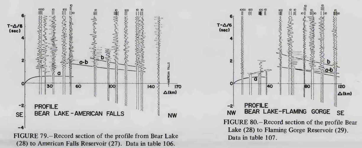
FIGURE 80.—Record section of the profile from Bear Lake (28) to Flaming Gorge (29). Data in table 107.
