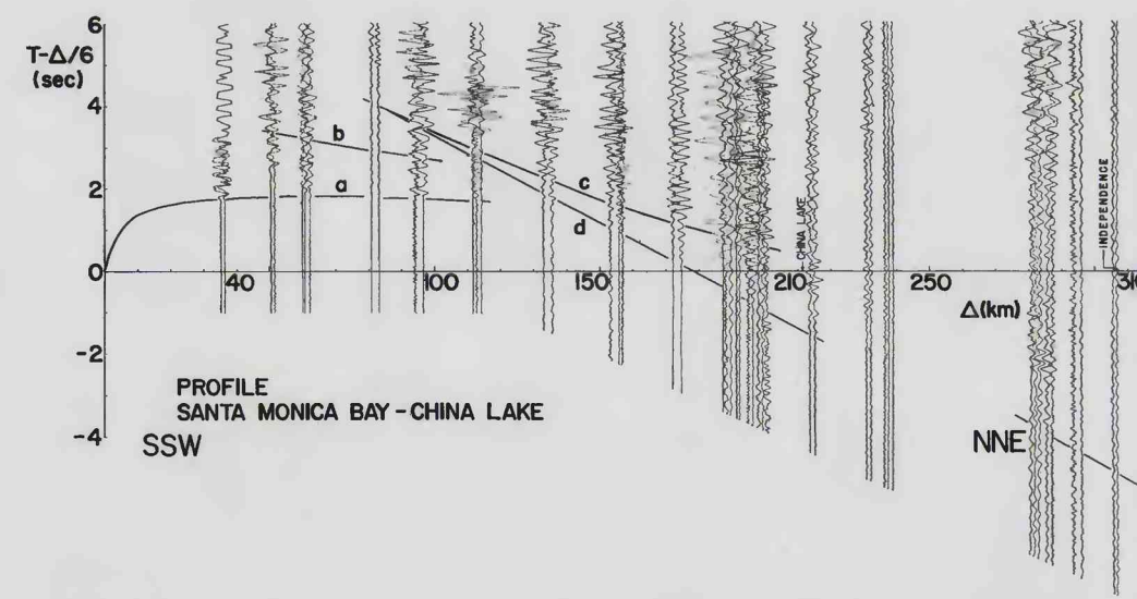
FIGURE 70.—Record section of the profile from Santa Monica Bay (4) to China Lake (8). Data in table 98.
