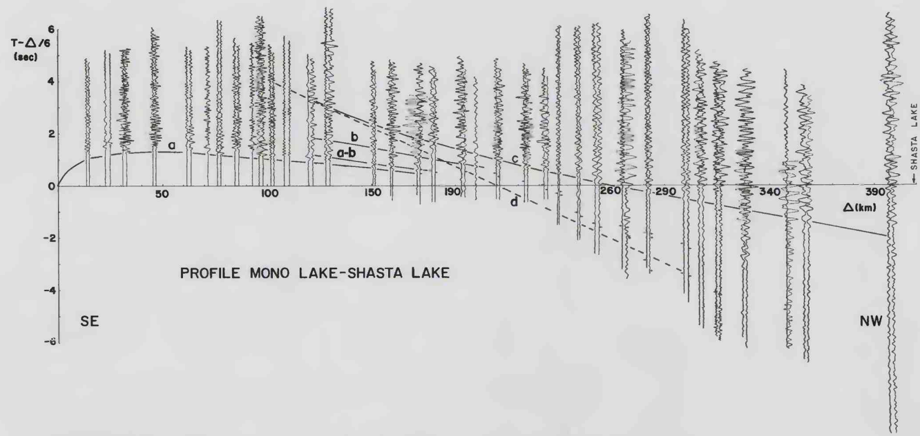
FIGURE 47.—Record section of the profile from Mono Lake (6) to Shasta Lake (5). Data in table 80.
