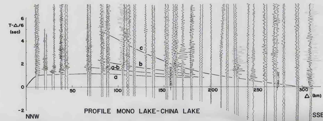
FIGURE 48.—Record section of the profile from Mono Lake (6) to China Lake (8). Data in table 81.
