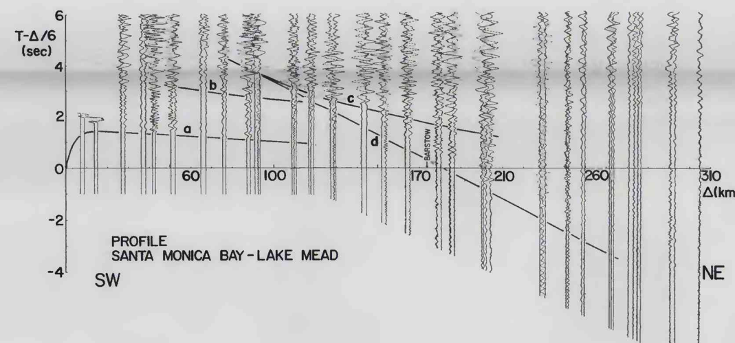
FIGURE 71.—Record section of the profile from Santa Monica Bay (4) to Lake Mead (22). Data in table 99.
