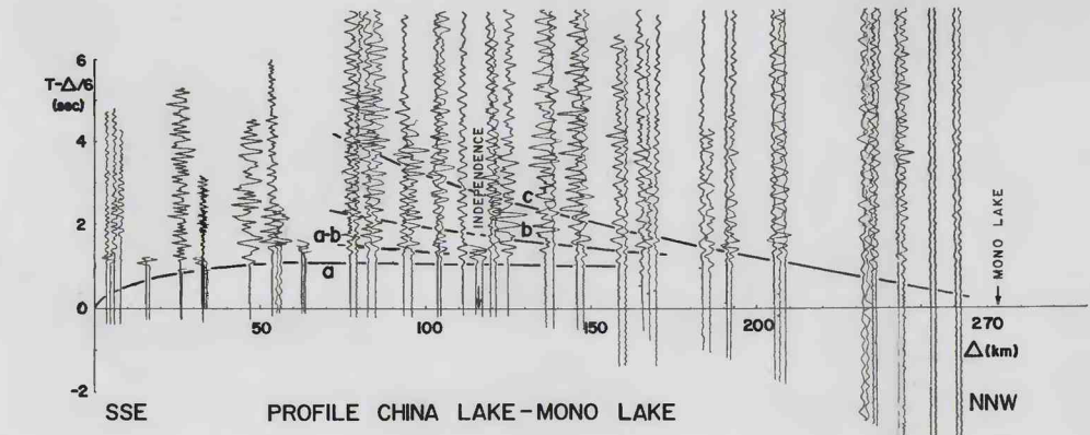
FIGURE 49.—Record section of the profile from China Lake (8) to Mono Lake (6). Data in table 82.
