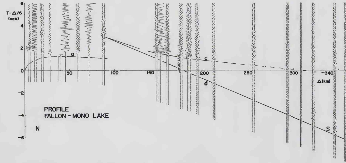
FIGURE 56.—Record section of the profile from Fallon (9) to Mono Lake (6). Data in table 88.
