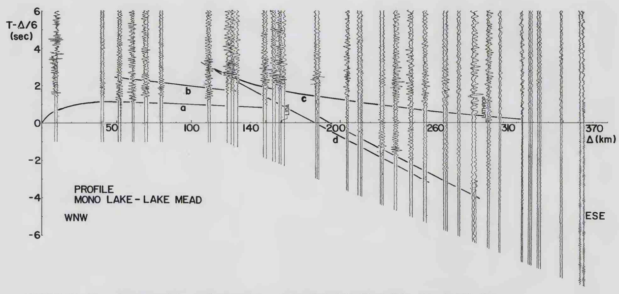
FIGURE 59.—Record section of the profile from Mono Lake (6) to Lake Mead (22). Data in table 91.
