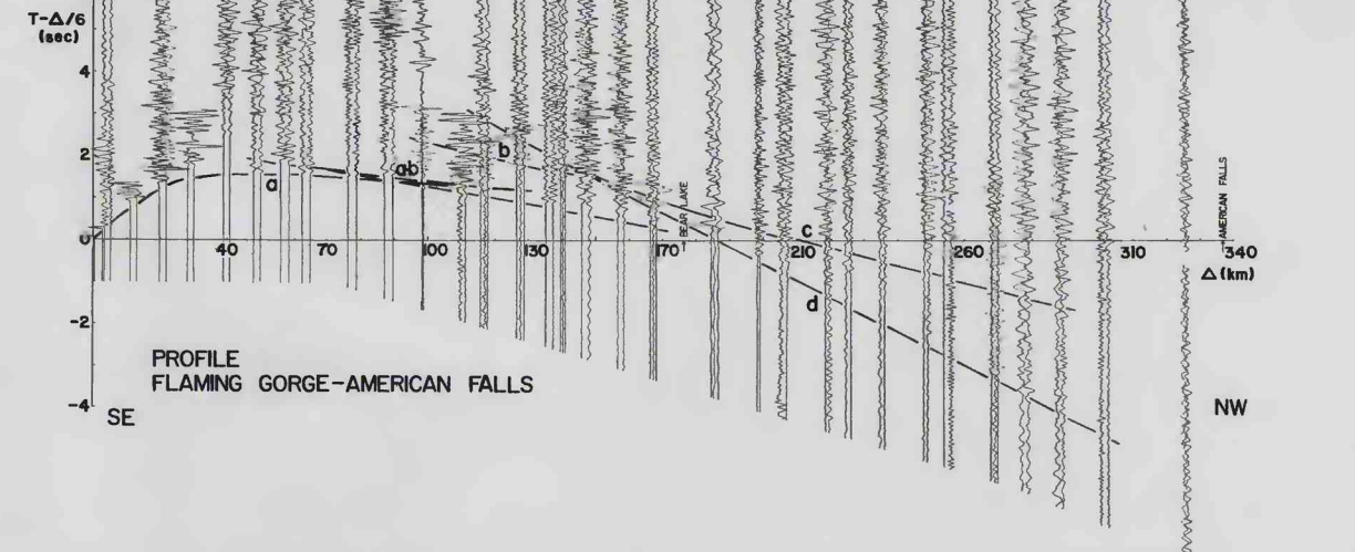
FIGURE 79.—Record section of the profile from Camp Roberts (2) to San Francisco (1). Data in table 94.
