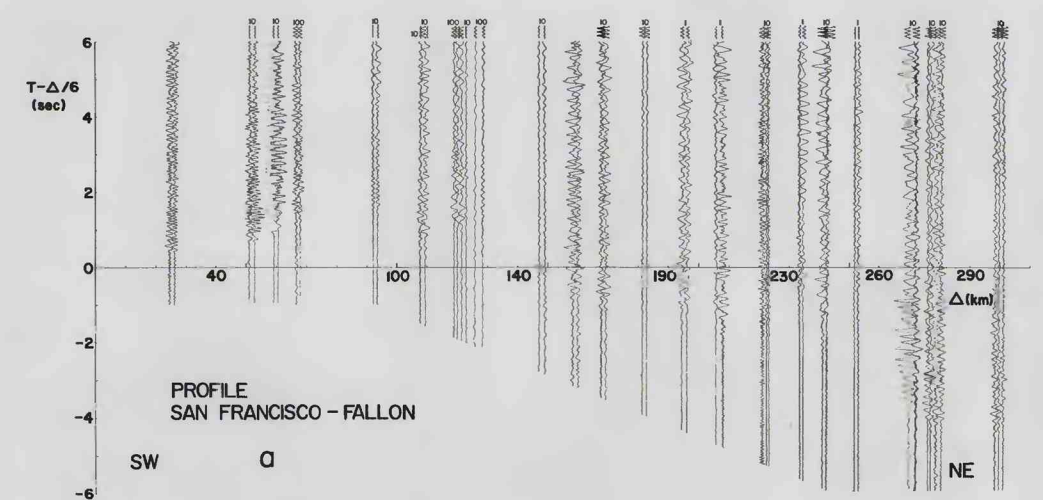
FIGURE 72.—Record section of the profile from San Francisco (1) to Fallon (9). Data in table 100. (a) Not corrected, without interpretation. (b) Corrected: Records of the stations in the Great Valley were shifted along the time axis to eliminate traveltime delays in sedimentary rocks in the valley. Corrections applied are listed in table 106.
