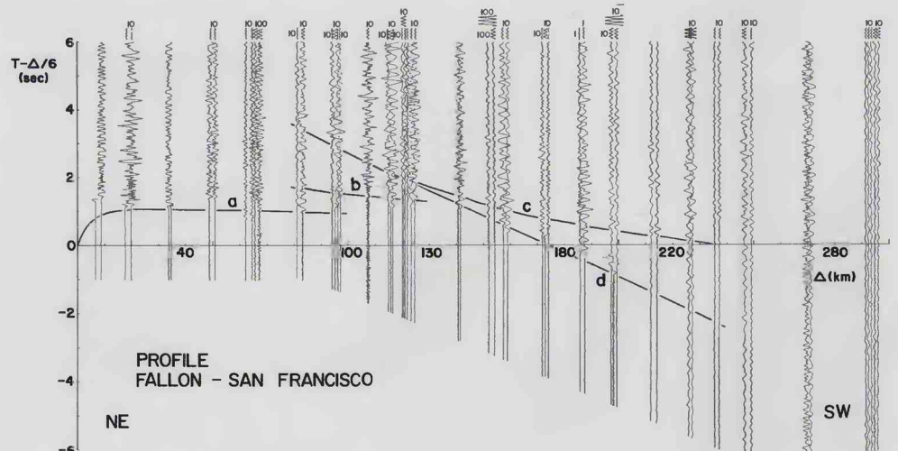
FIGURE 55.—Record section of the profile from Fallon (9) to San Francisco (1). Data in table 87.
