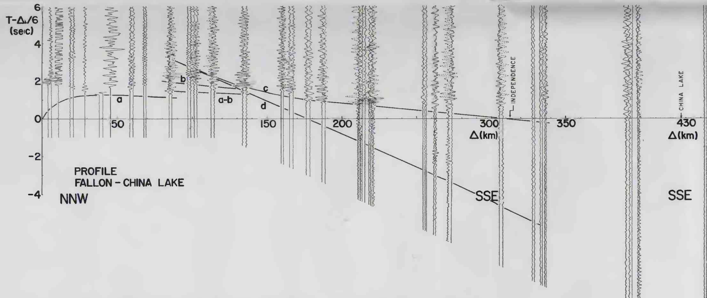
FIGURE 58.—Record section of the profile from Fallon (9) to China Lake (8). Data in table 90.
