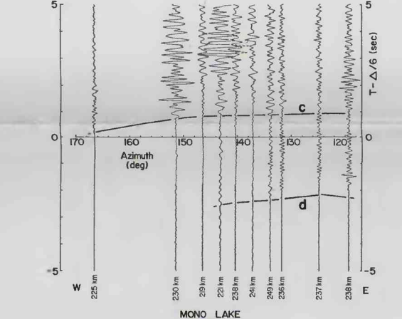
FIGURE 60.—Record section of fan observations from Mono Lake at 230 km distance. Data in table 92.
