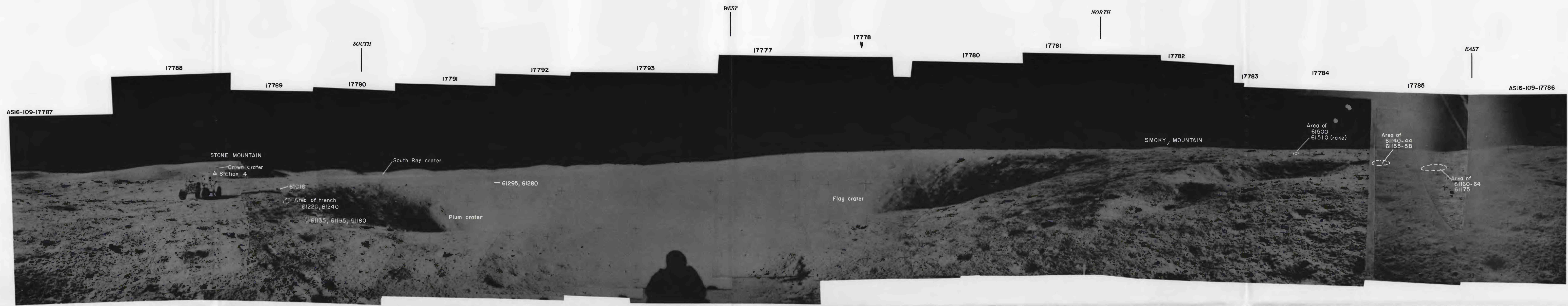
STATION 1 (NE), FLAG CRATER PANORAMA 4
