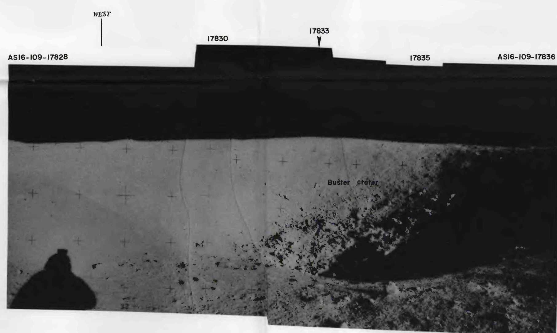
STATION 2, BUSTER CRATER PARTIAL PANORAMA 7
