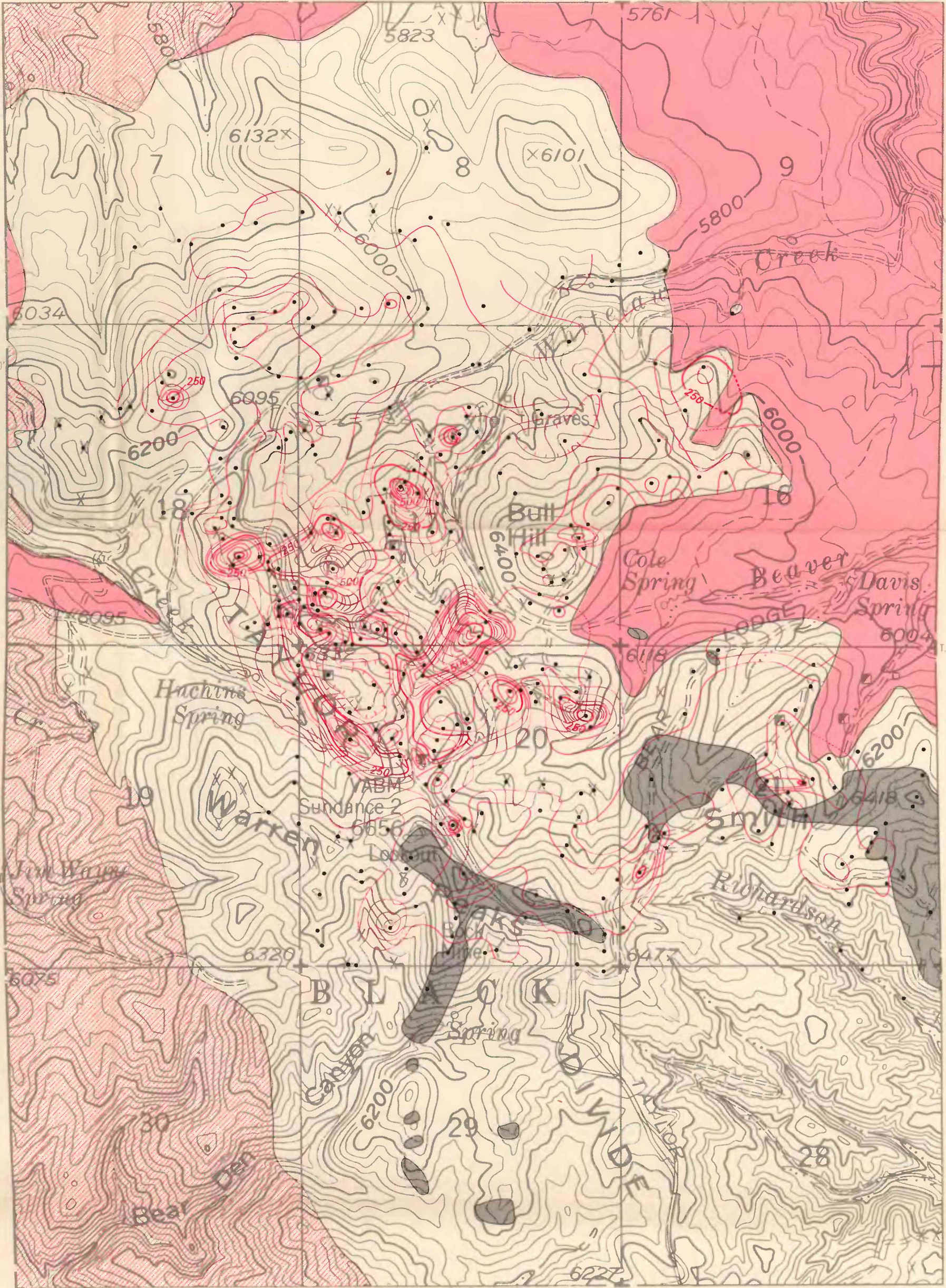
C. THORIUM CONTENT MAP OF AREA UNDERLAIN BY THE DISSEMINATED DEPOSITS
