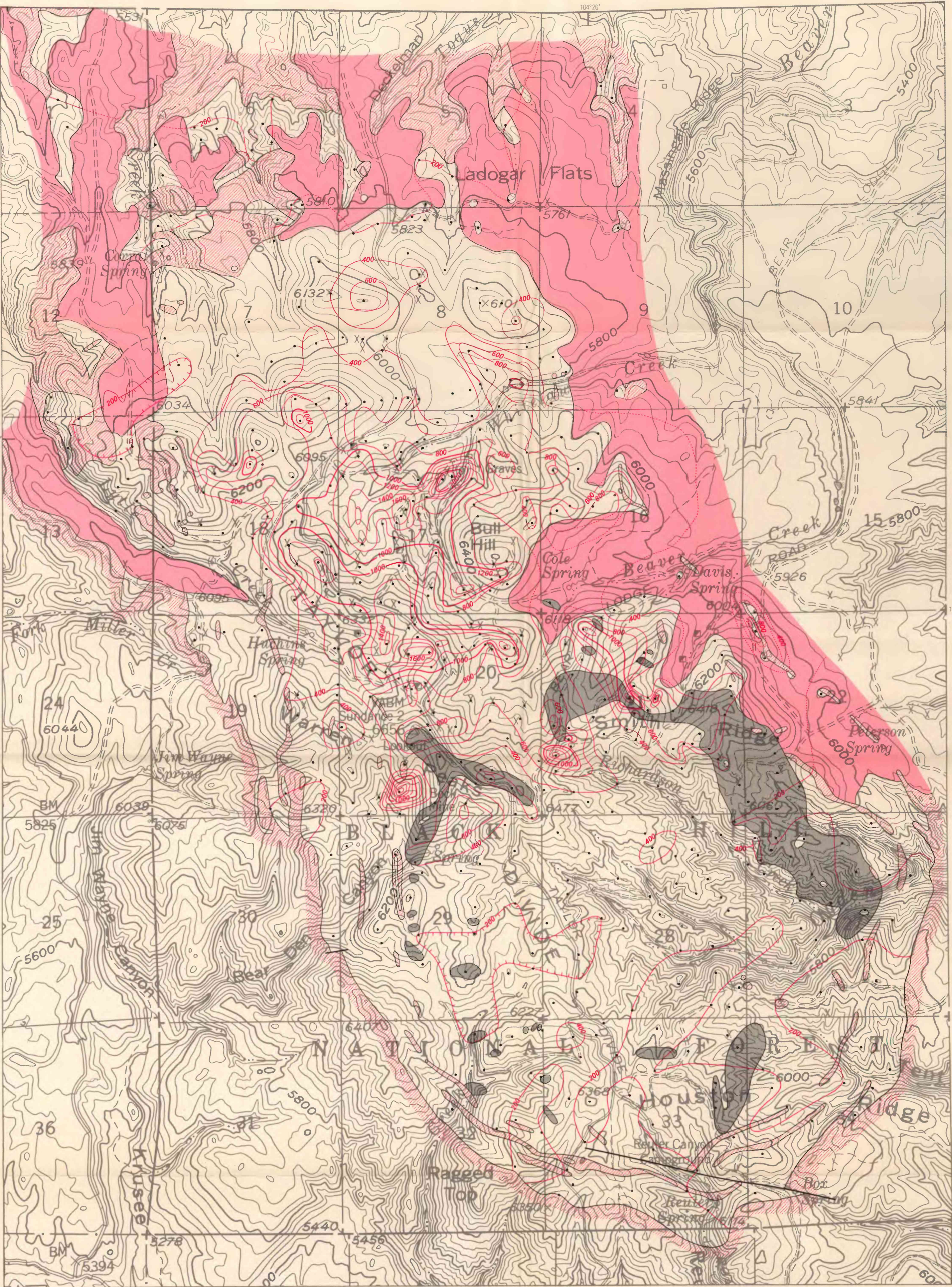
A. RADIOMETRIC MAP OF THE TERTIARY INTRUSIVE CORE OF THE BEAR LODGE DOME
