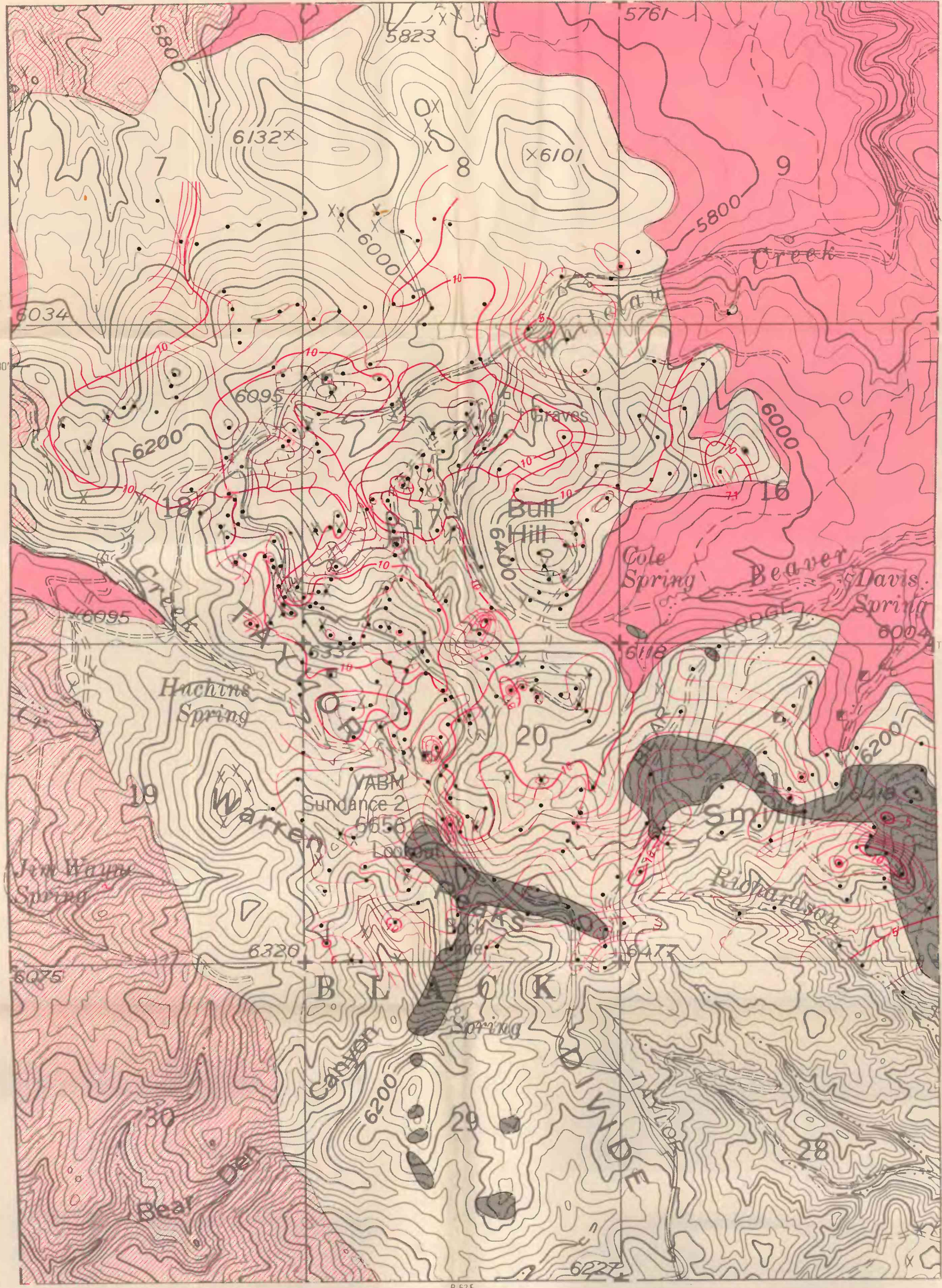
E. POTASSIUM CONTENT MAP OF AREA UNDERLAIN BY THE DISSEMINATED DEPOSITS
