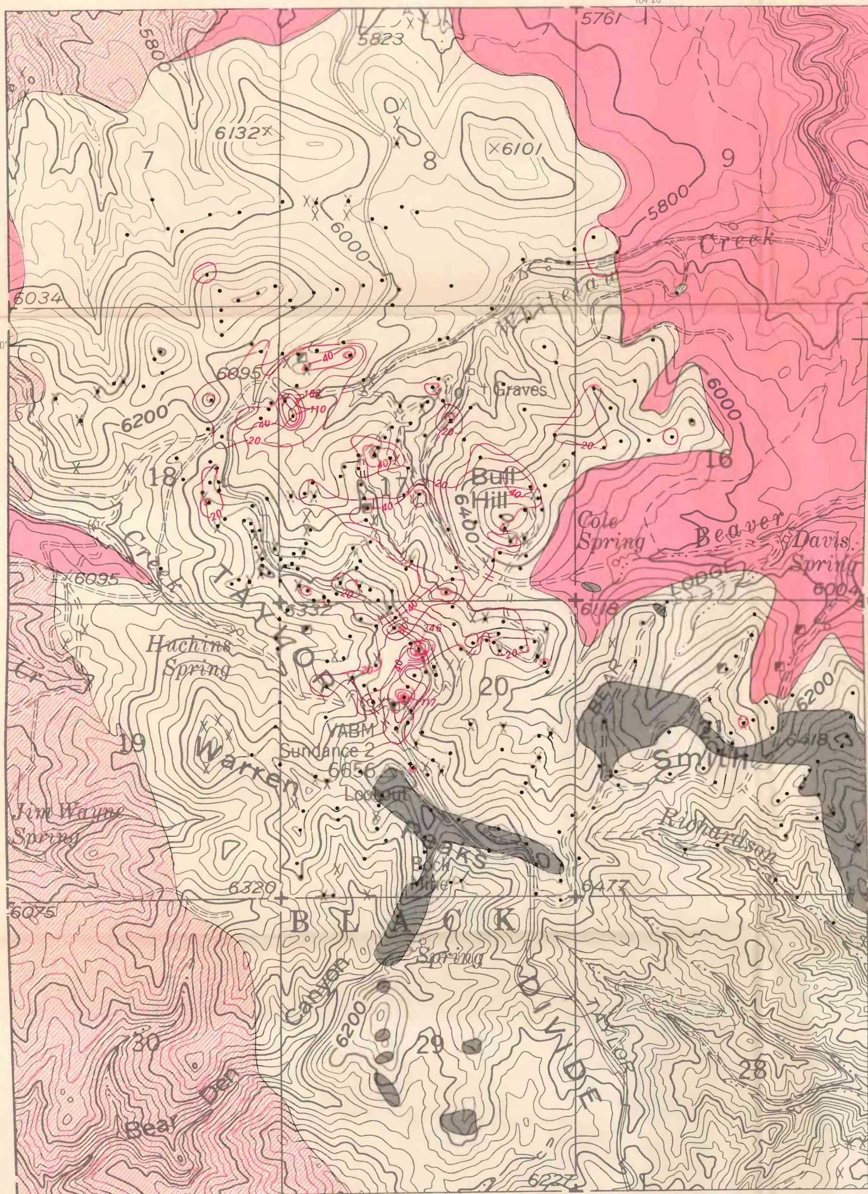
D. URANIUM CONTENT MAP OF AREA UNDERLAIN BY THE DISSEMINATED DEPOSITS
