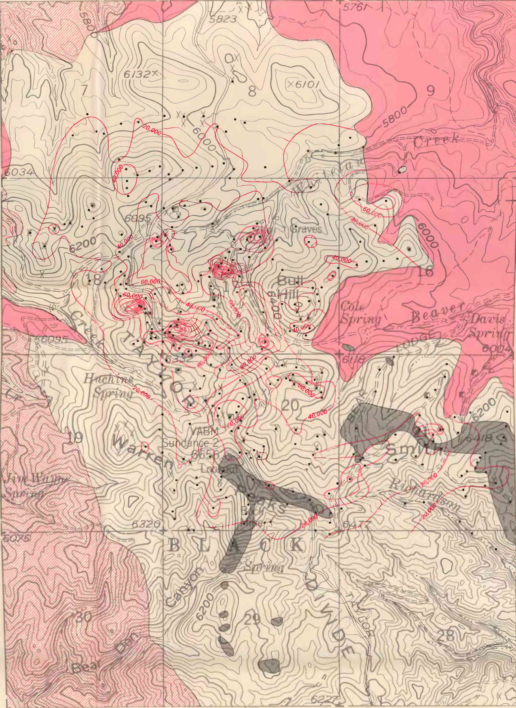
B. DETAILED RADIOMETRIC MAP OF AREA UNDERLAIN BY THE DISSEMINATED DEPOSITS
