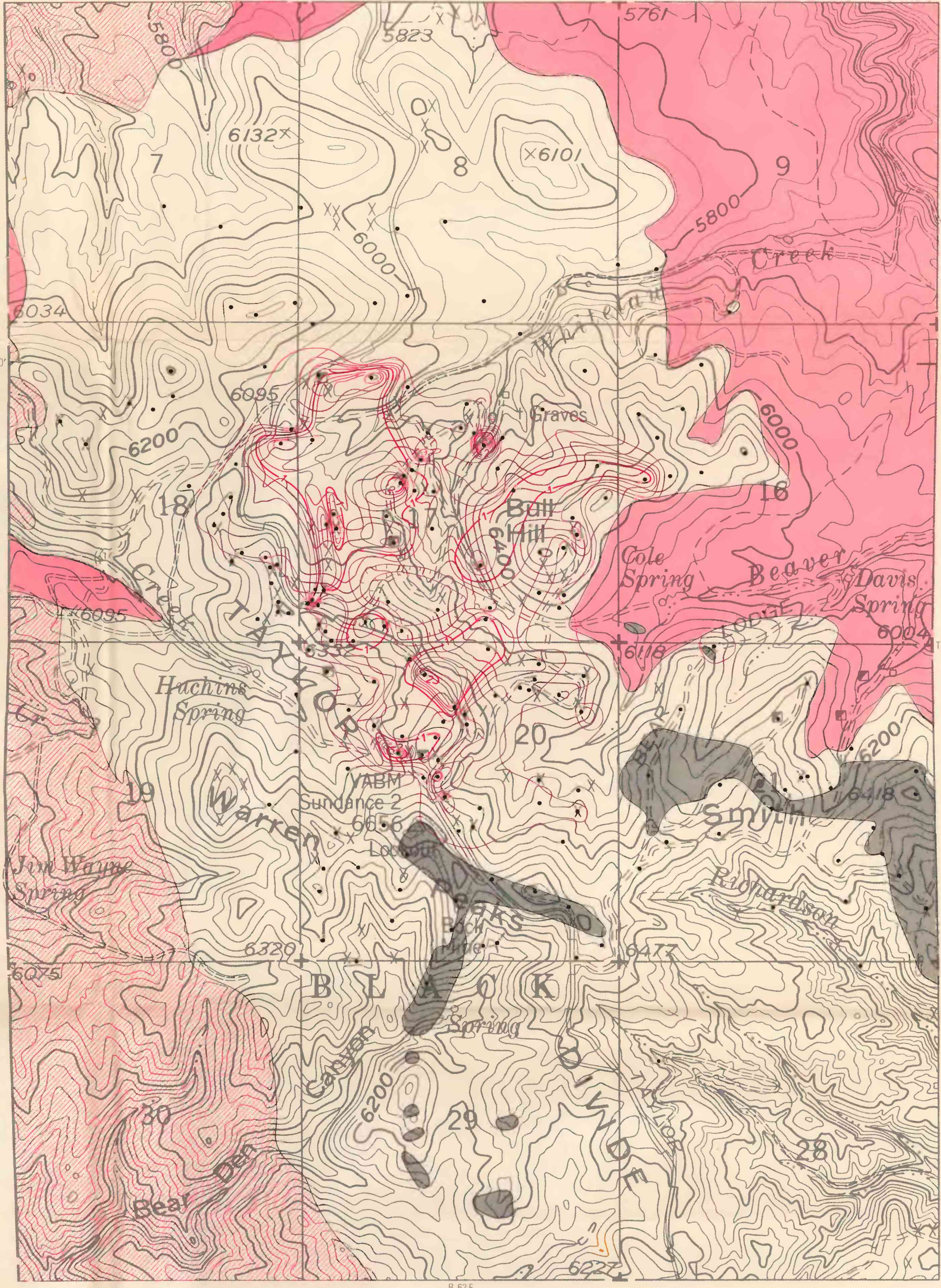
F. TOTAL RARE-EARTH CONTENT MAP OF AREA UNDERLAIN BY THE DISSEMINATED DEPOSITS
