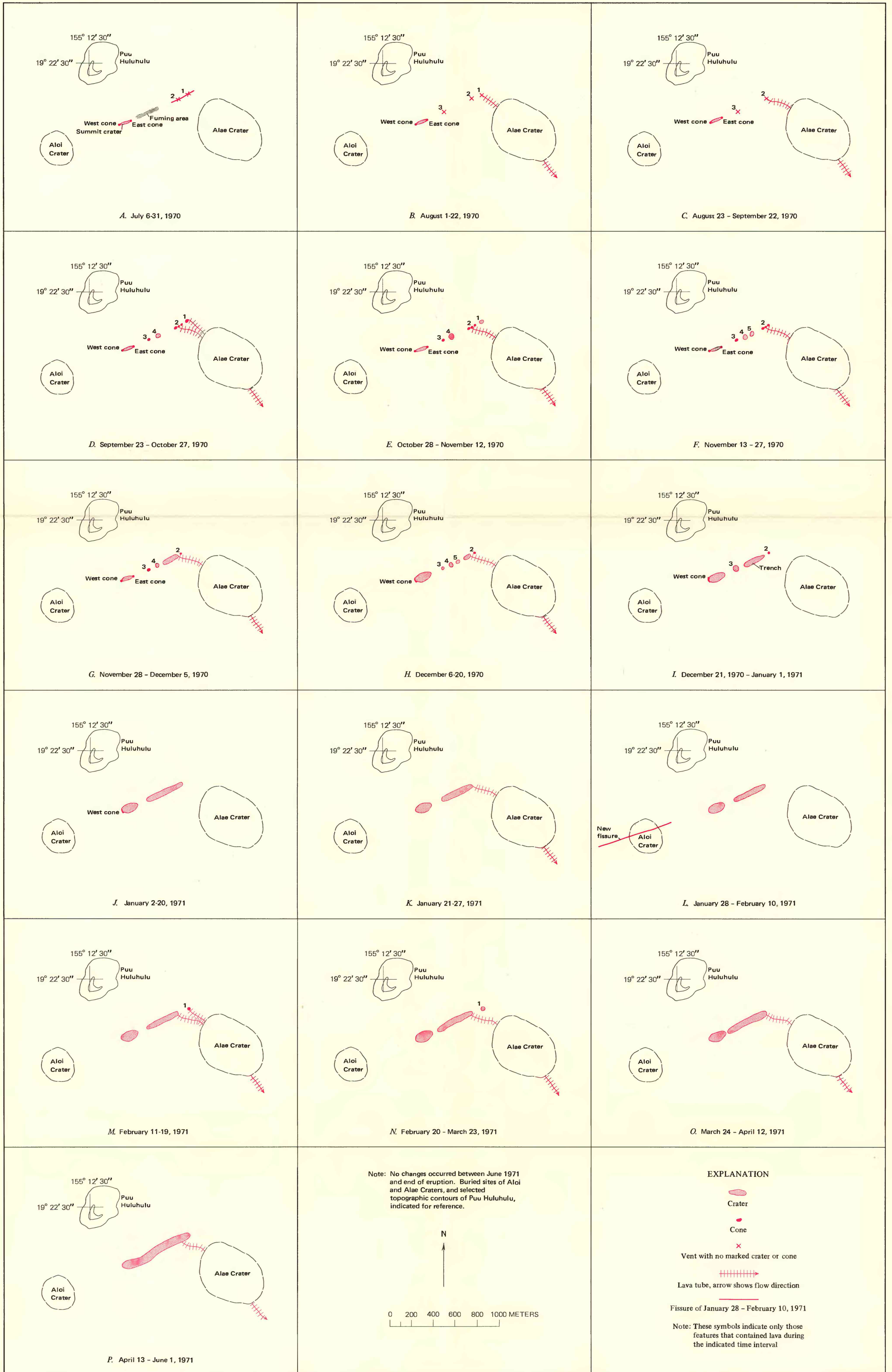
MAPS SHOWING CHANGES IN CONFIGURATION AND LOCATION OF VENTS AT MAUNA ULU, JULY 1970 TO JUNE 1971
