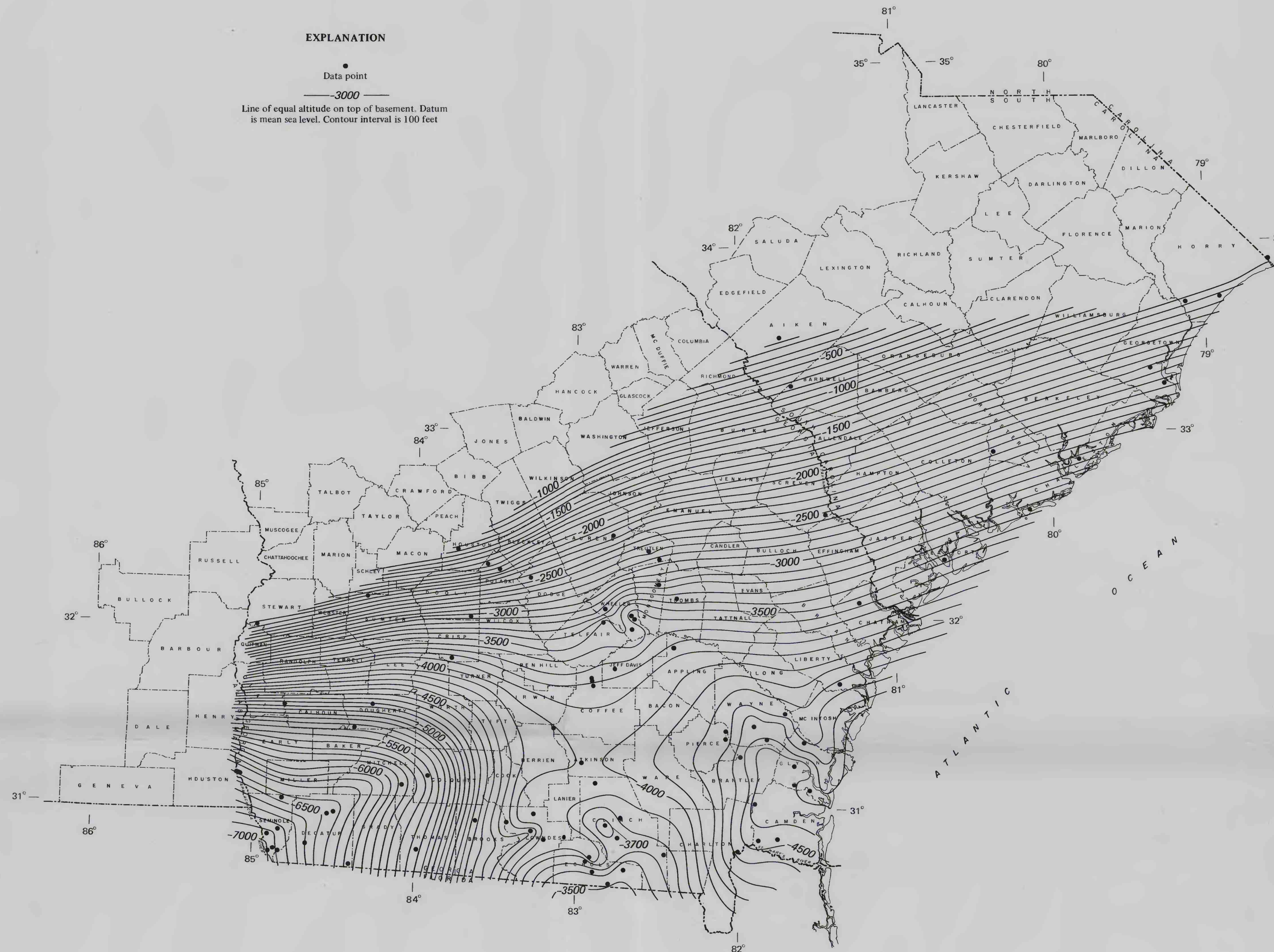
A. STRUCTURAL TOP OF THE PRE-UNIT H(?) BASEMENT SURFACE
