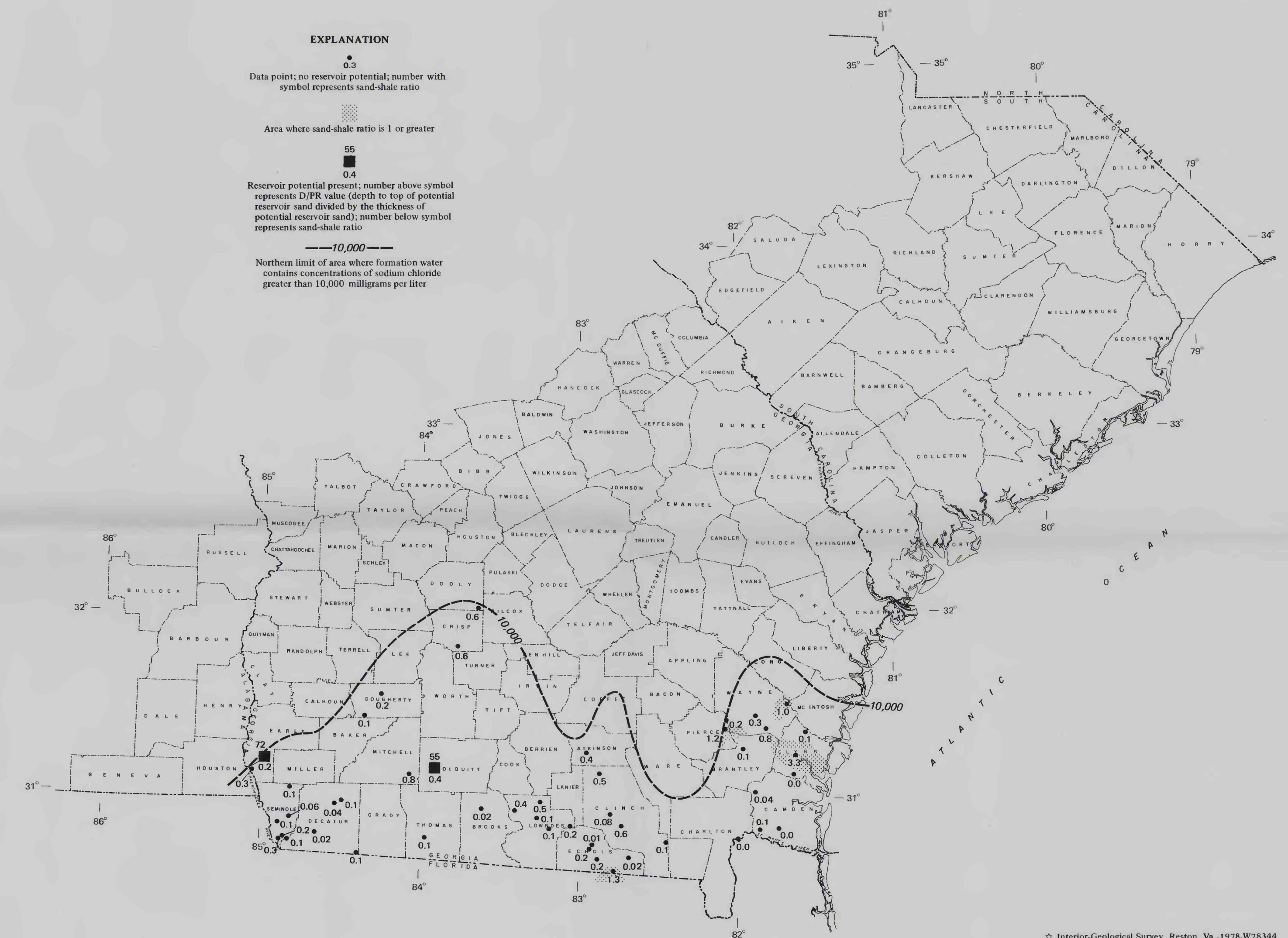
C. SAND-SHALE DISTRIBUTION MAP, UNIT E
