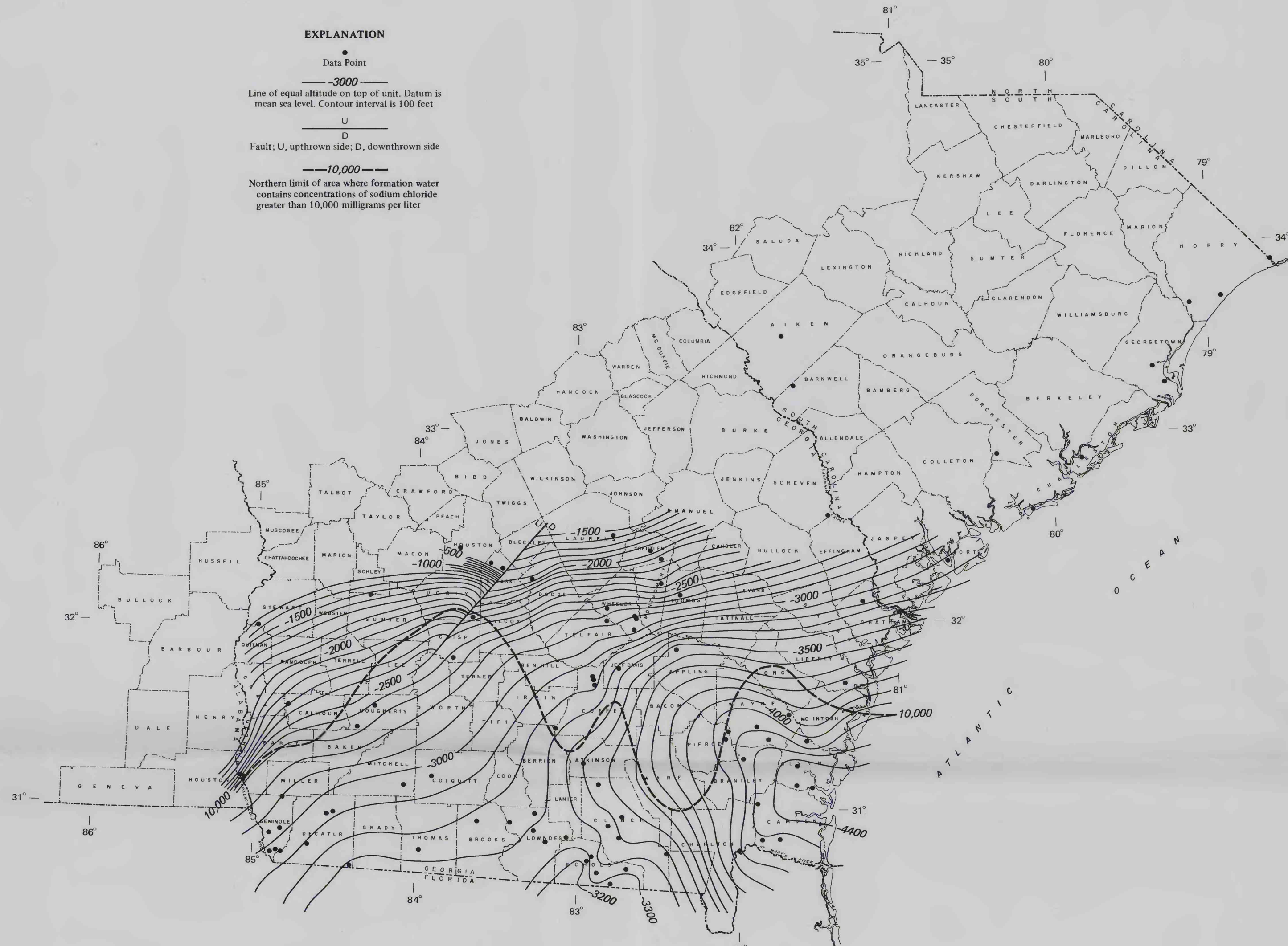
A. STRUCTURAL TOP OF UNIT E
