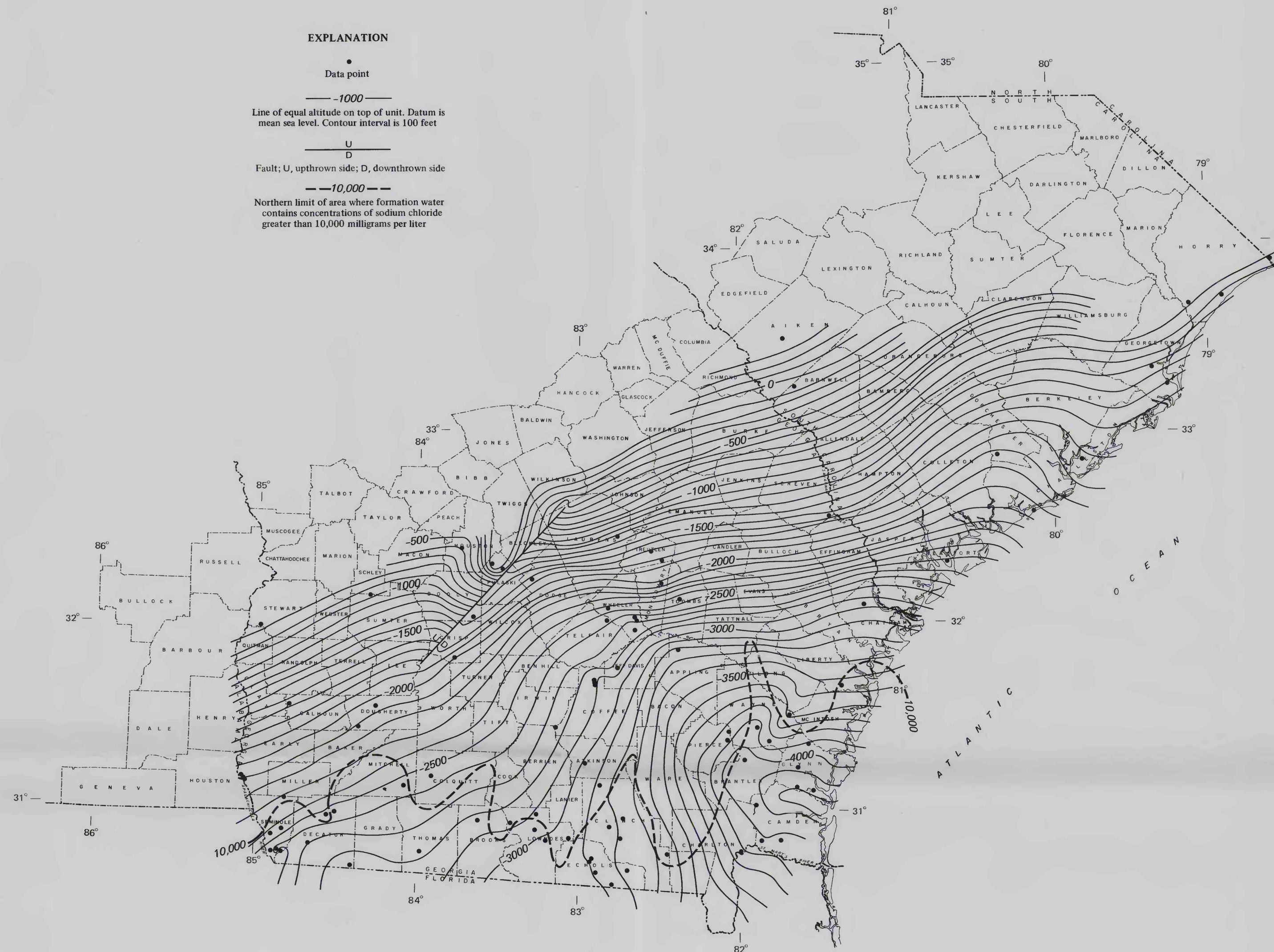
A. STRUCTURAL TOP OF UNIT D
