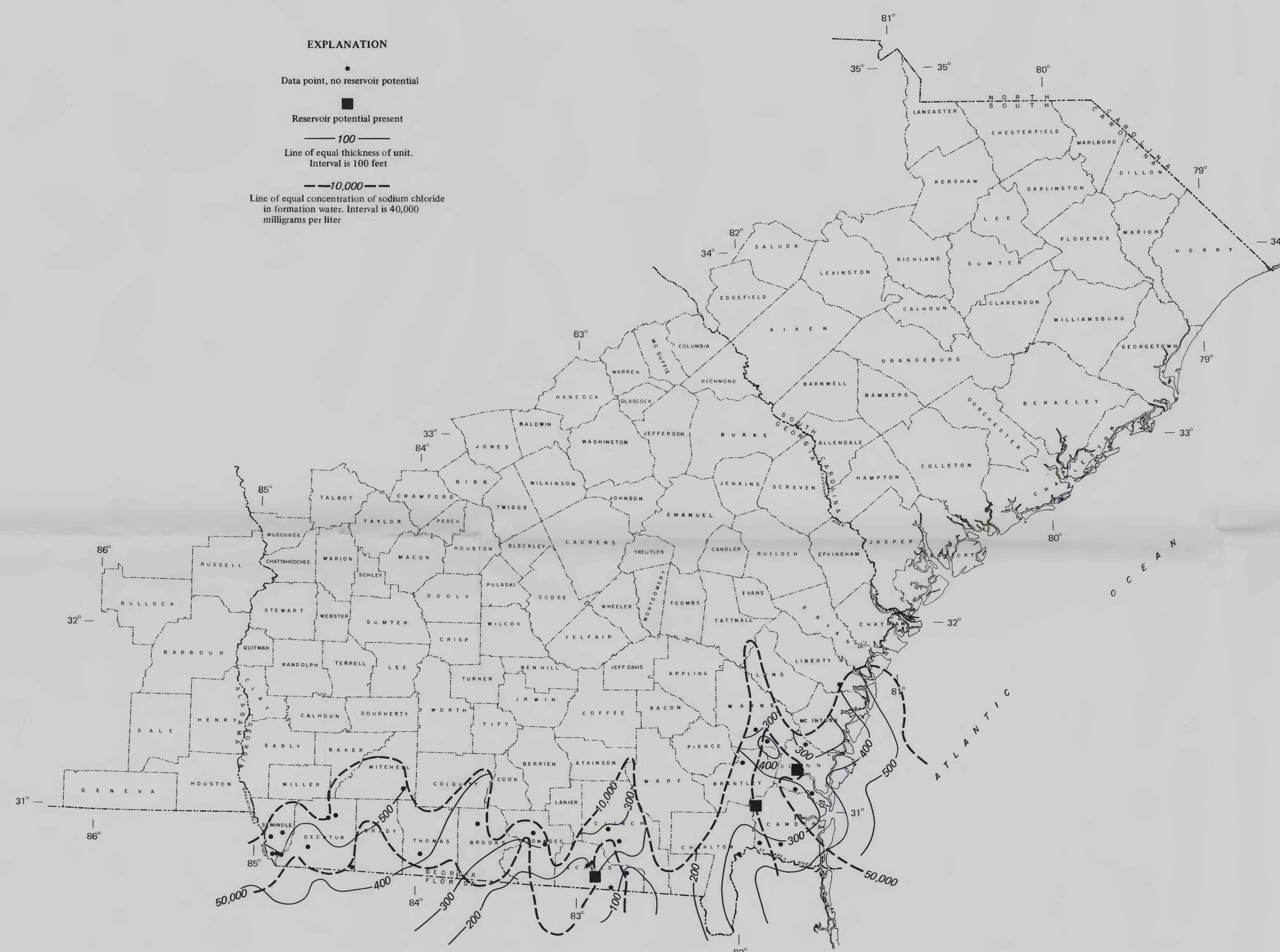
B. THICKNESS AND SODIUM CHLORIDE CONCENTRATION OF UNIT D IN AREA OF NON-USEABLE GROUND WATER
