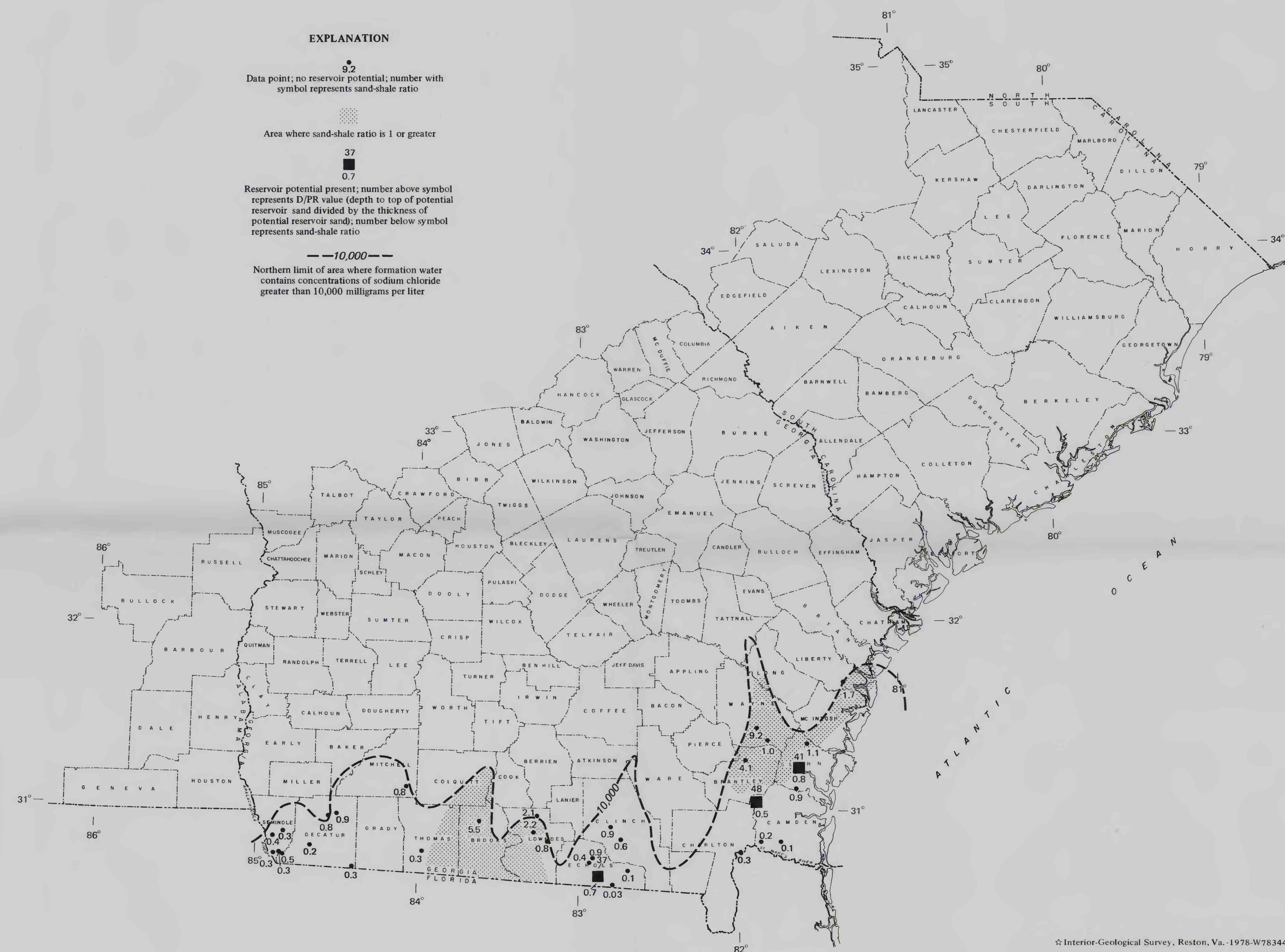
C. SAND-SHALE DISTRIBUTION MAP, UNIT D
