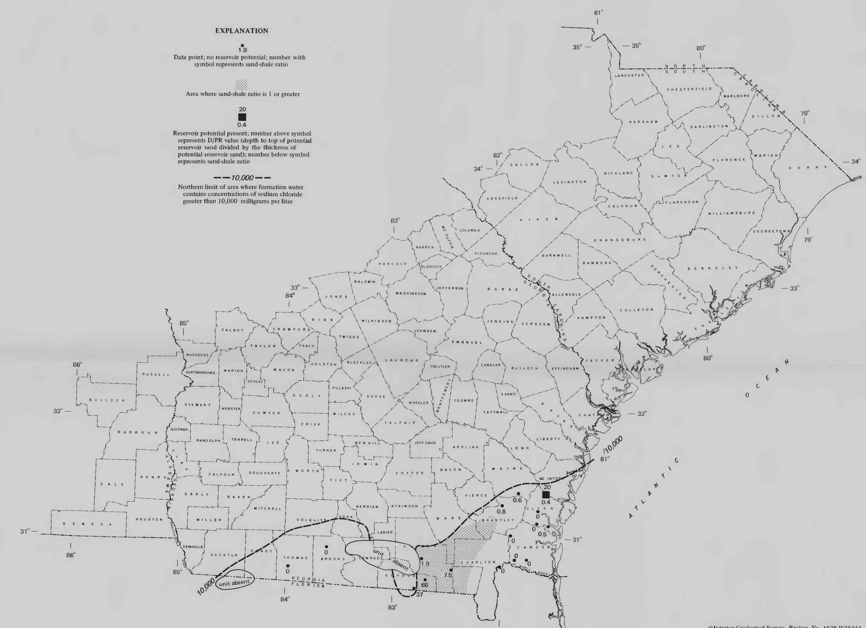
C. SAND-SHALE DISTRIBUTION MAP, UNIT A
