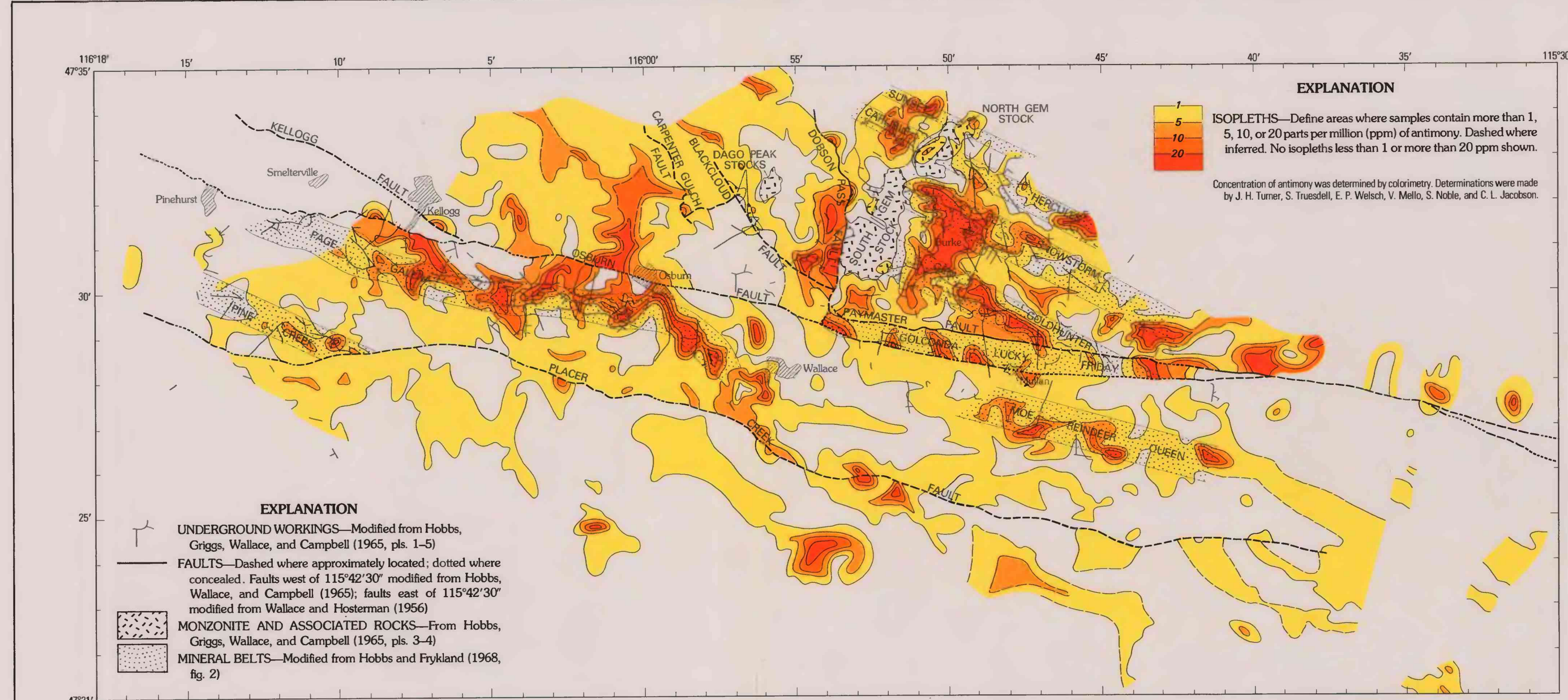
A. DISTRIBUTION OF ANTIMONY IN ROCKS
