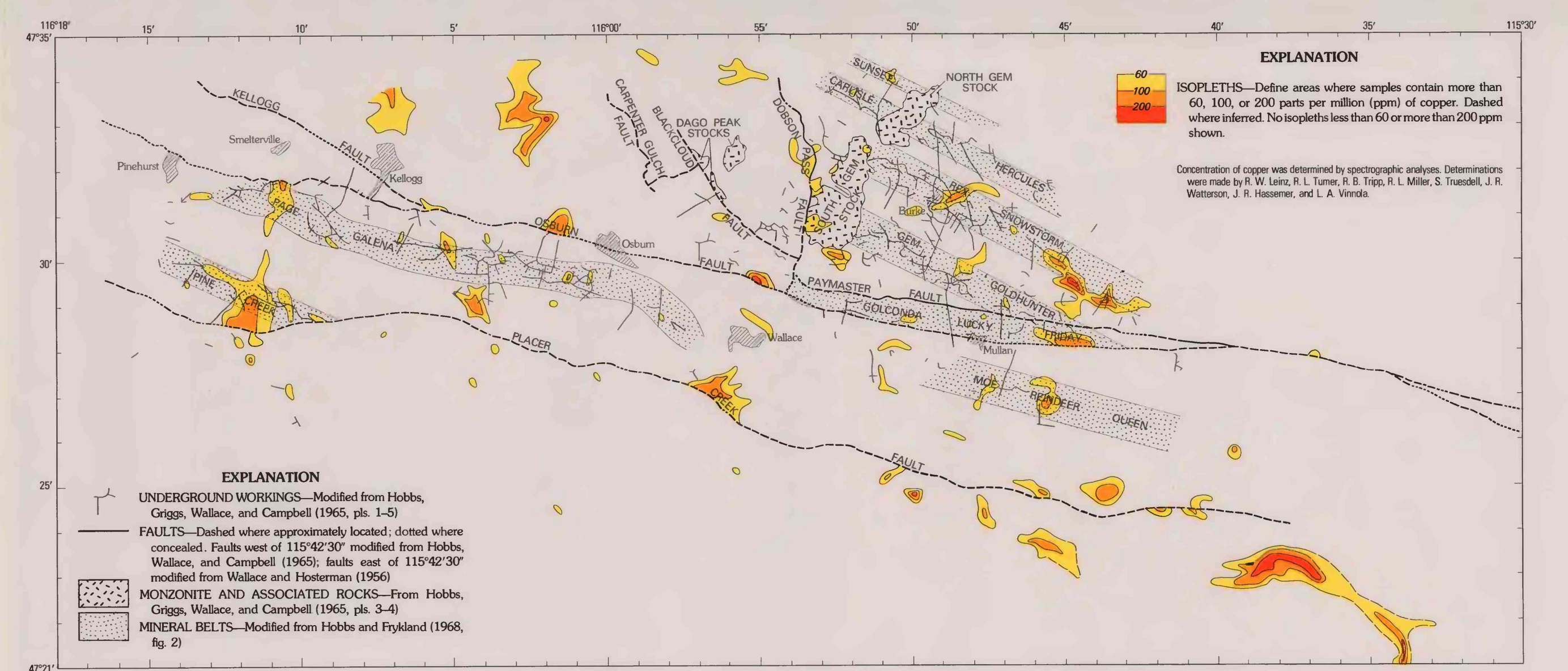
J. DISTRIBUTION OF COPPER IN SOILS
