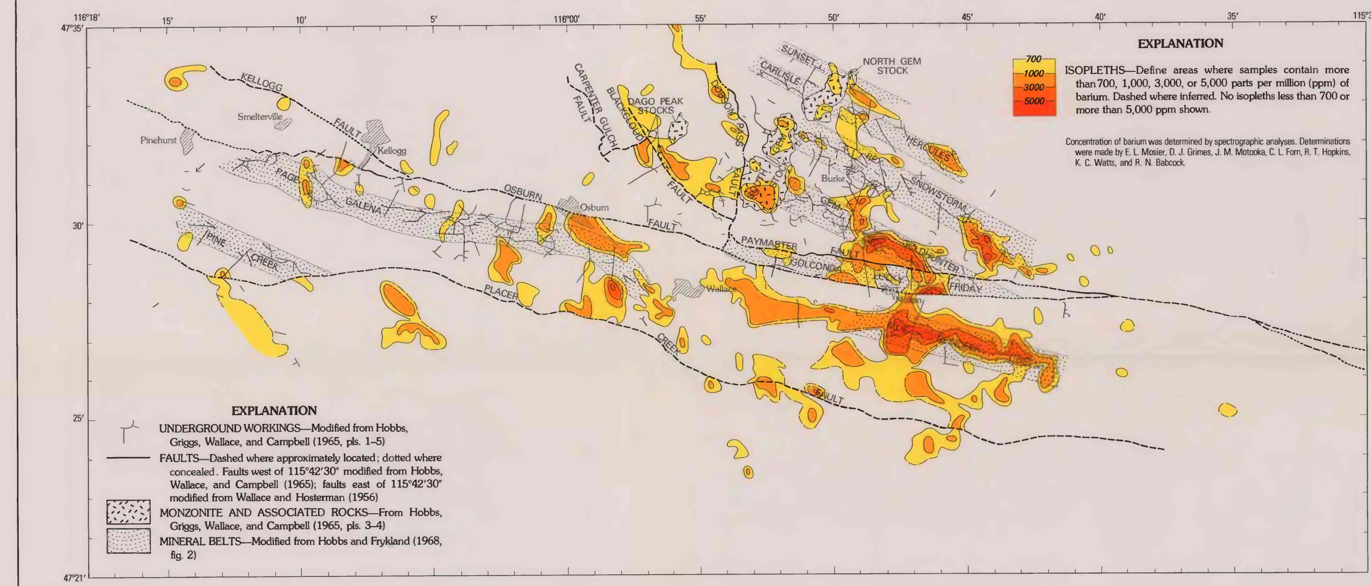
E. DISTRIBUTION OF BARIUM IN ROCKS
