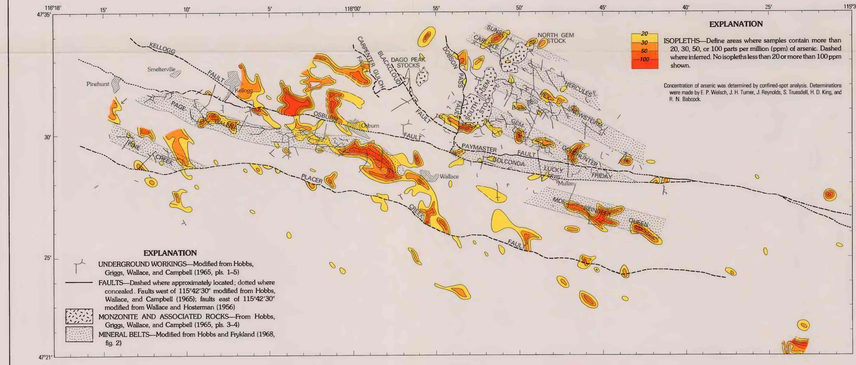
C. DISTRIBUTION OF ARSENIC IN ROCKS
