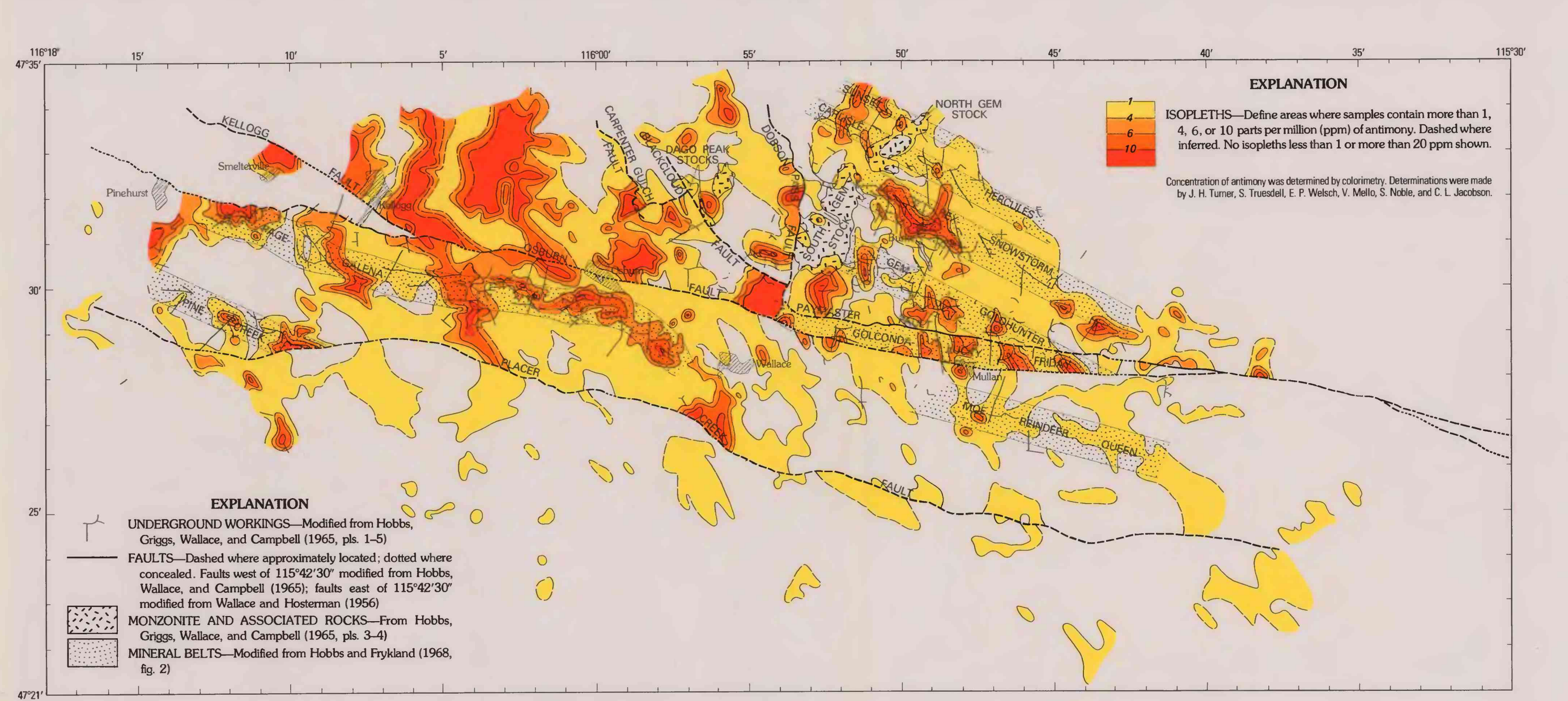
B. DISTRIBUTION OF ANTIMONY IN SOILS
