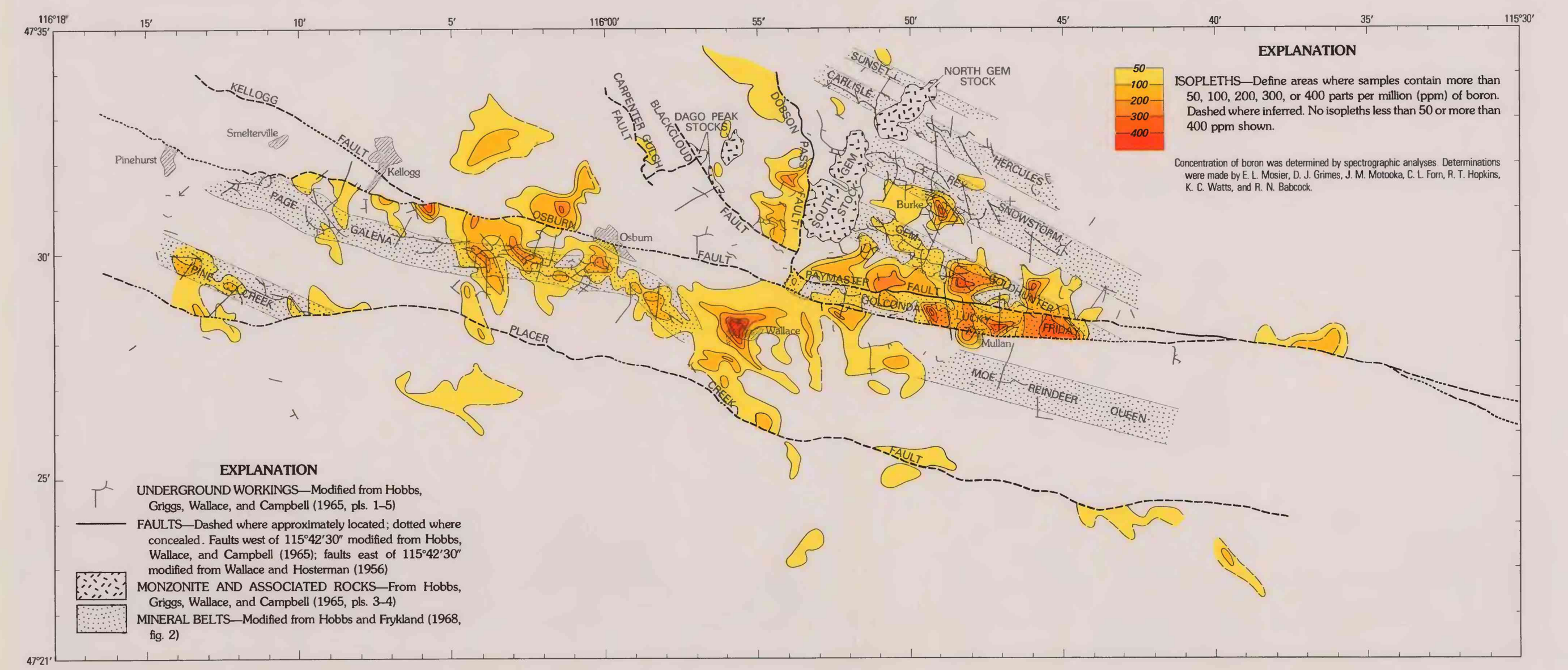
H. DISTRIBUTION OF BORON IN SOILS
