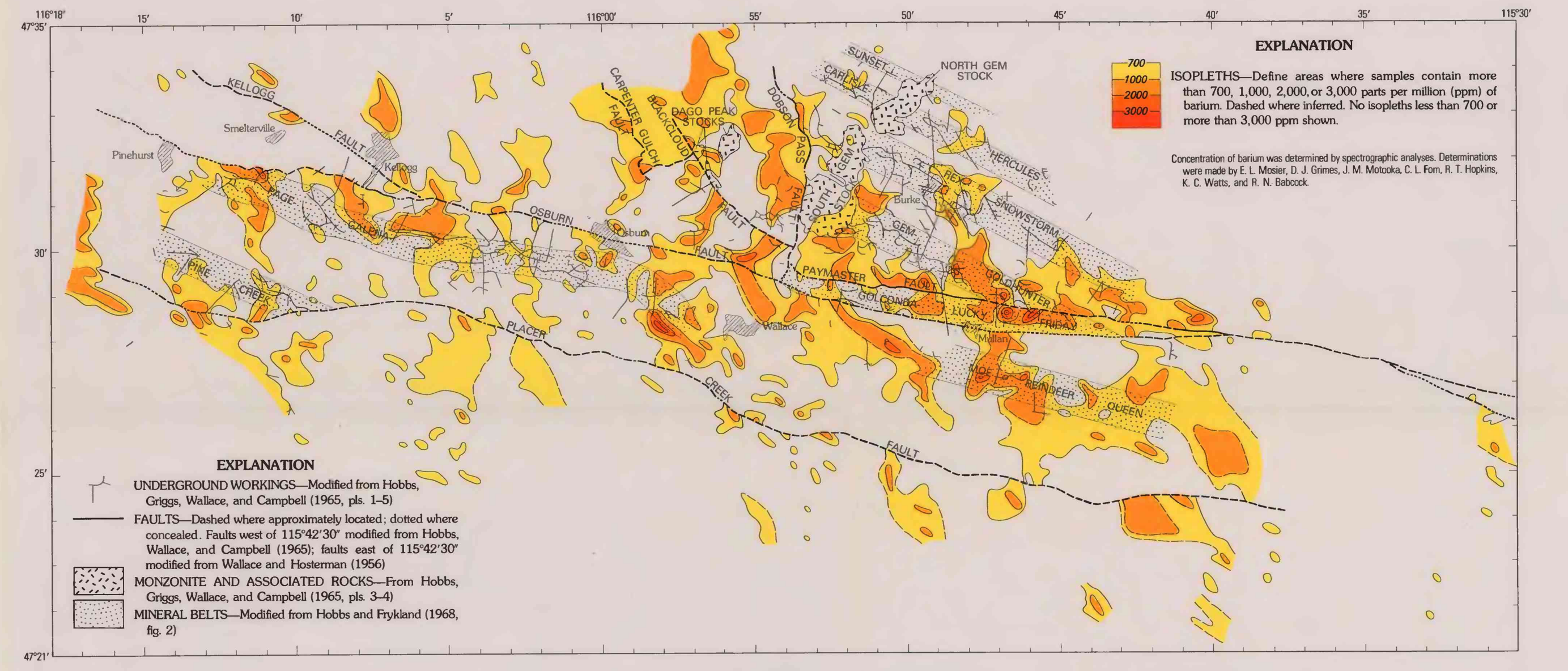
F. DISTRIBUTION OF BARIUM IN SOILS
