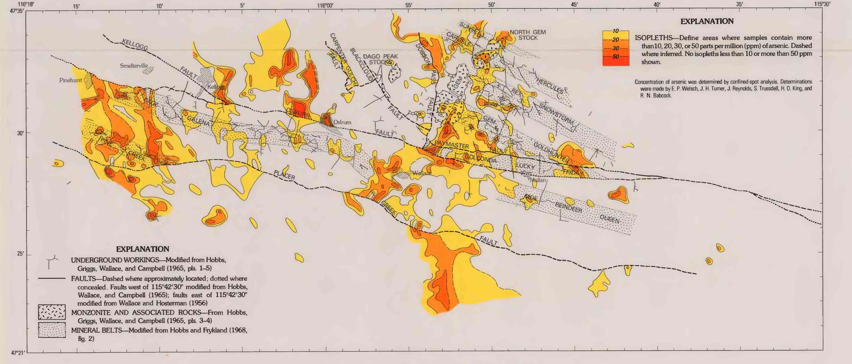
D. DISTRIBUTION OF ARSENIC IN SOILS
