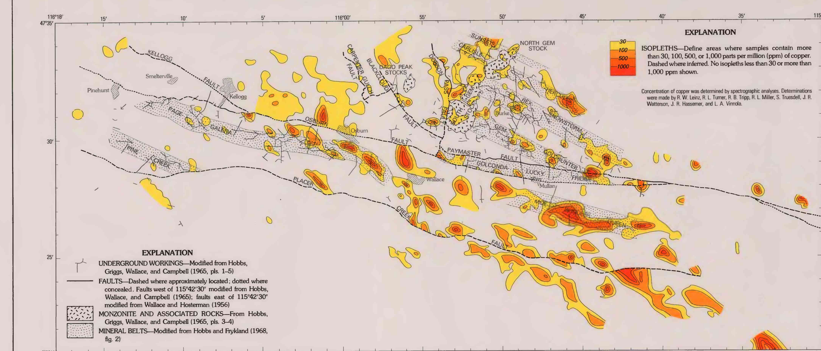
I. DISTRIBUTION OF COPPER IN ROCKS
