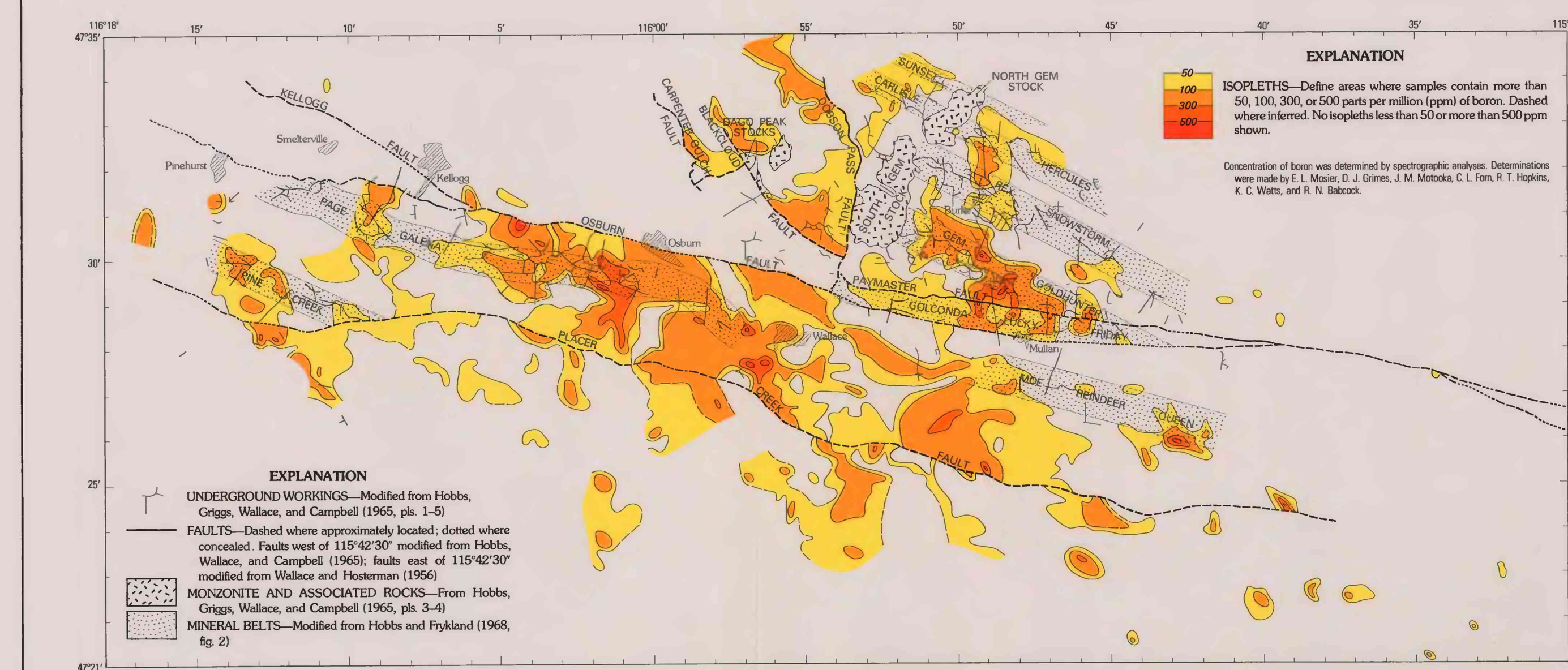
G. DISTRIBUTION OF BORON IN ROCKS
