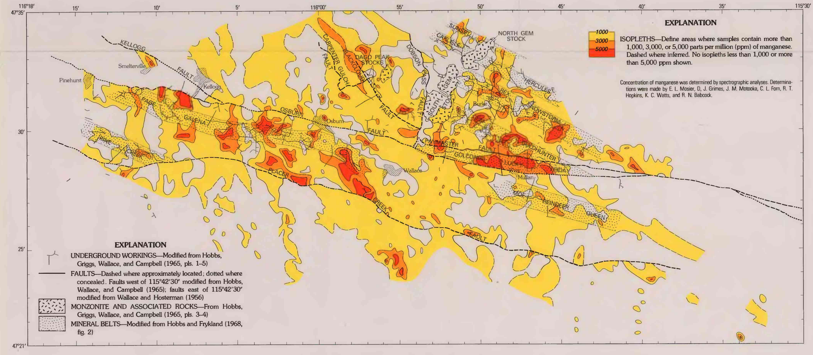
N. DISTRIBUTION OF MANGANESE IN SOILS
