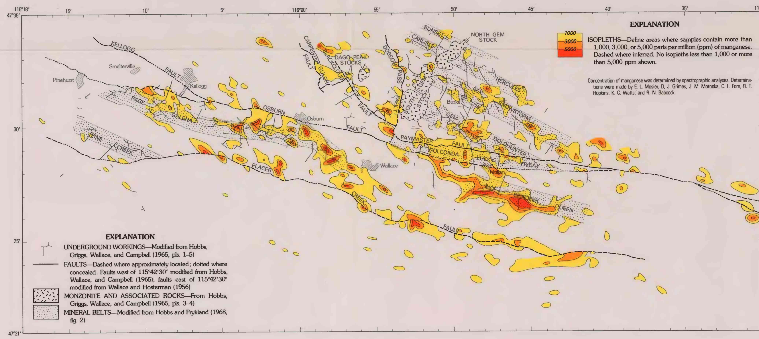
M. DISTRIBUTION OF MANGANESE IN ROCKS
