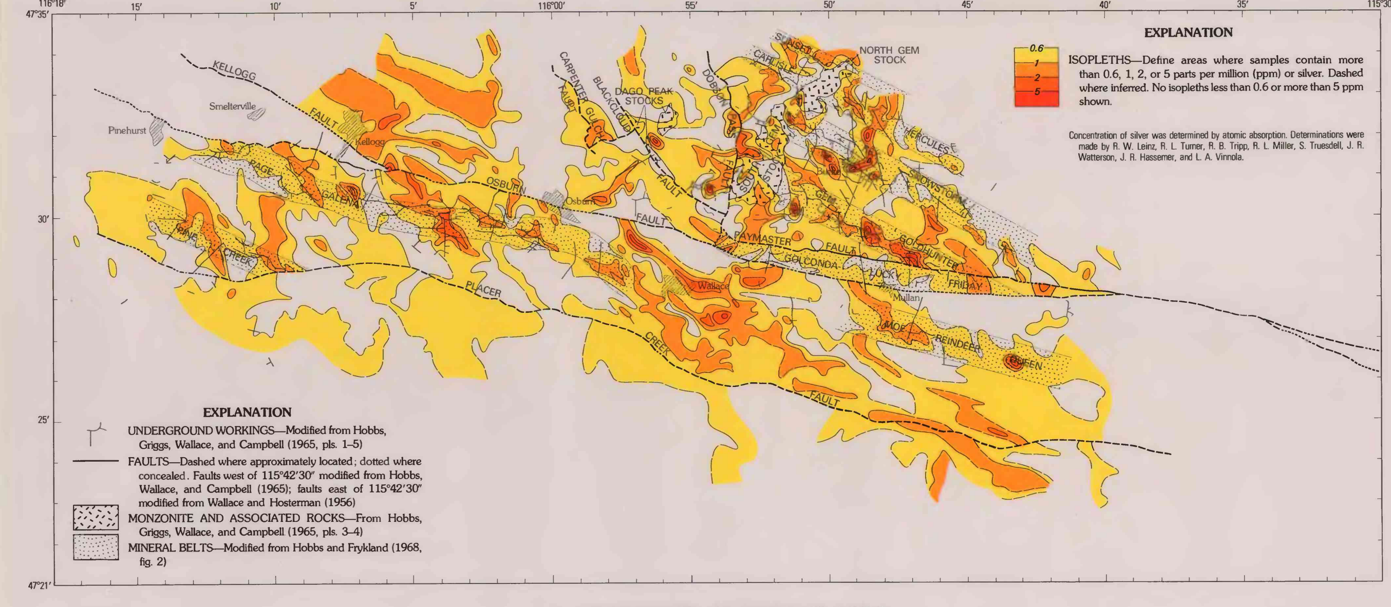
T. DISTRIBUTION OF SILVER IN SOILS
