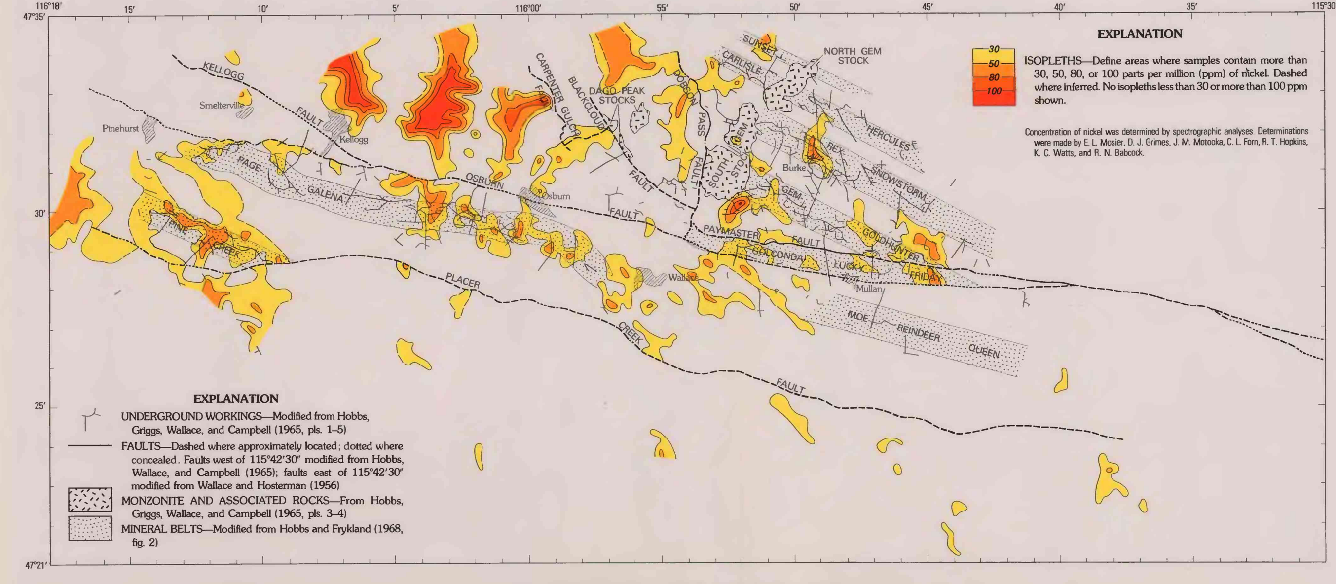
R. DISTRIBUTION OF NICKEL IN SOILS
