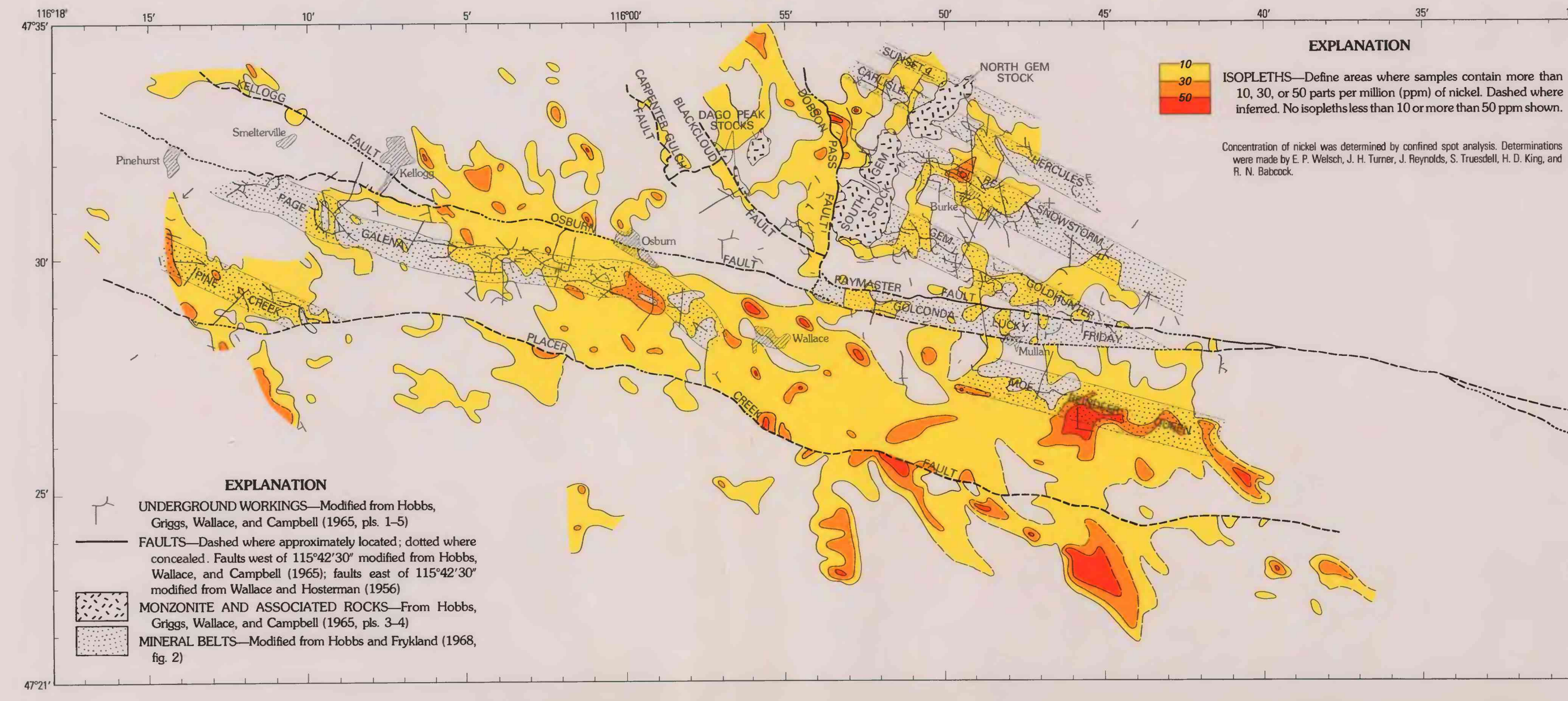
Q. DISTRIBUTION OF NICKEL IN ROCKS
