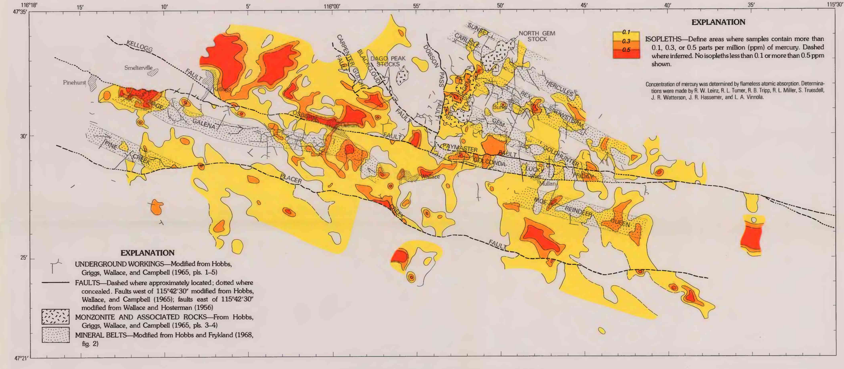
P. DISTRIBUTION OF MERCURY IN SOILS
