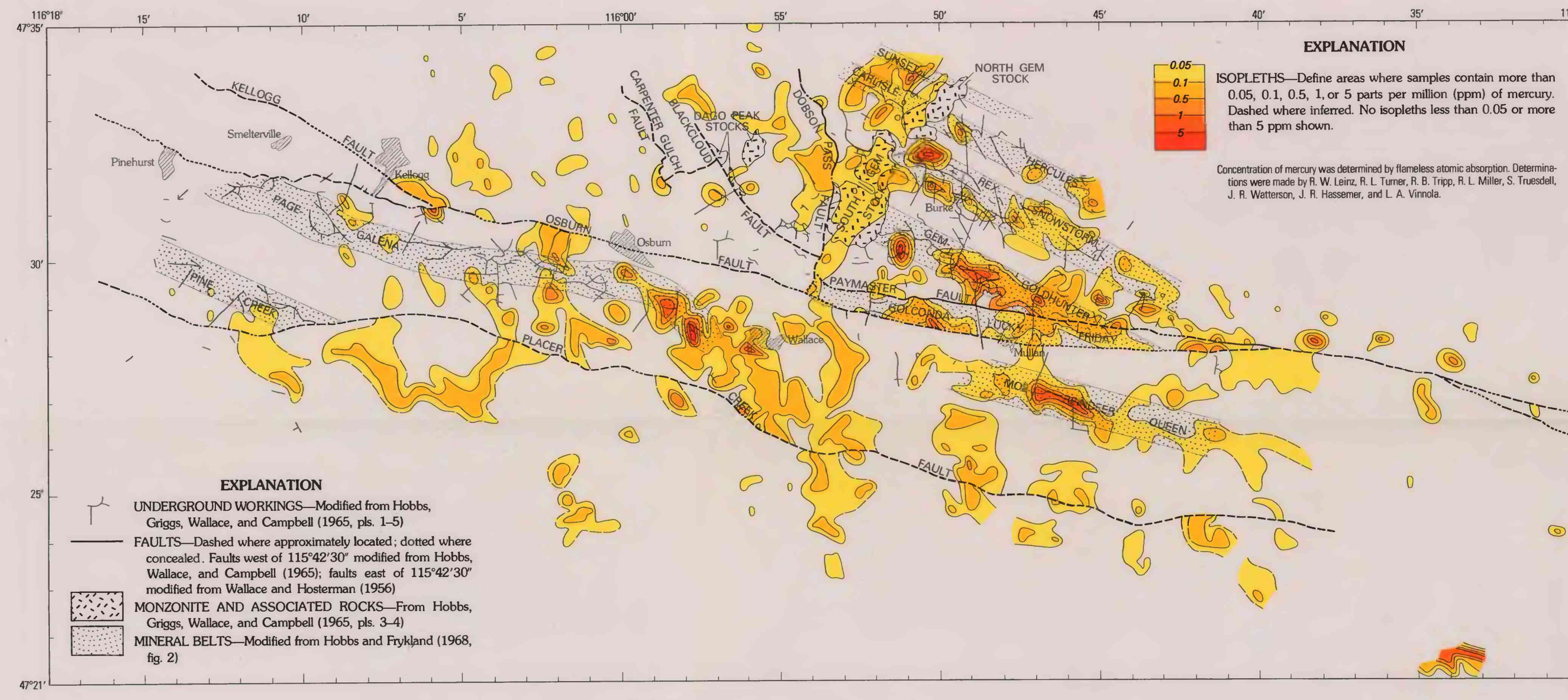
O. DISTRIBUTION OF MERCURY IN ROCKS
