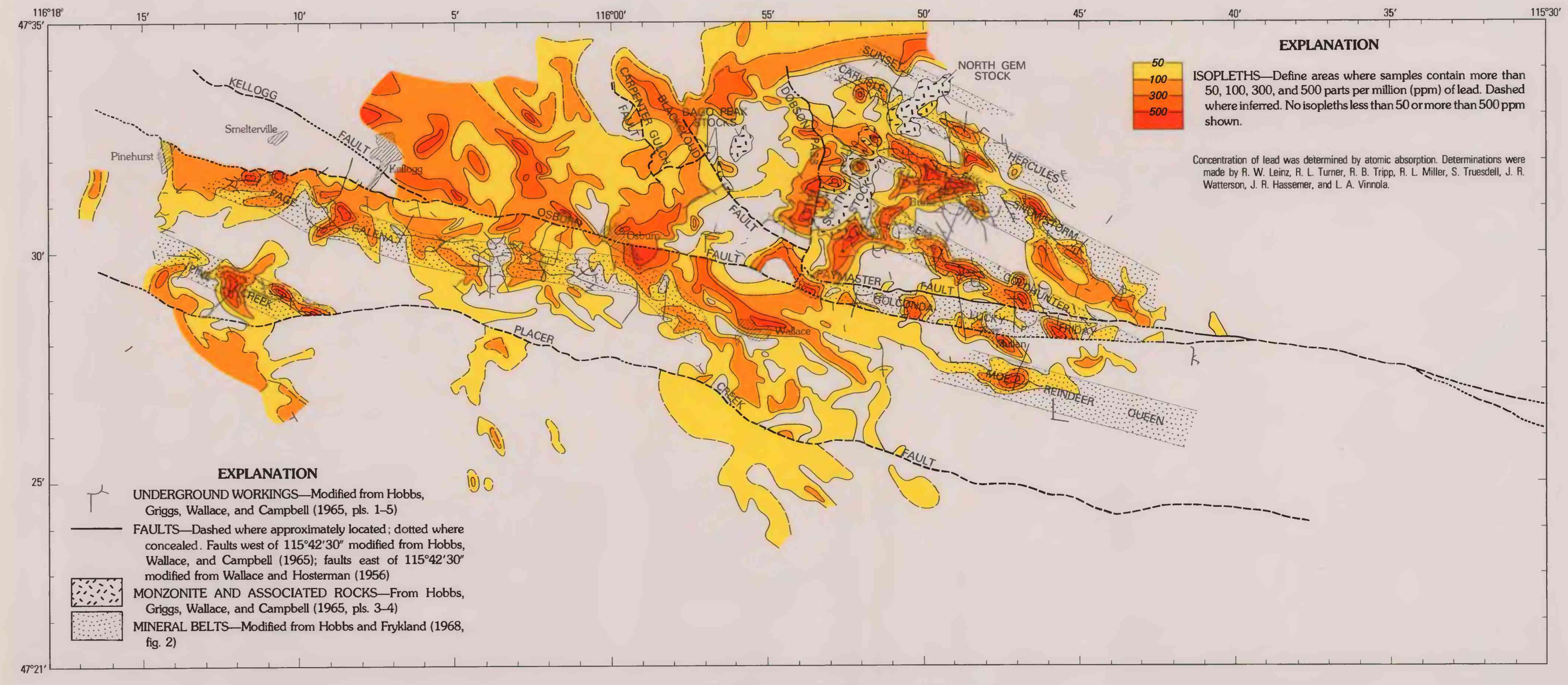
L. DISTRIBUTION OF LEAD IN SOILS
