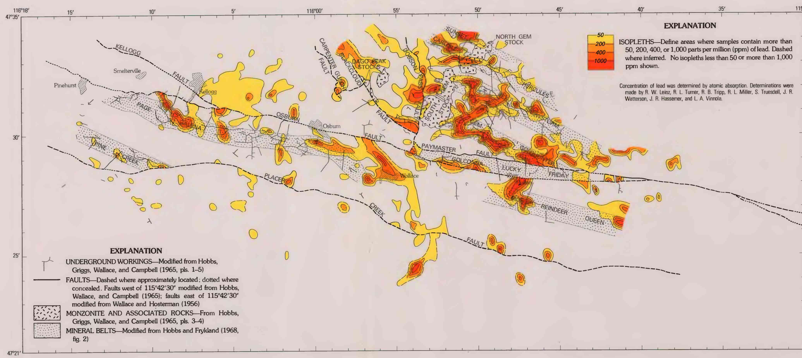
K. DISTRIBUTION OF LEAD IN ROCKS
