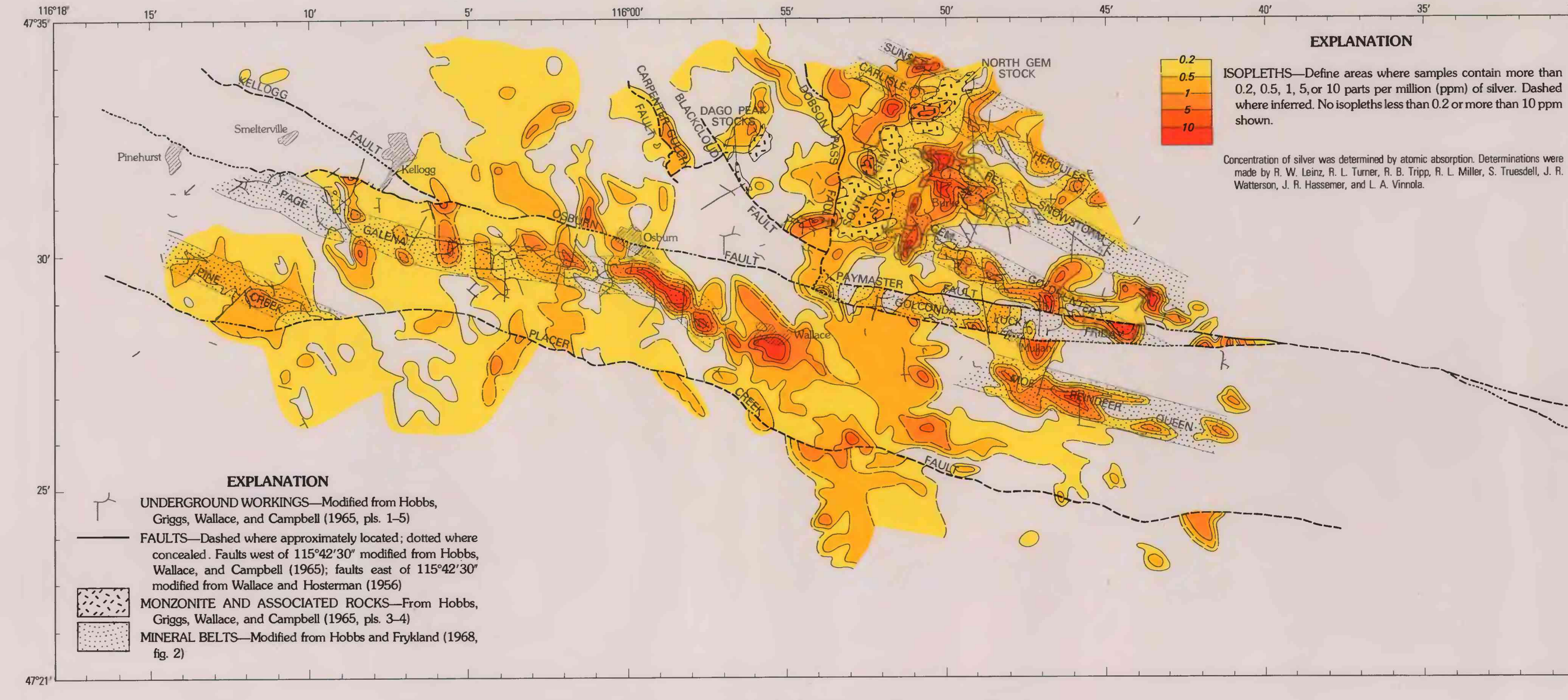
S. DISTRIBUTION OF SILVER IN ROCKS
