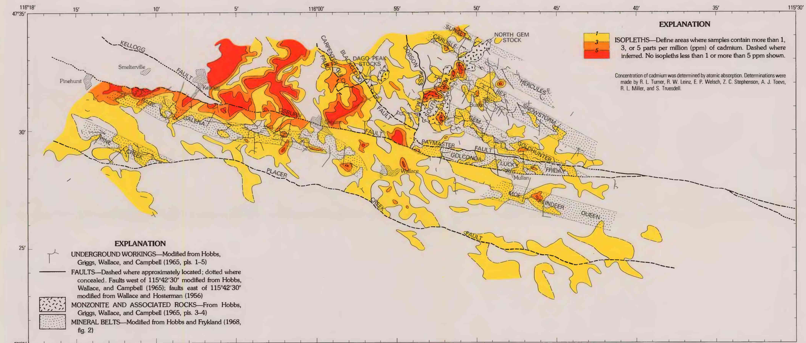
Z. DISTRIBUTION OF CADMIUM IN SOILS
