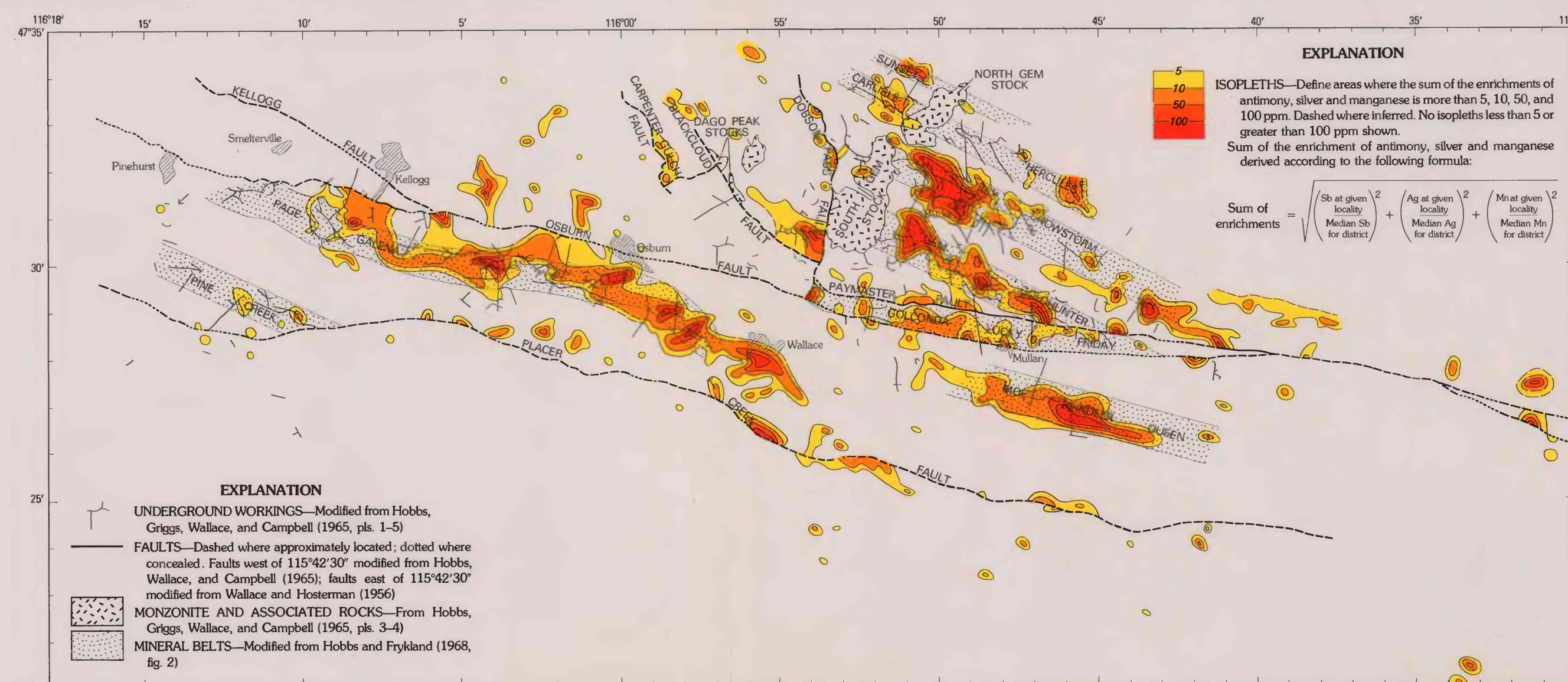
AA. SUM OF THE ENRICHMENTS ABOVE DISTRICT MEDIAN VALUES OF ANTIMONY, SILVER AND MANGANESE IN ROCKS
