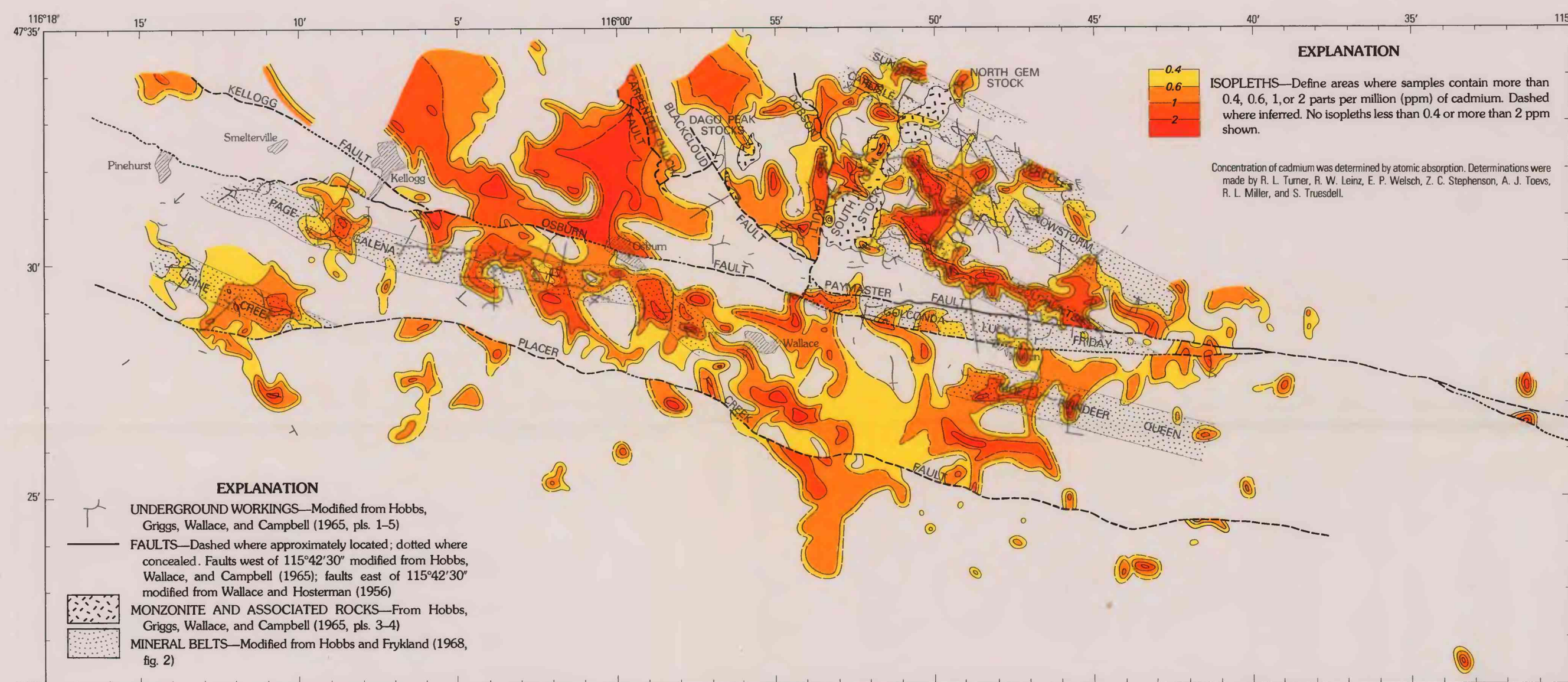
Y. DISTRIBUTION OF CADMIUM IN ROCKS
