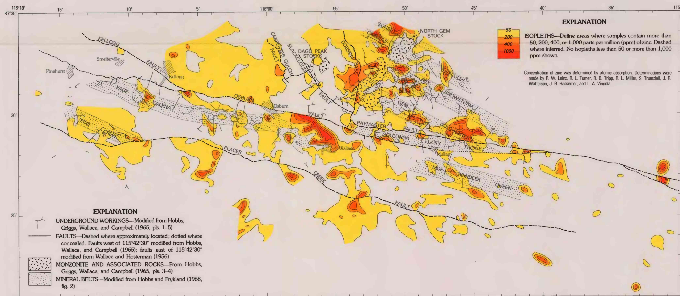
W. DISTRIBUTION OF ZINC IN ROCKS
