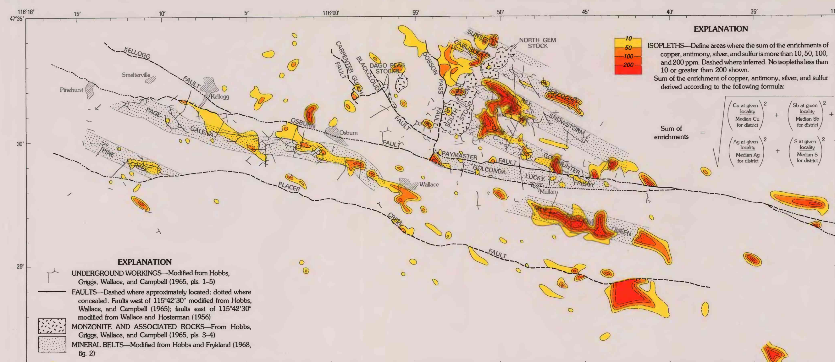
BB. SUM OF THE ENRICHMENTS IN ROCKS ABOVE THE DISTRICT MEDIAN VALUES OF COPPER, ANTIMONY, SILVER AND SULFUR
