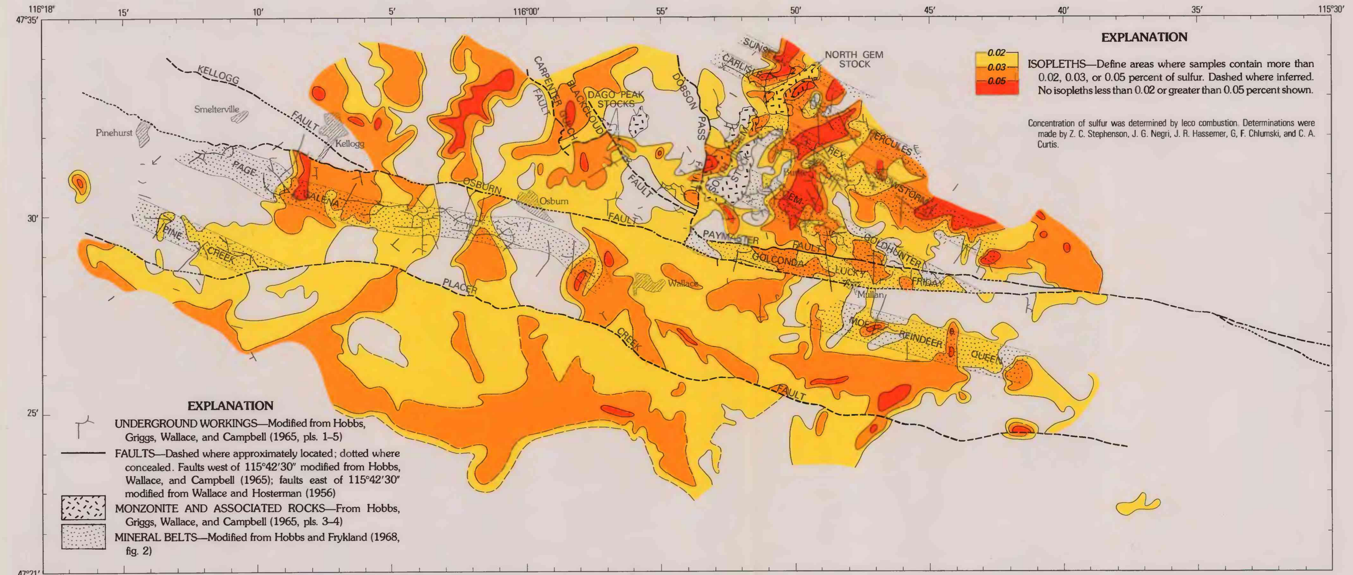
V. DISTRIBUTION OF SULFUR IN SOILS
