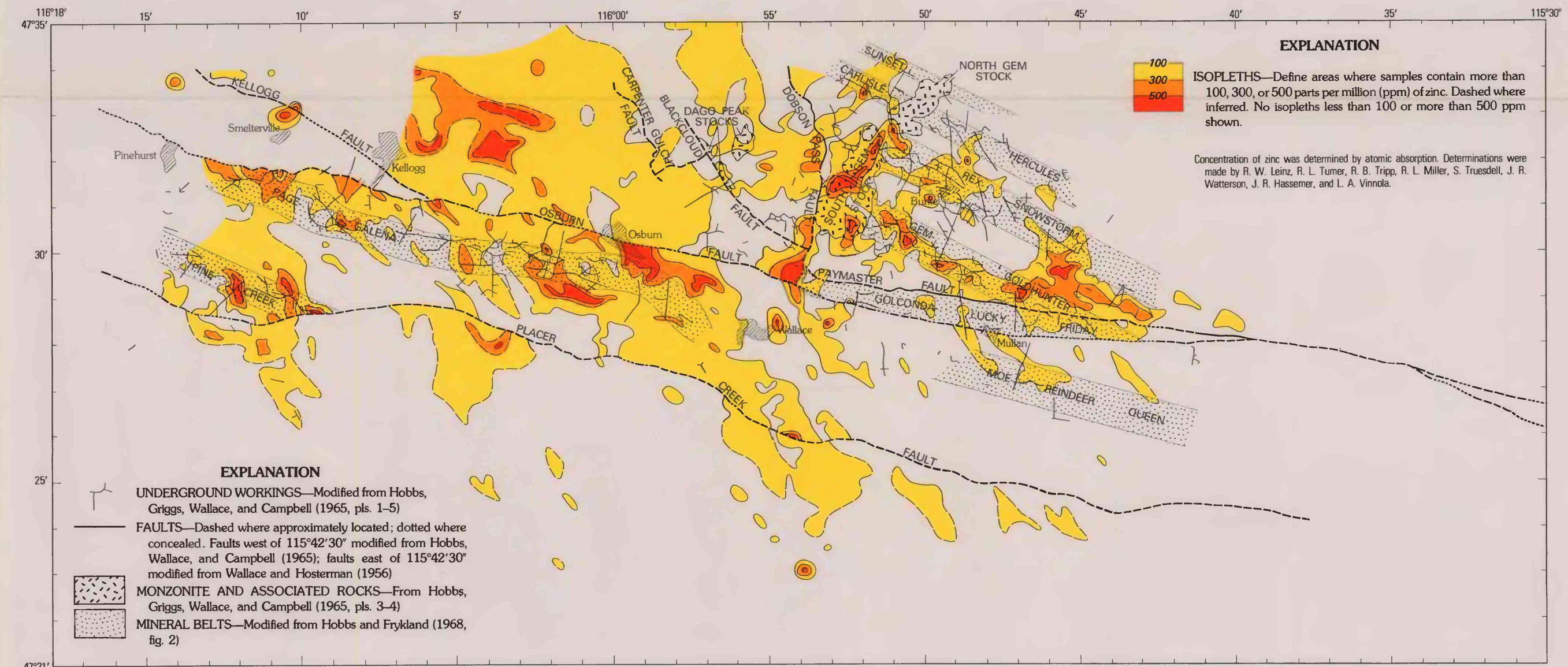
X. DISTRIBUTION OF ZINC IN SOILS
