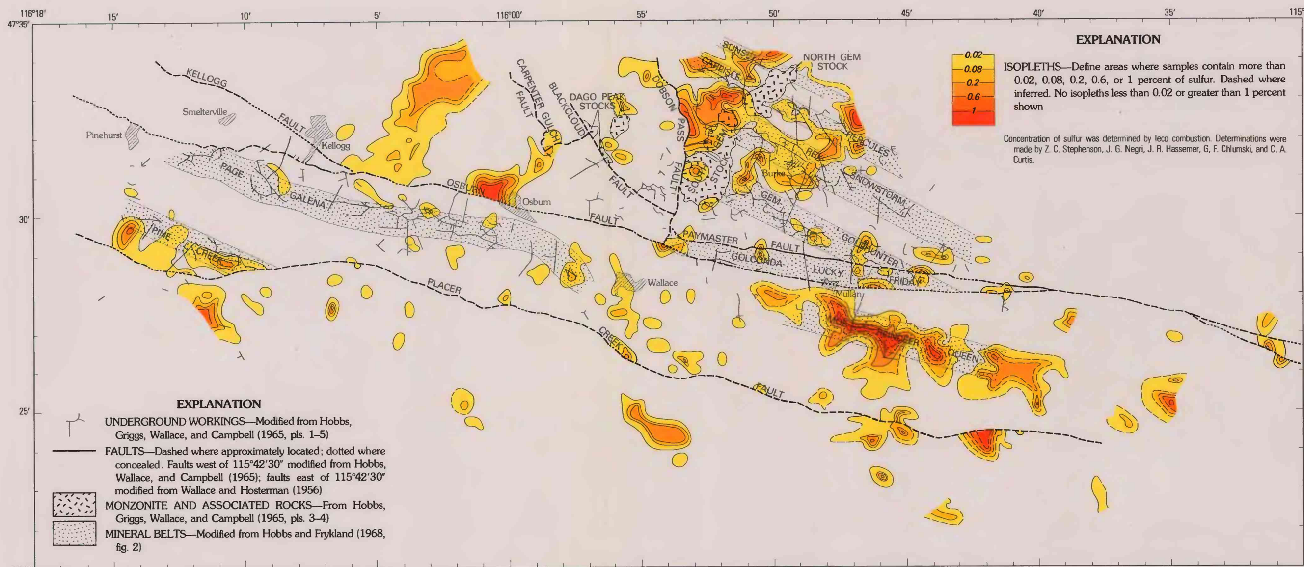
U. DISTRIBUTION OF SULFUR IN ROCKS
