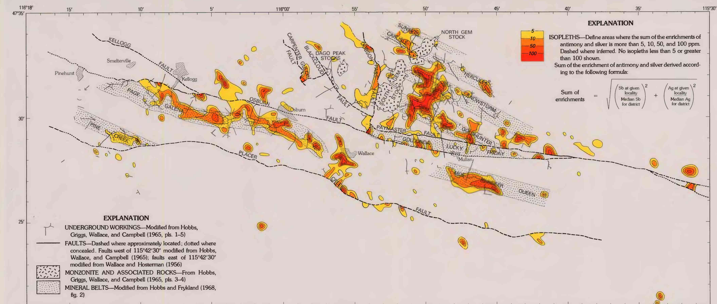
CC. SUM OF THE ENRICHMENTS IN ROCKS ABOVE THE DISTRICT MEDIAN VALUES OF ANTIMONY AND SILVER
