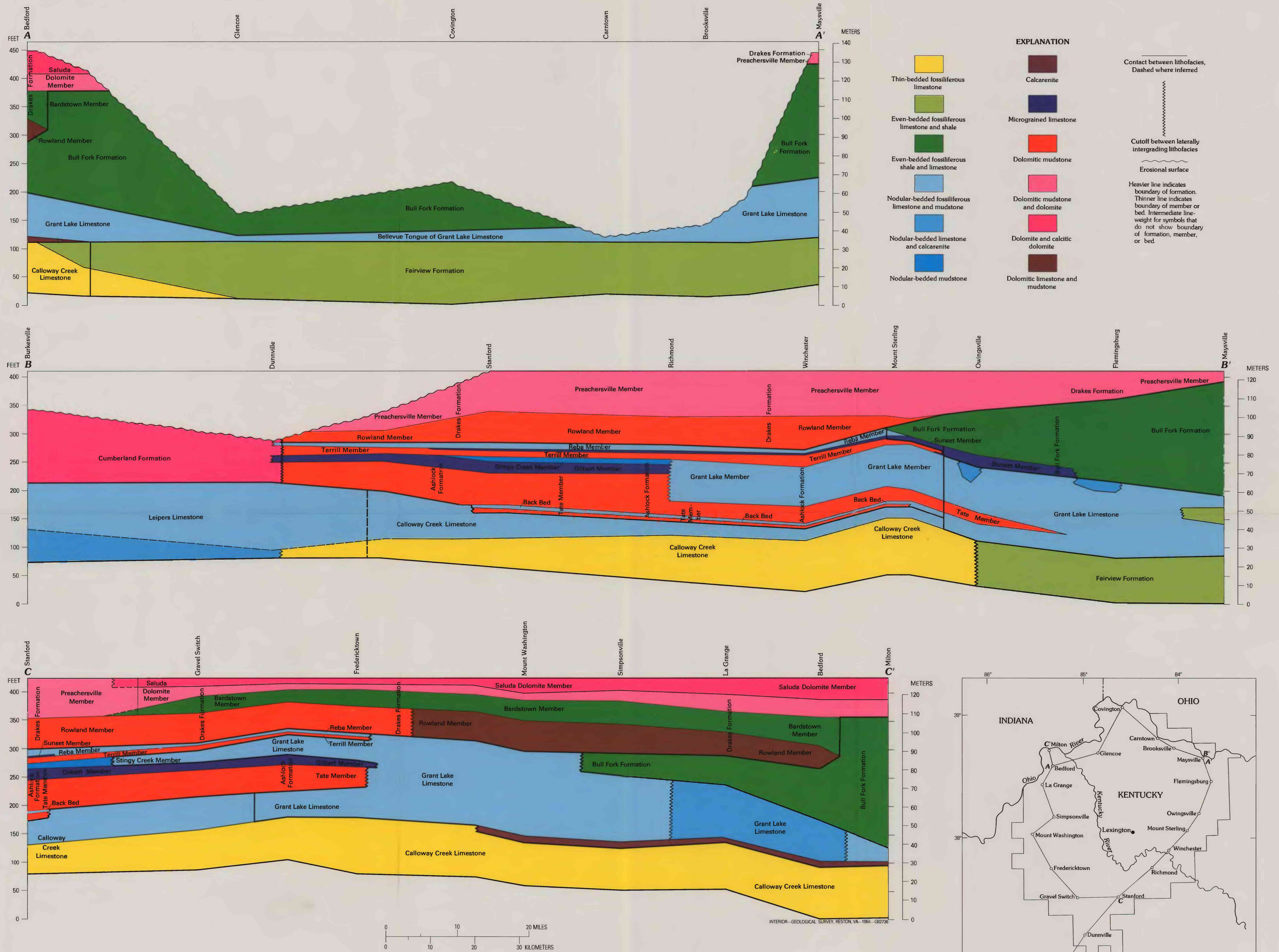
LITHOFACIES AND STRATIGRAPHIC NOMENCLATURE OF THE FAIRVIEW FORMATION, CALLOWAY CREEK LIMESTONE, AND YOUNGER ORDOVICIAN FORMATIONS IN KENTUCKY. ORDOVICIAN SEQUENCE IS OVERLAIN BY SILURIAN OR DEVONIAN ROCKS (SEE FIG. 8).
