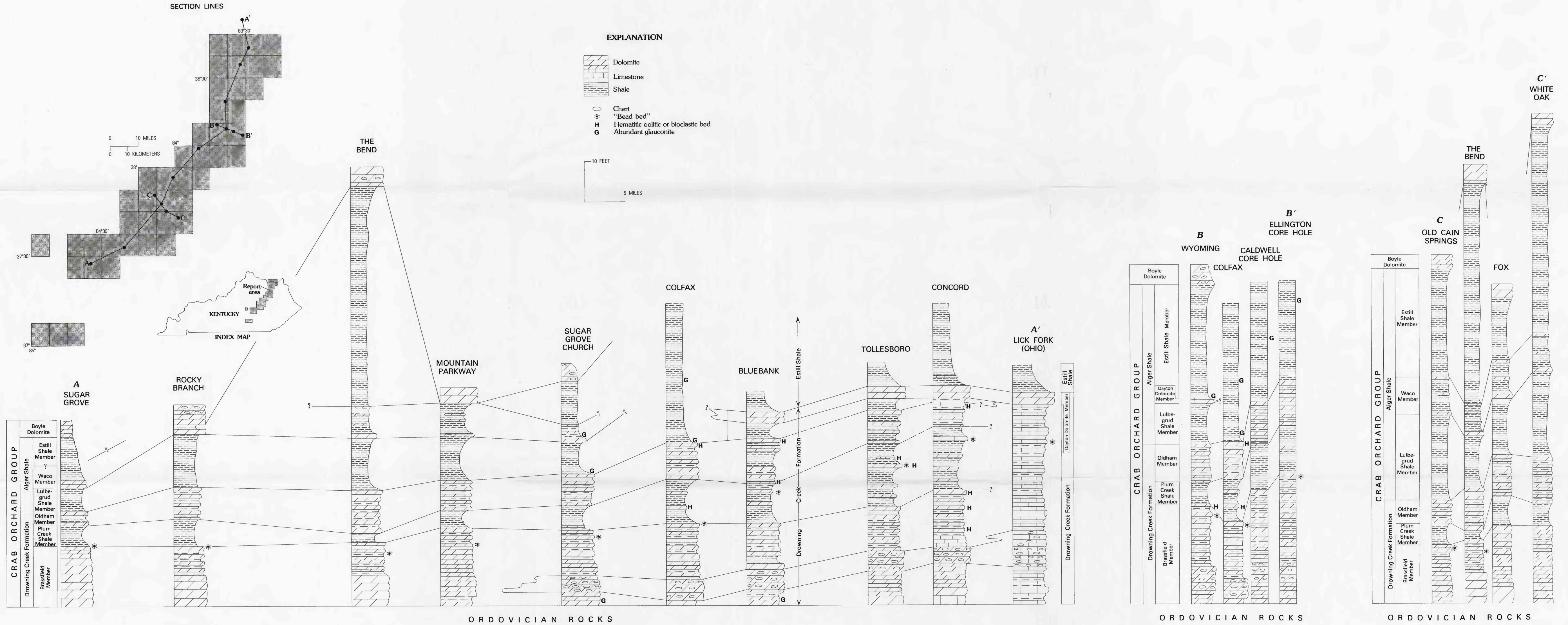
STRATIGRAPHIC SECTIONS OF THE CRAB ORCHARD GROUP, EAST-CENTRAL KENTUCKY
