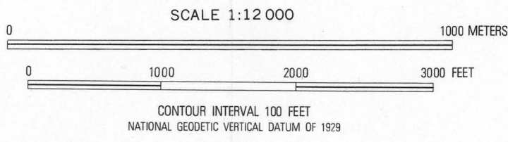
GEOLOGIC MAP OF PART OF THE HUMBOLDT RANGE, NEVADA, SHOWING COLLECTING SITES A, B, AND C
