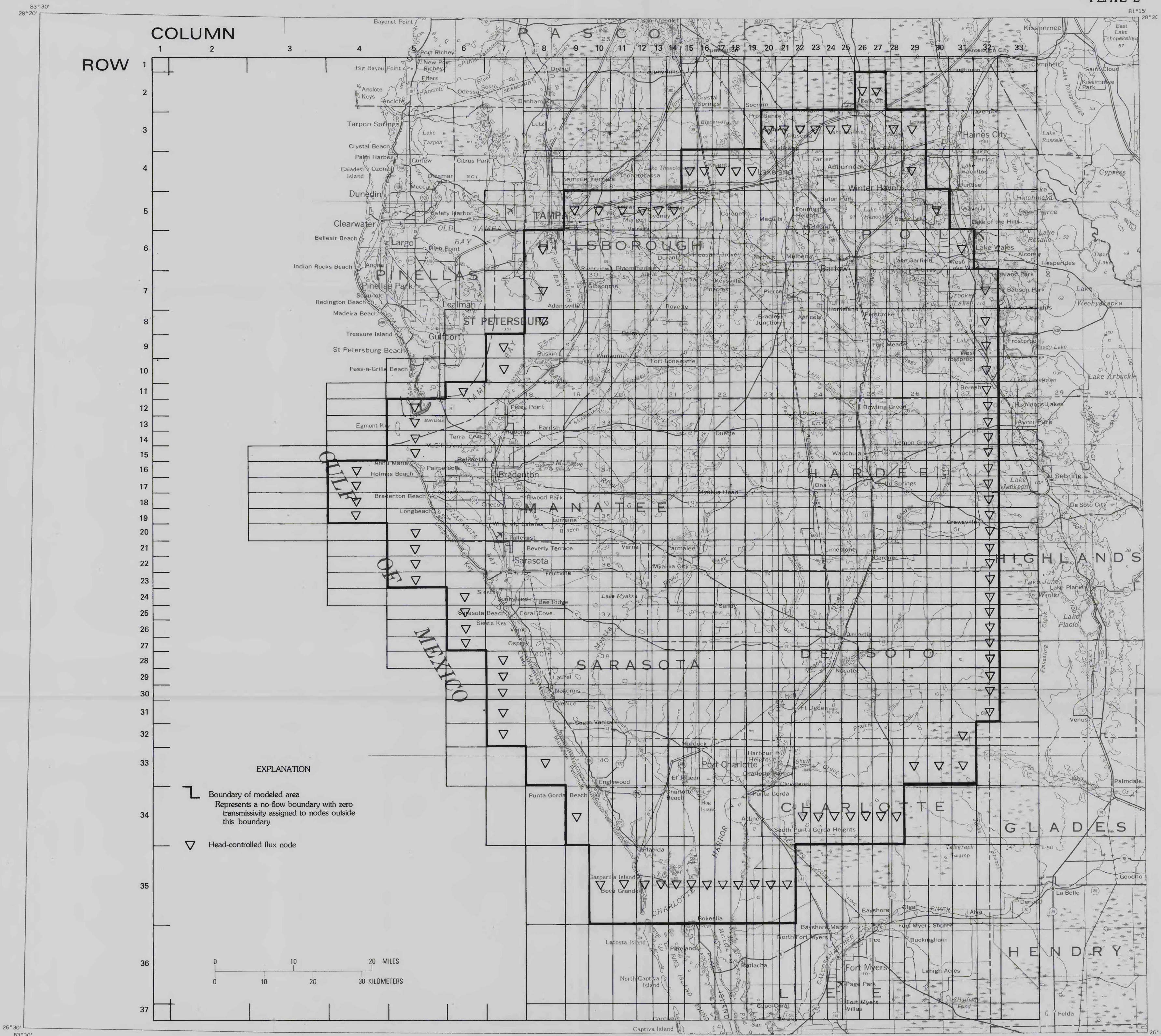
MAP SHOWING GRID NETWORK AND BOUNDARY OF MODELED AREA, WEST-CENTRAL FLORIDA
