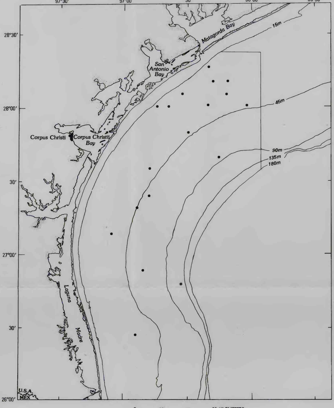
Distribution of unidentified sipunculid.
