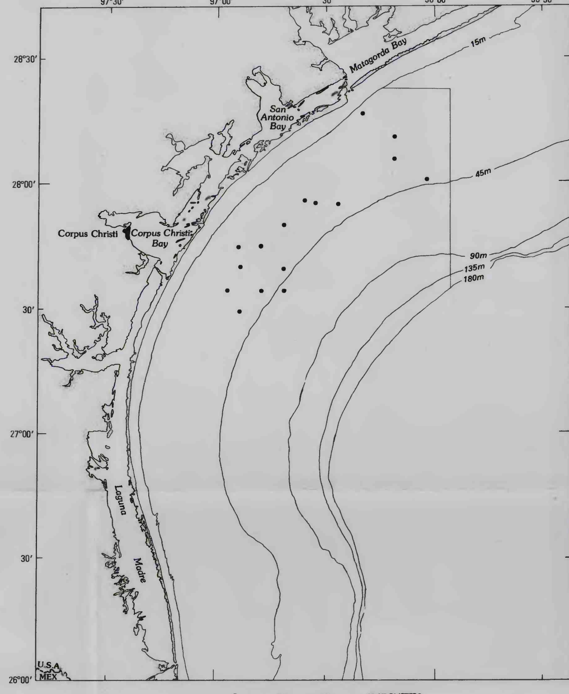
Distribution of Armandia maculata .
