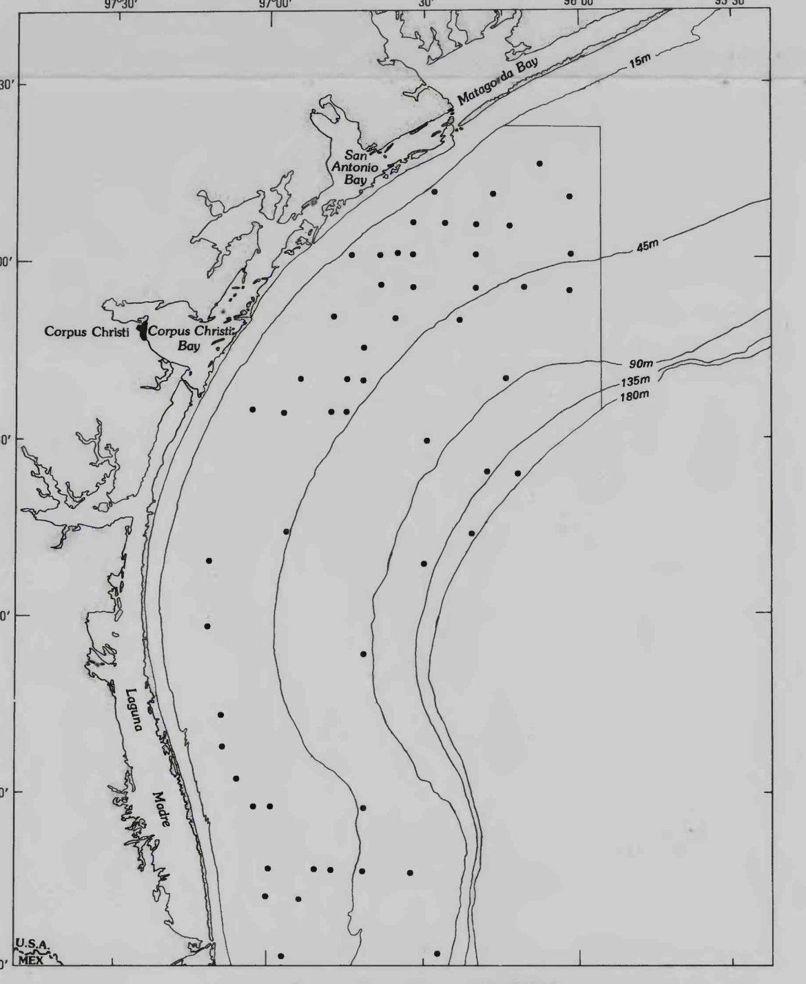
Distribution of Ampelicea cristoides .
