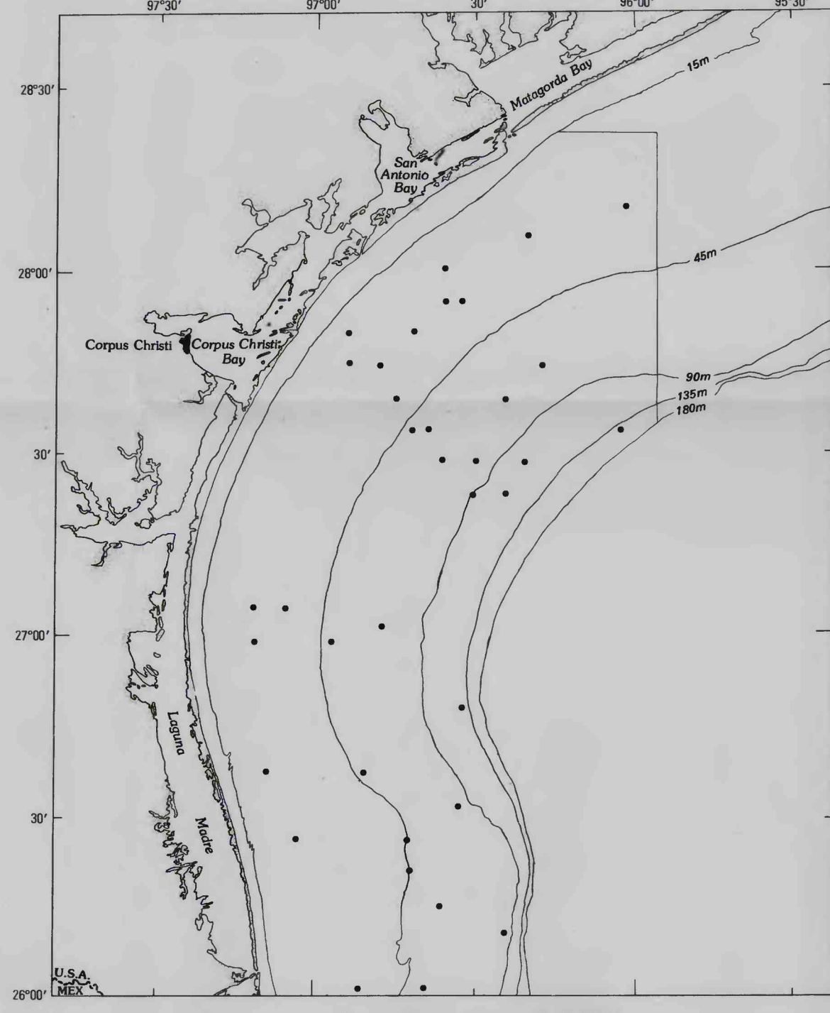
Distribution of Sigambra tentaculata .
