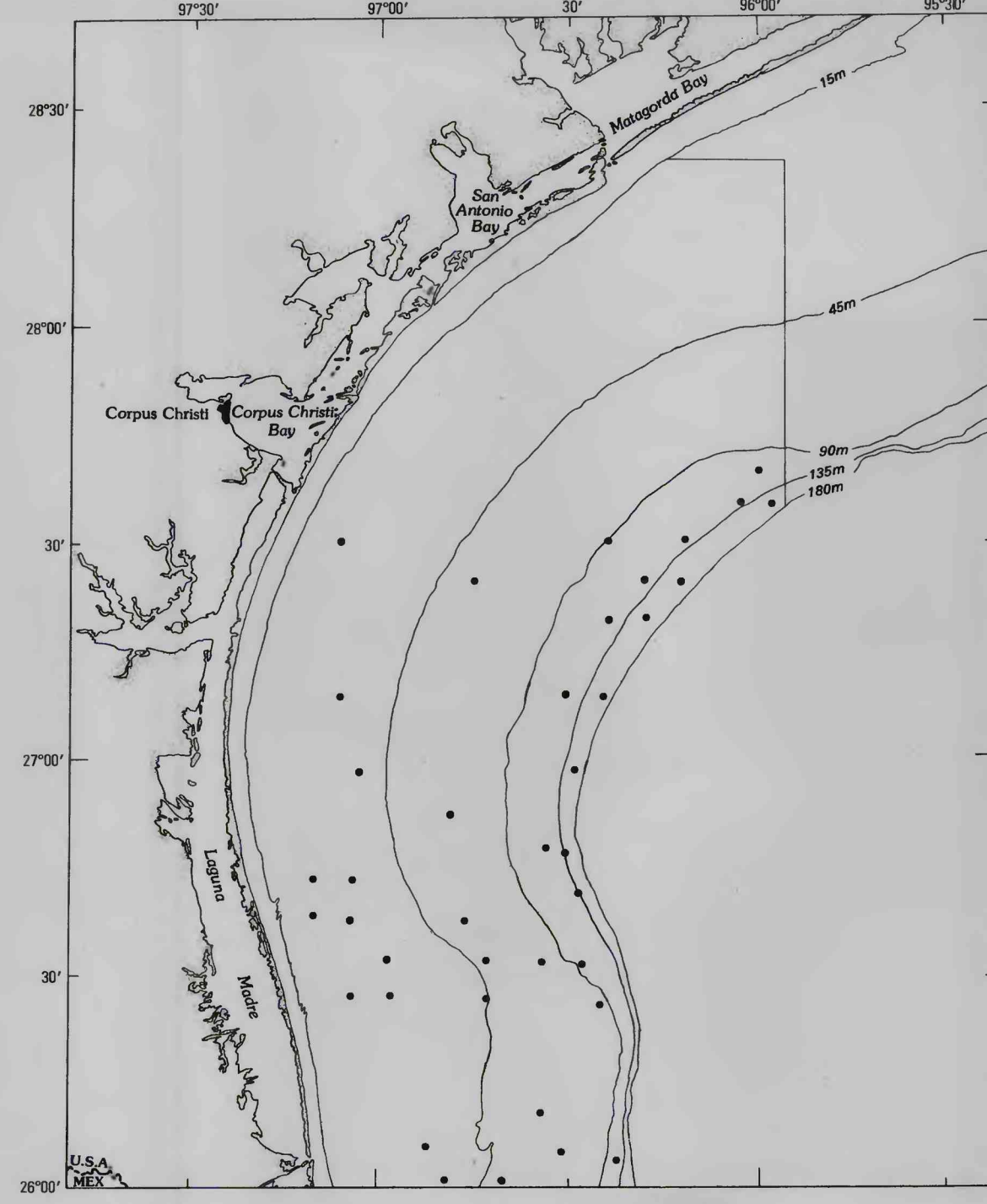
Distribution of an unidentified echiurid.
