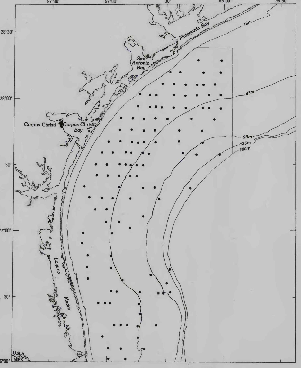
Distribution of Paraprionospio pinnata .
