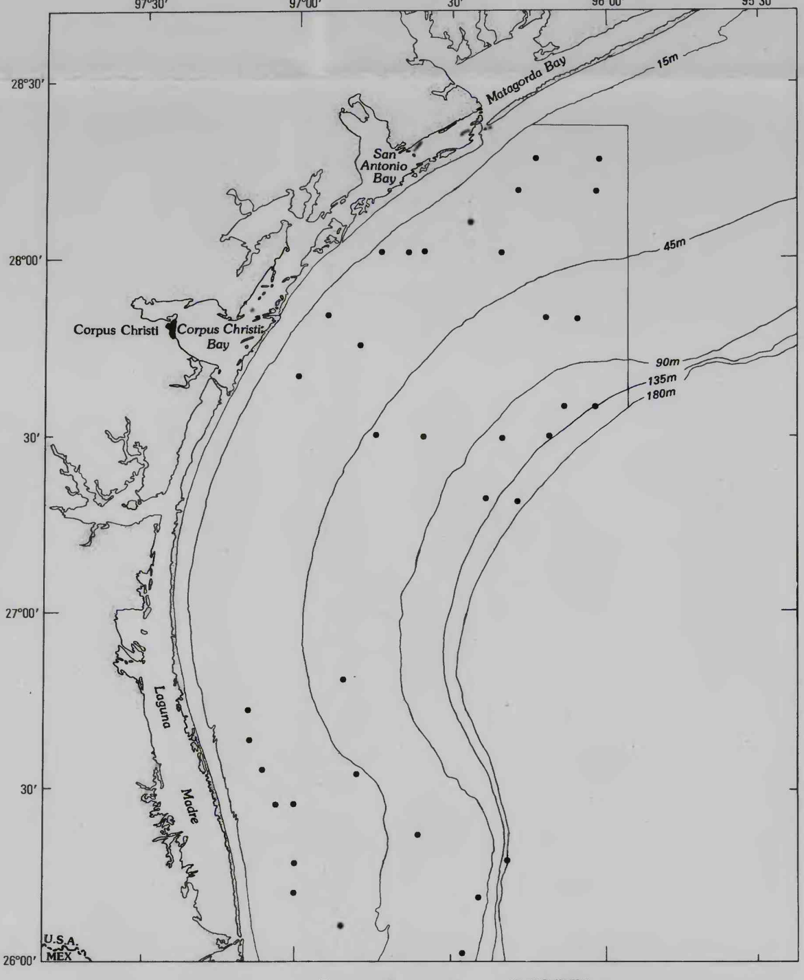
Distribution of Onuphis sp.
