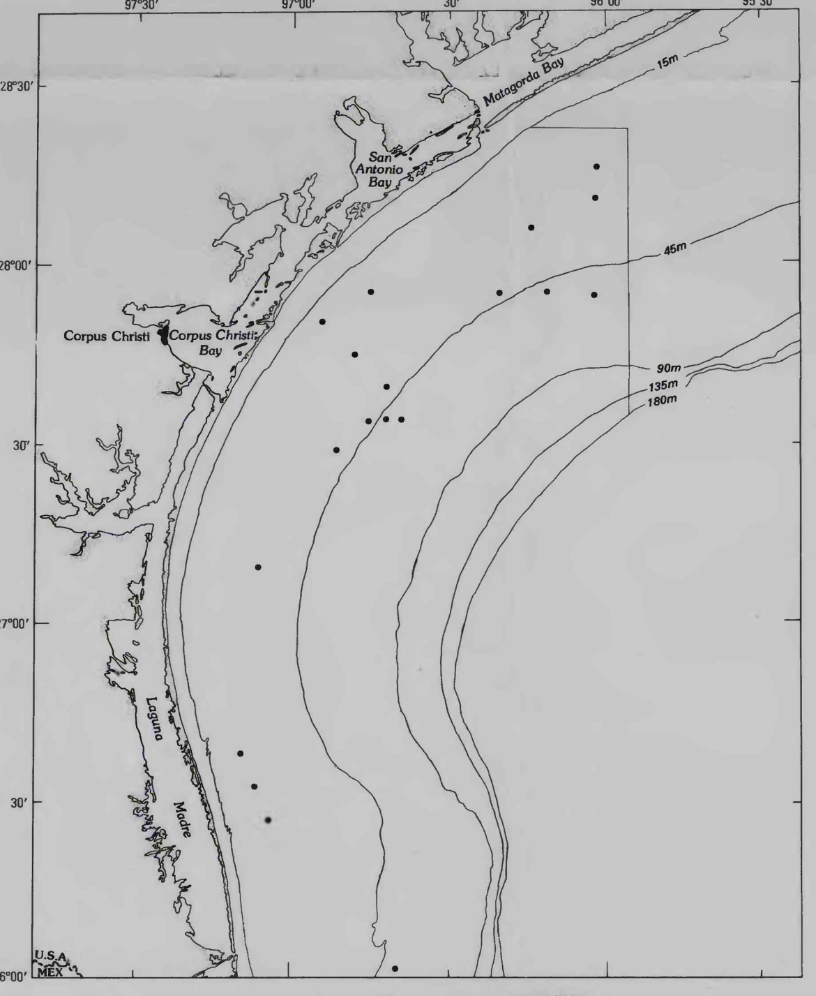
Distribution of Speocarcinus sp.
