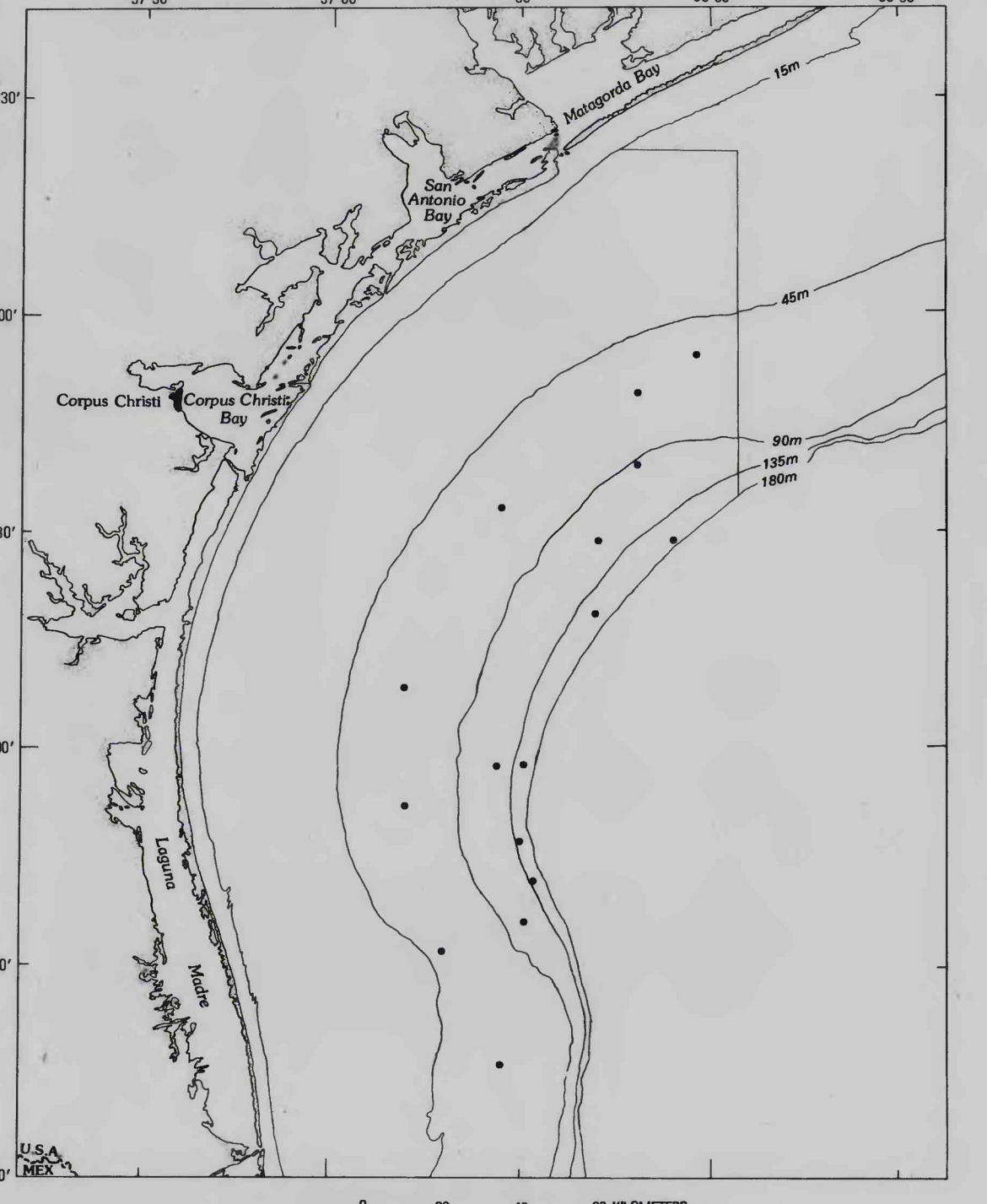
Distribution of Diploporia sp.
