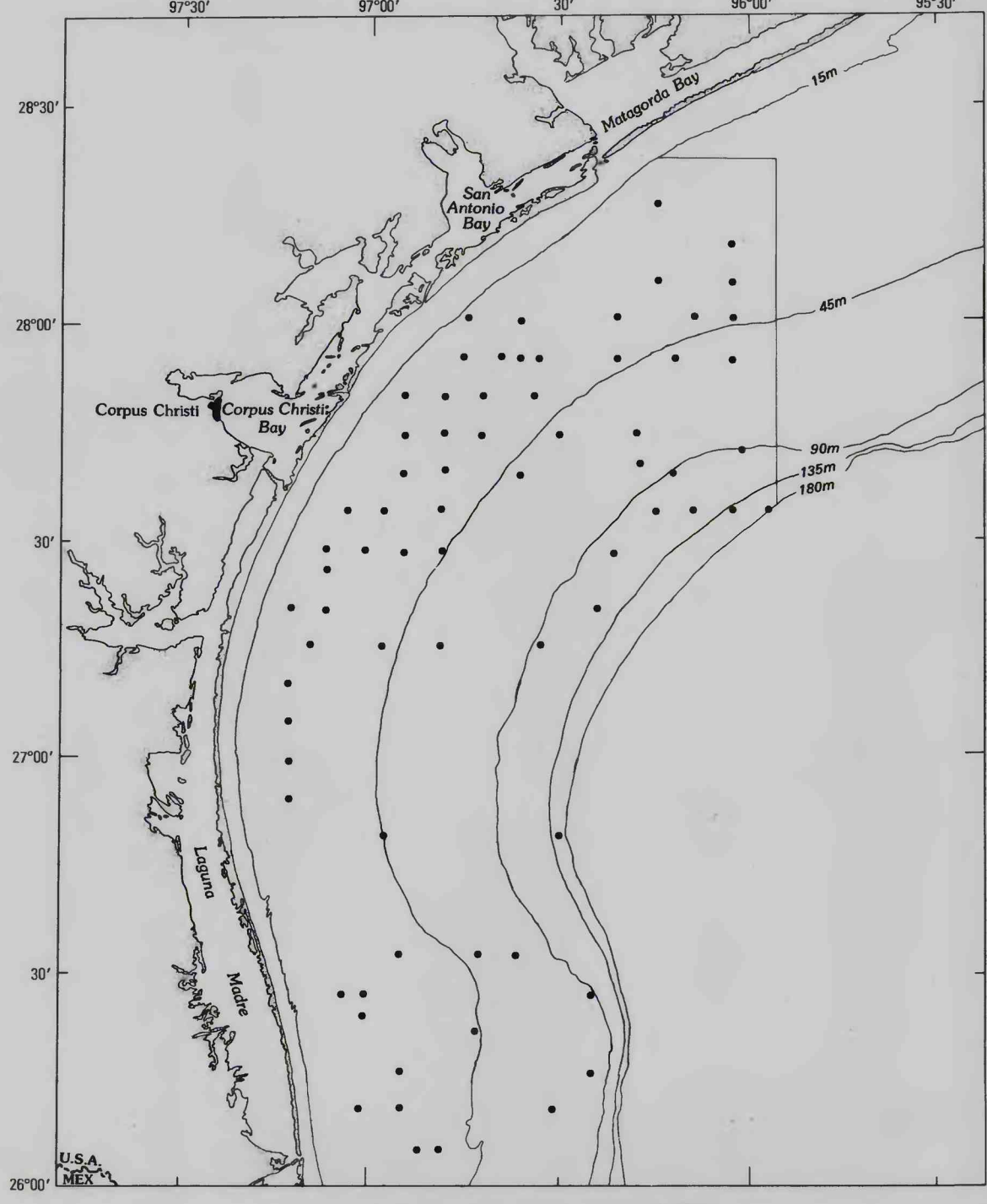
Distribution of Ampelicea cf. cucullata .
