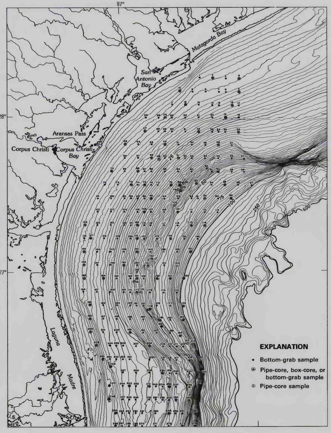
Location of benthic sample stations for geologic studies. Isobaths in fathoms.
