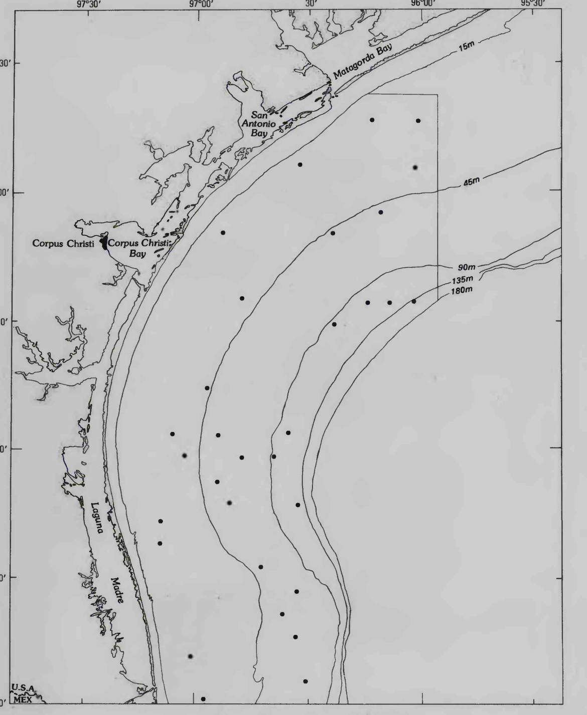
Distribution of an unidentified pararonid.
