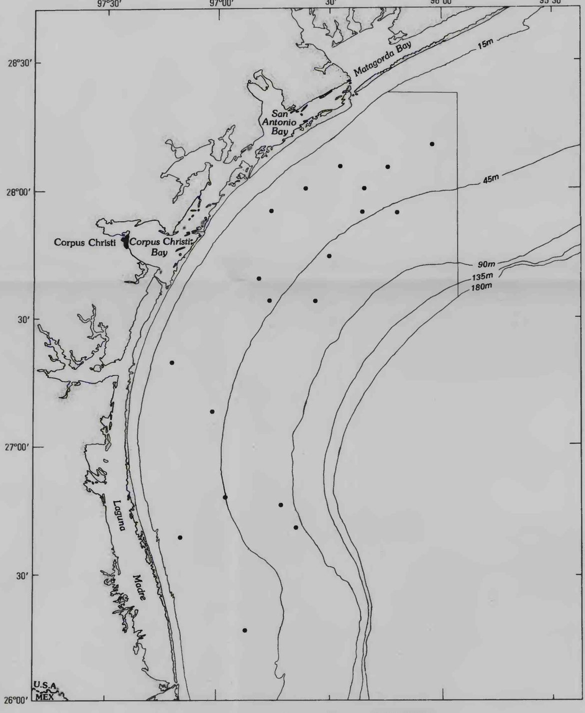
Distribution of Armandia agilis .
