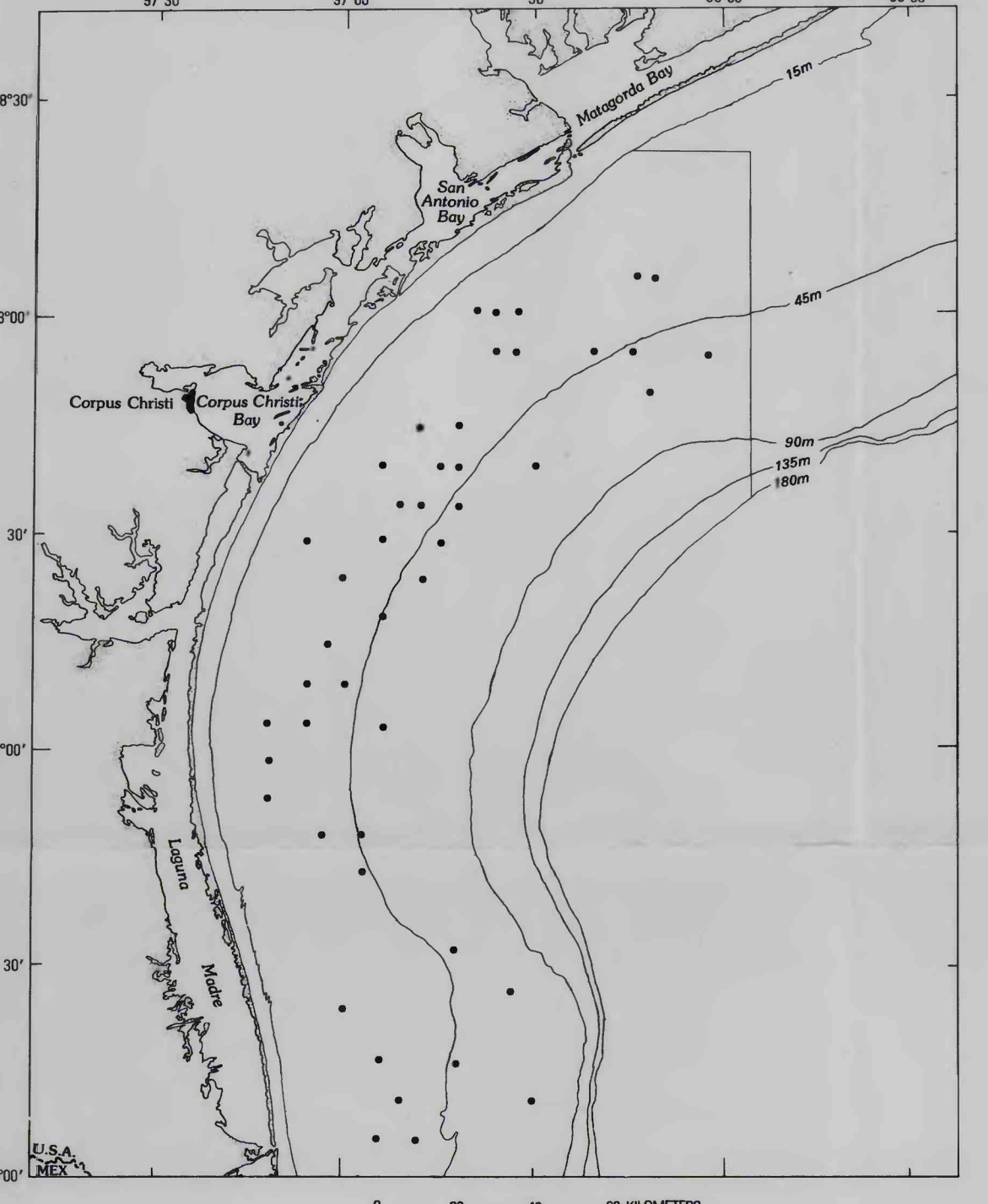
Distribution of Eudorella monodon .
