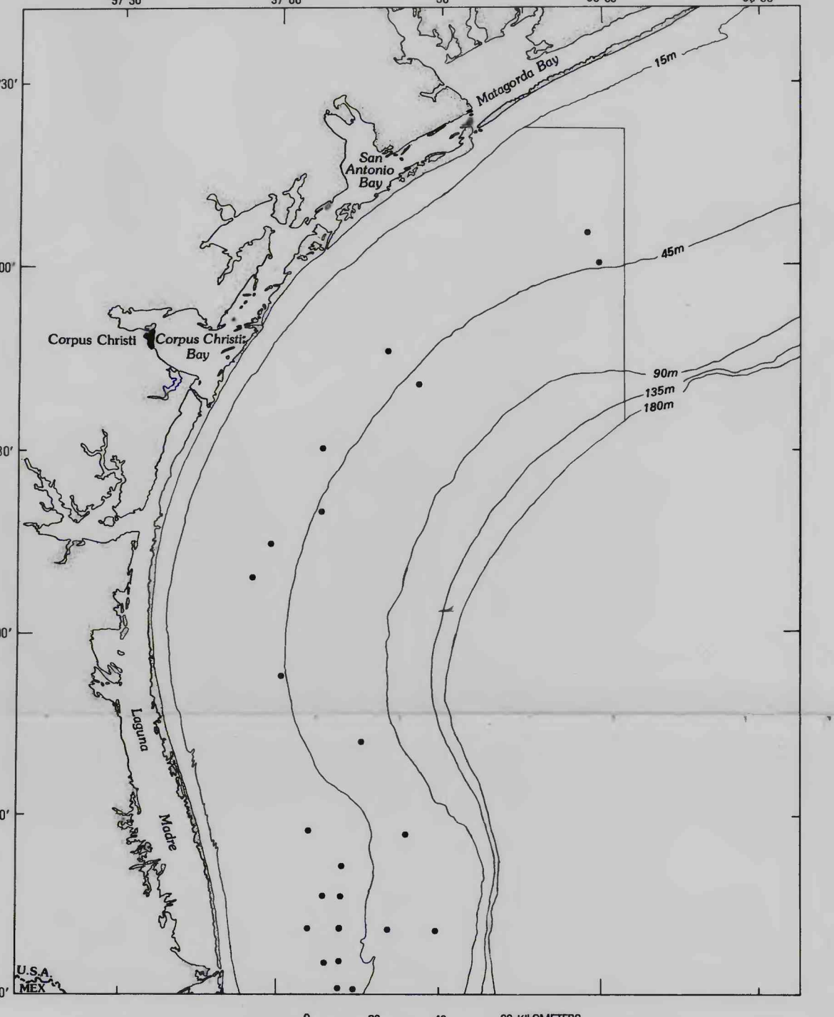
Distribution of Pinna retifera .
