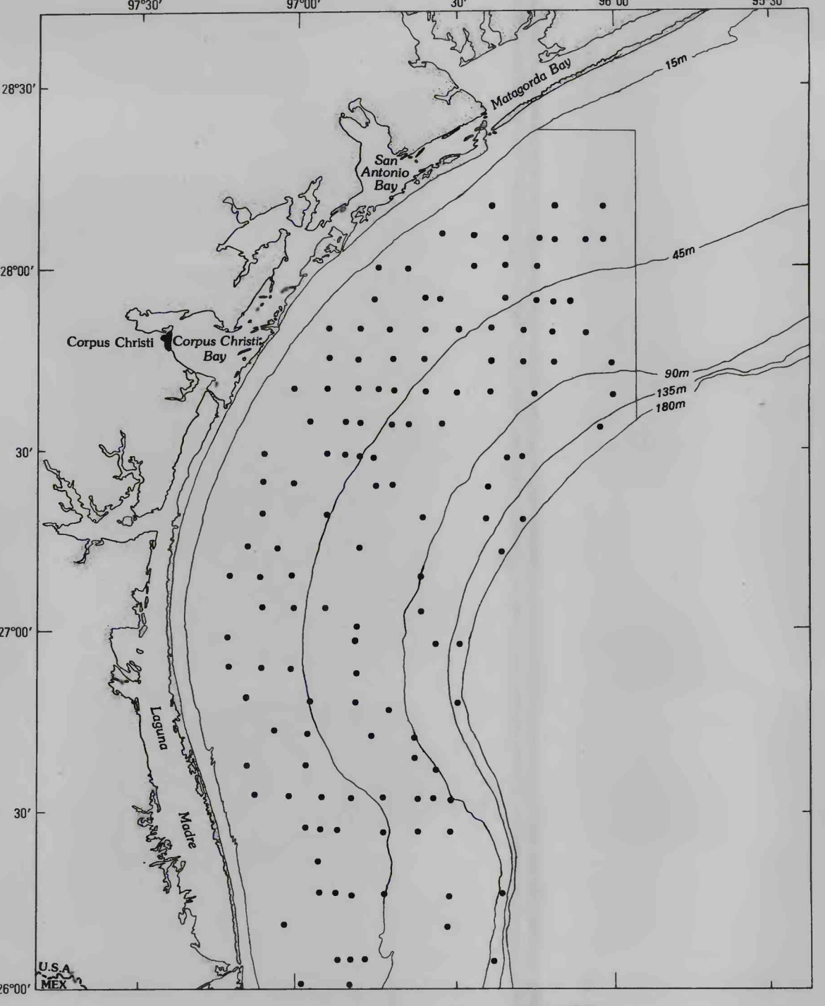
Distribution of Nephysa picta .
