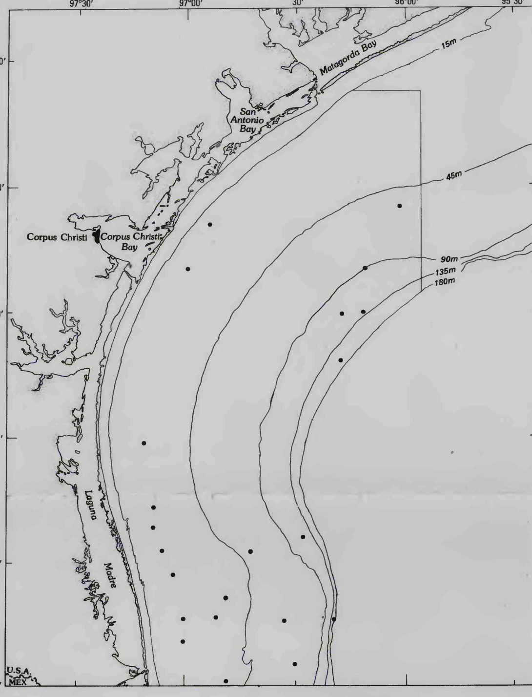
Distribution of Nuculana acuta .
