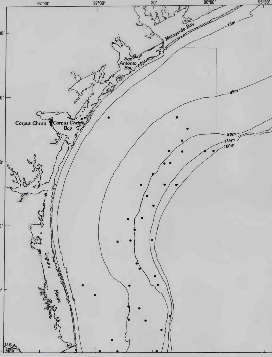
Distribution of Glycera sp.
