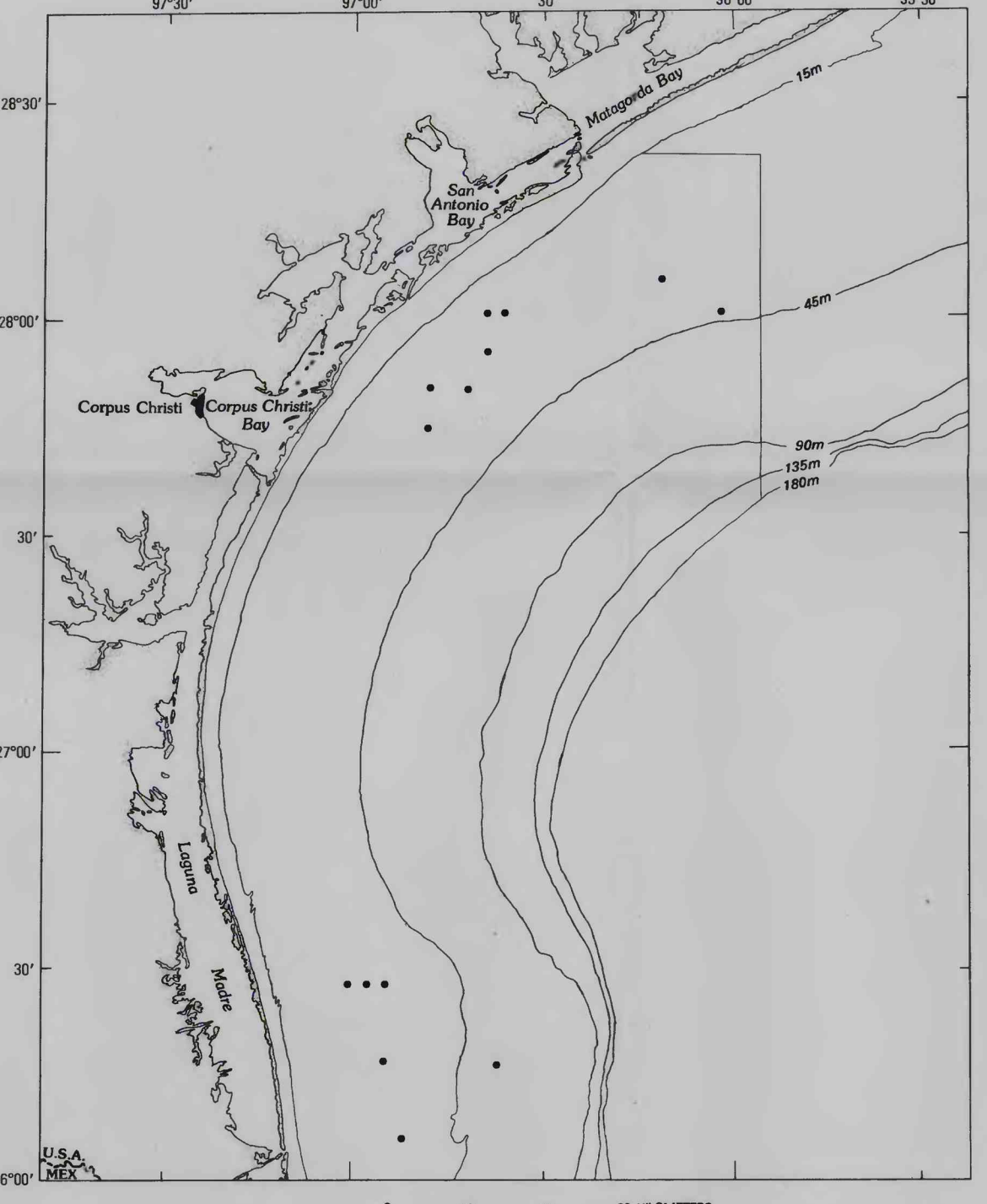
Distribution of Ampelicea cf. cristata .
