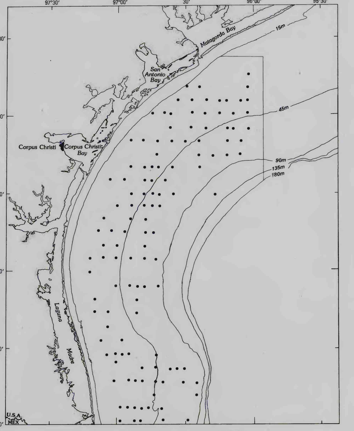
Distribution of Magelona sp.
