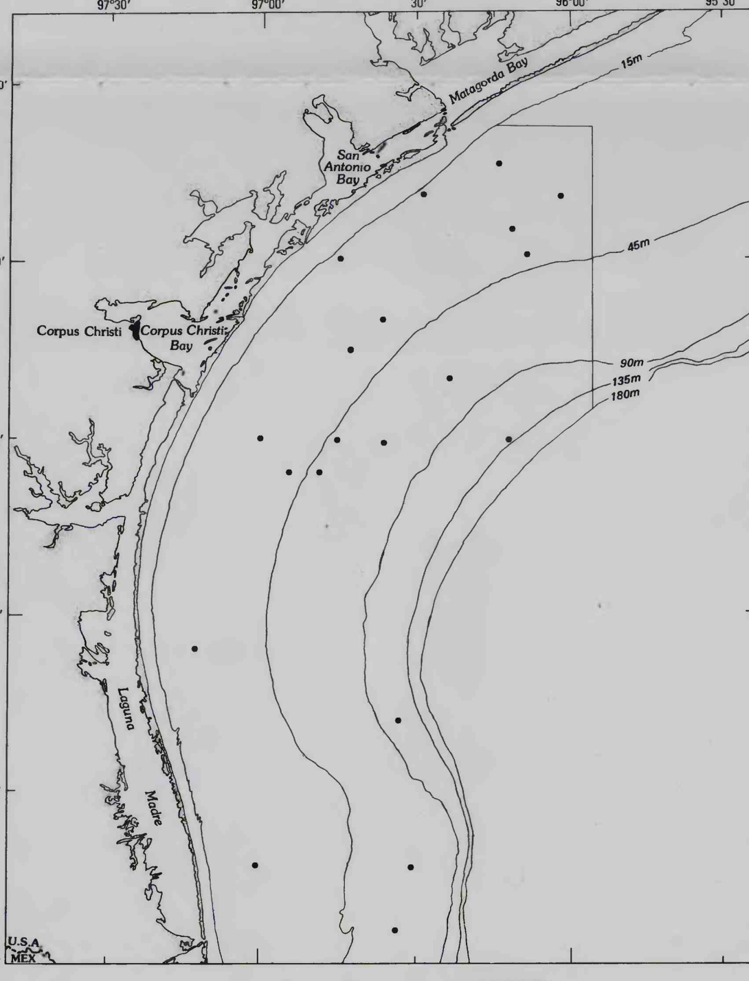
Distribution of Chamocarcinus mississippiensis .
