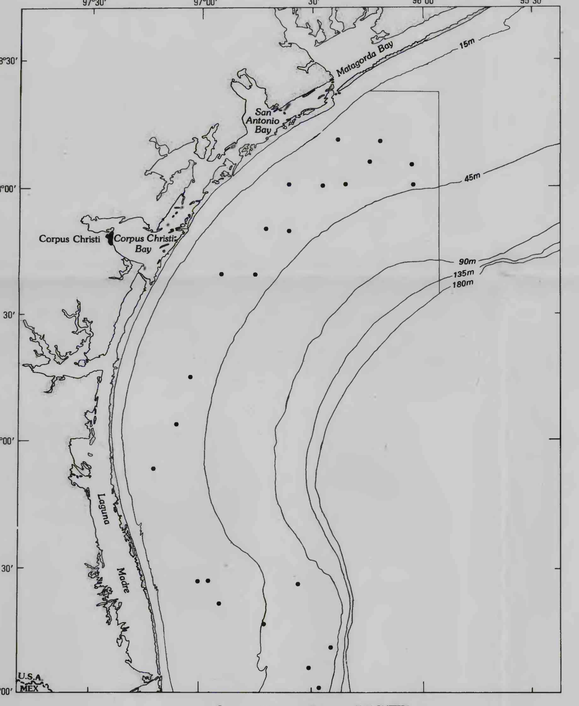
Distribution of Nitomastus latericus .
