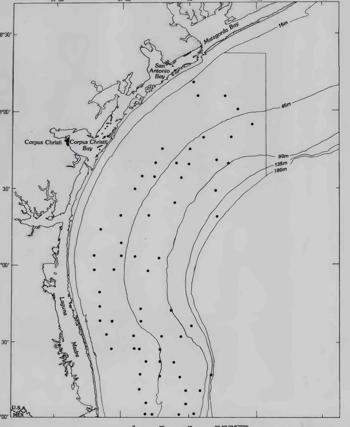
Distribution of Corbula sp.
