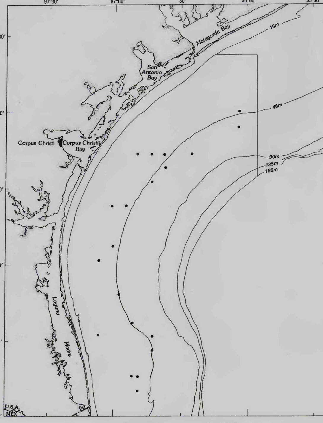
Distribution of Leptognathia gracilis .
