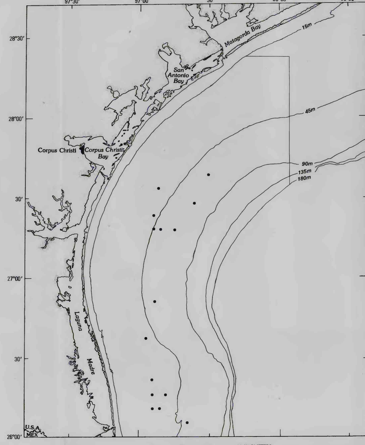
Distribution of an unidentified gastropod.
