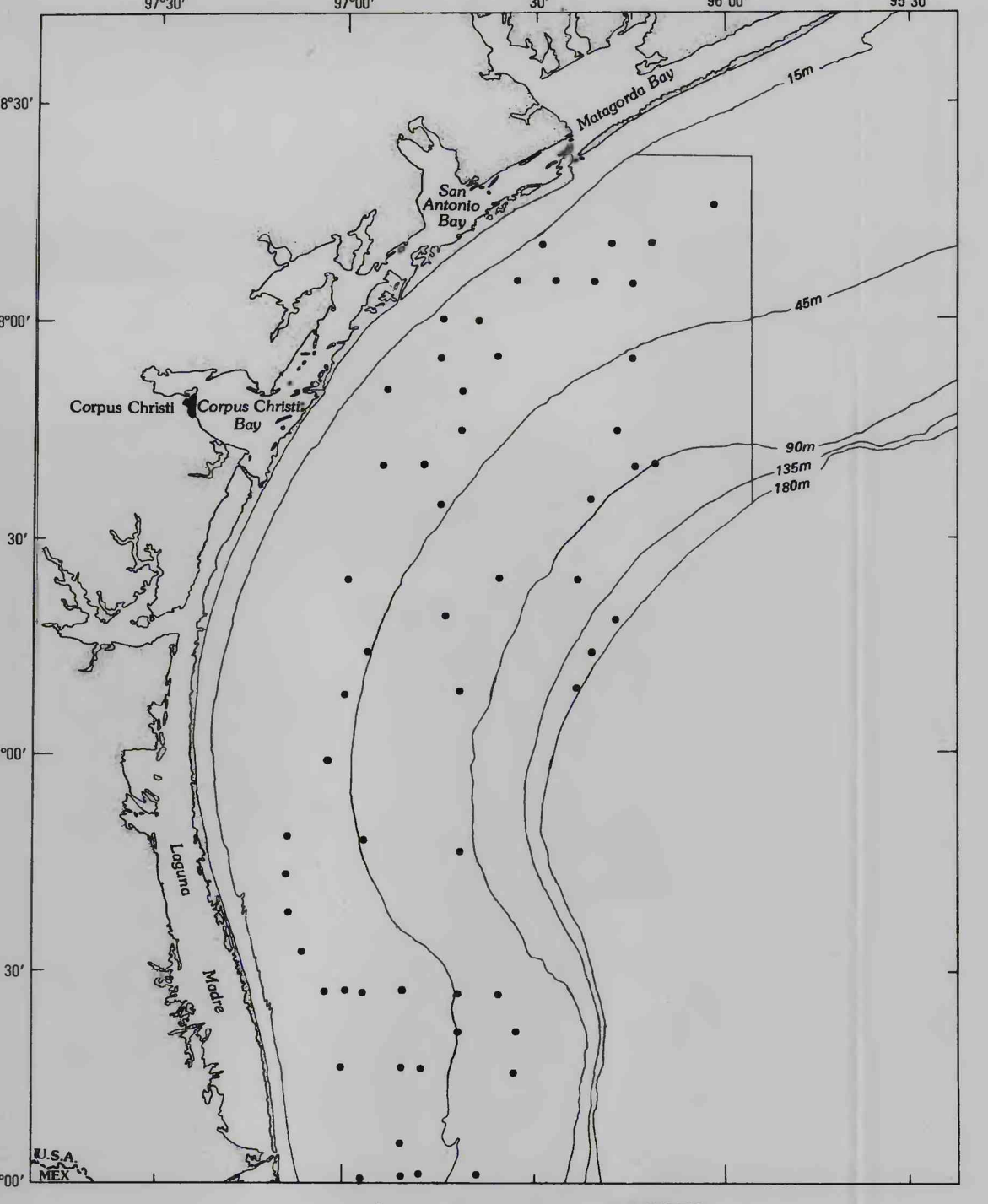
Distribution of Lumbrineris sp.
