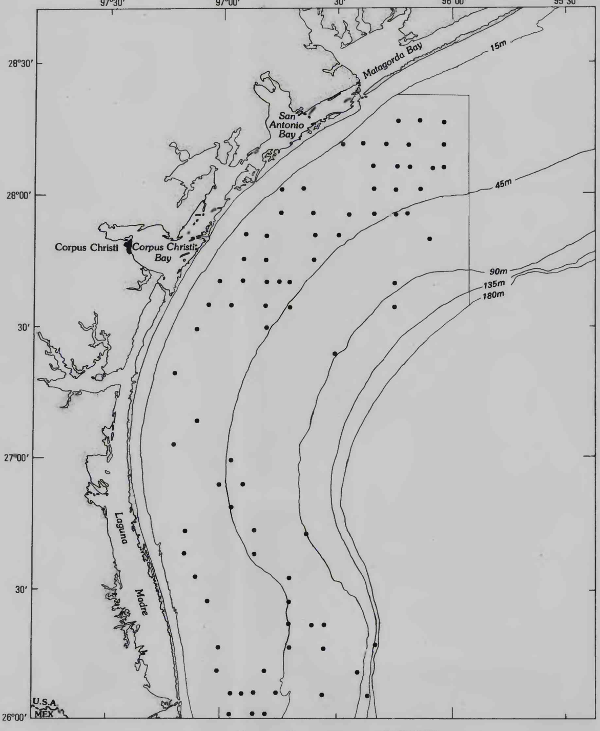
Distribution of Nereis sp.
