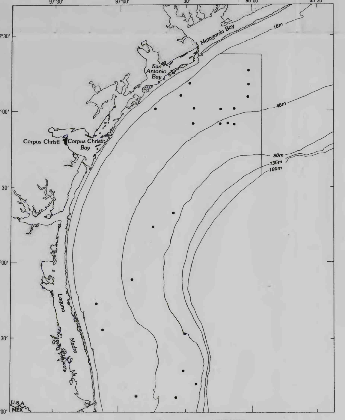
Distribution of an unidentified malacostrac.
