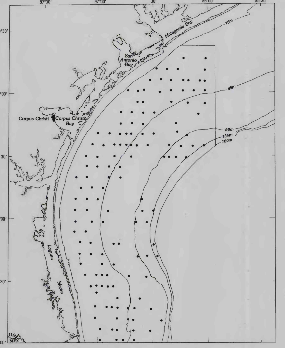
Distribution of unidentified nemertean.
