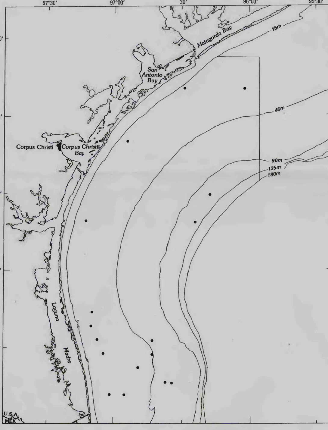
Distribution of Nuculana concentrica .
