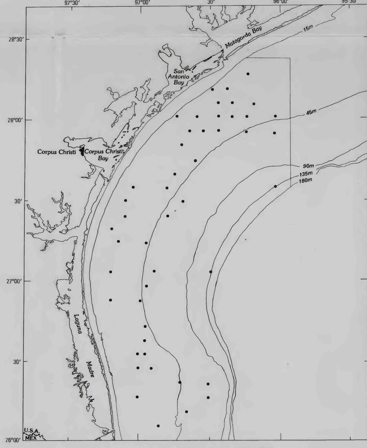
Distribution of Ninoe nigripes .
