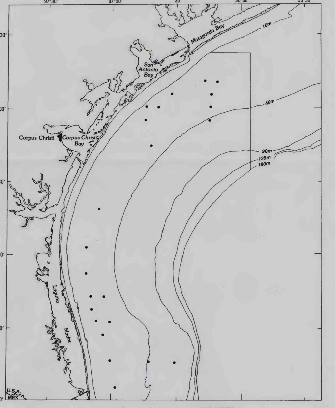
Distribution of Diopatra cuprea .
