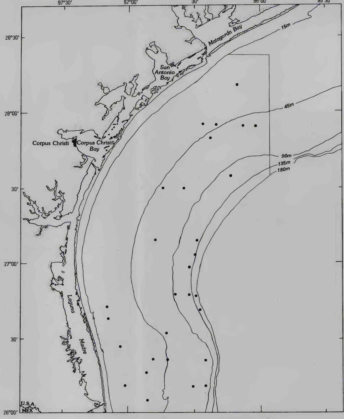
Distribution of an unidentified cirratulid.
