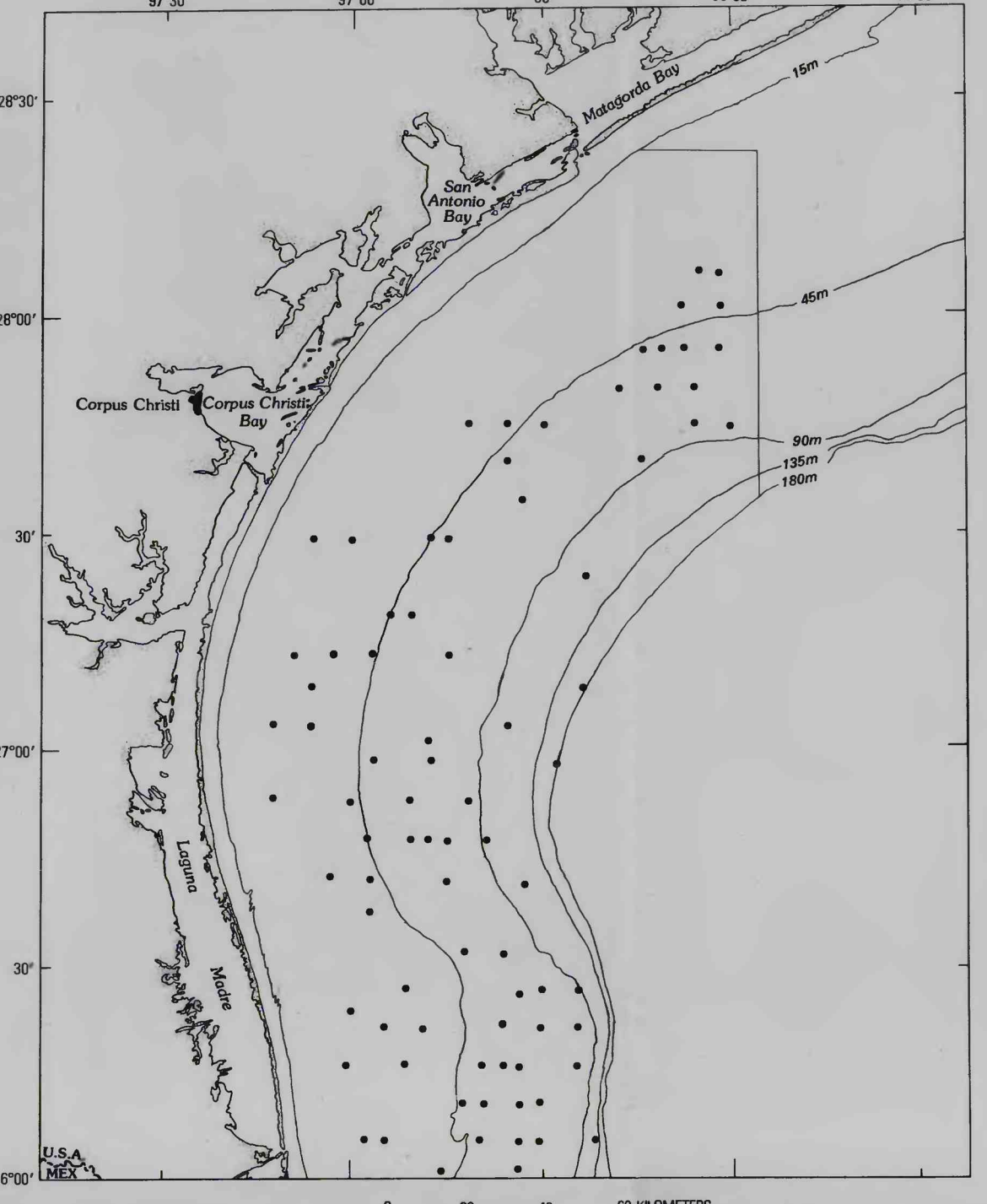
Distribution of an unidentified ophiurid.
