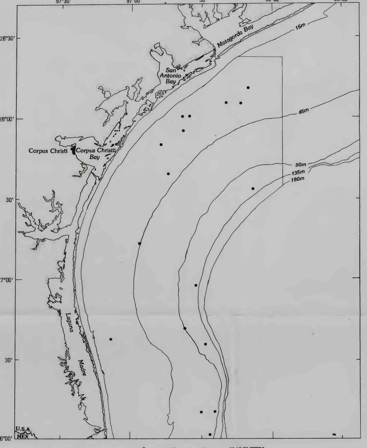
Distribution of Sthenelais sp.
