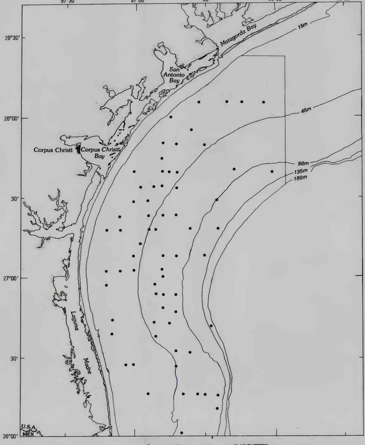
Distribution of Cossura delta .
