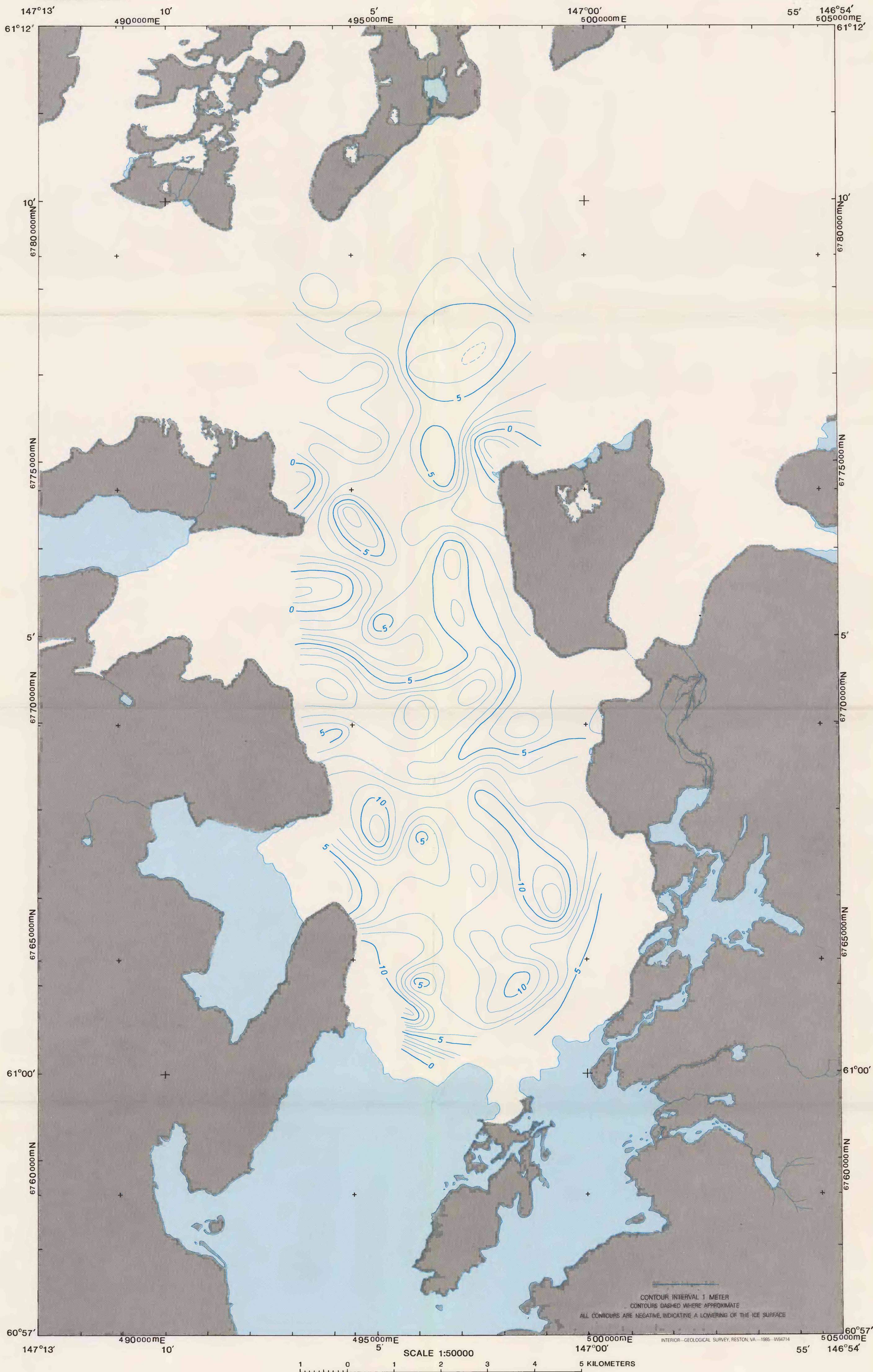
CHANGE IN SURFACE ALTITUDE FROM AUGUST 29, 1977, TO AUGUST 26, 1978
