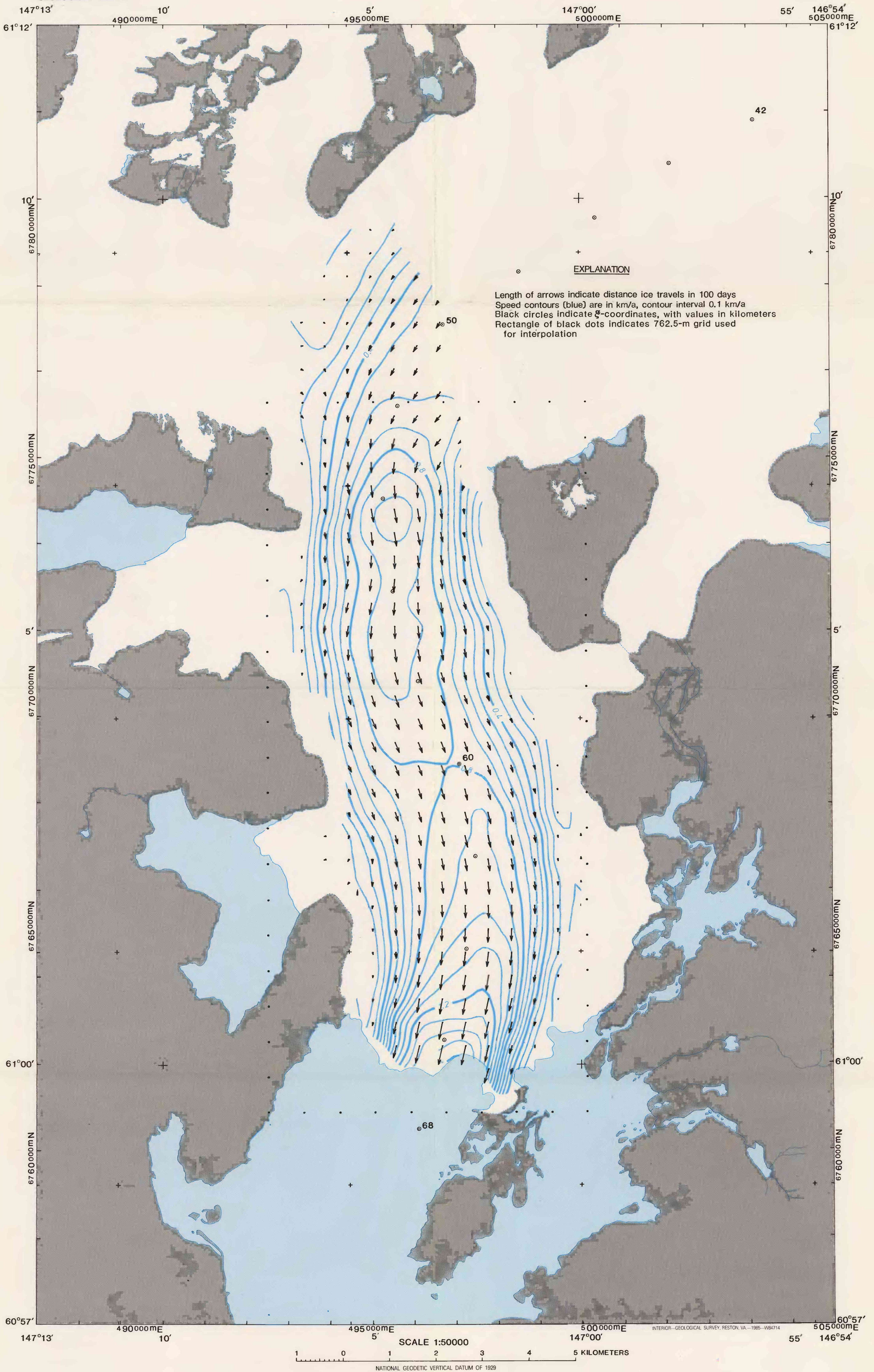
VELOCITY AND SPEED DURING THE MEASUREMENT YEAR, FOR THE LOWER COLUMBIA GLACIER
