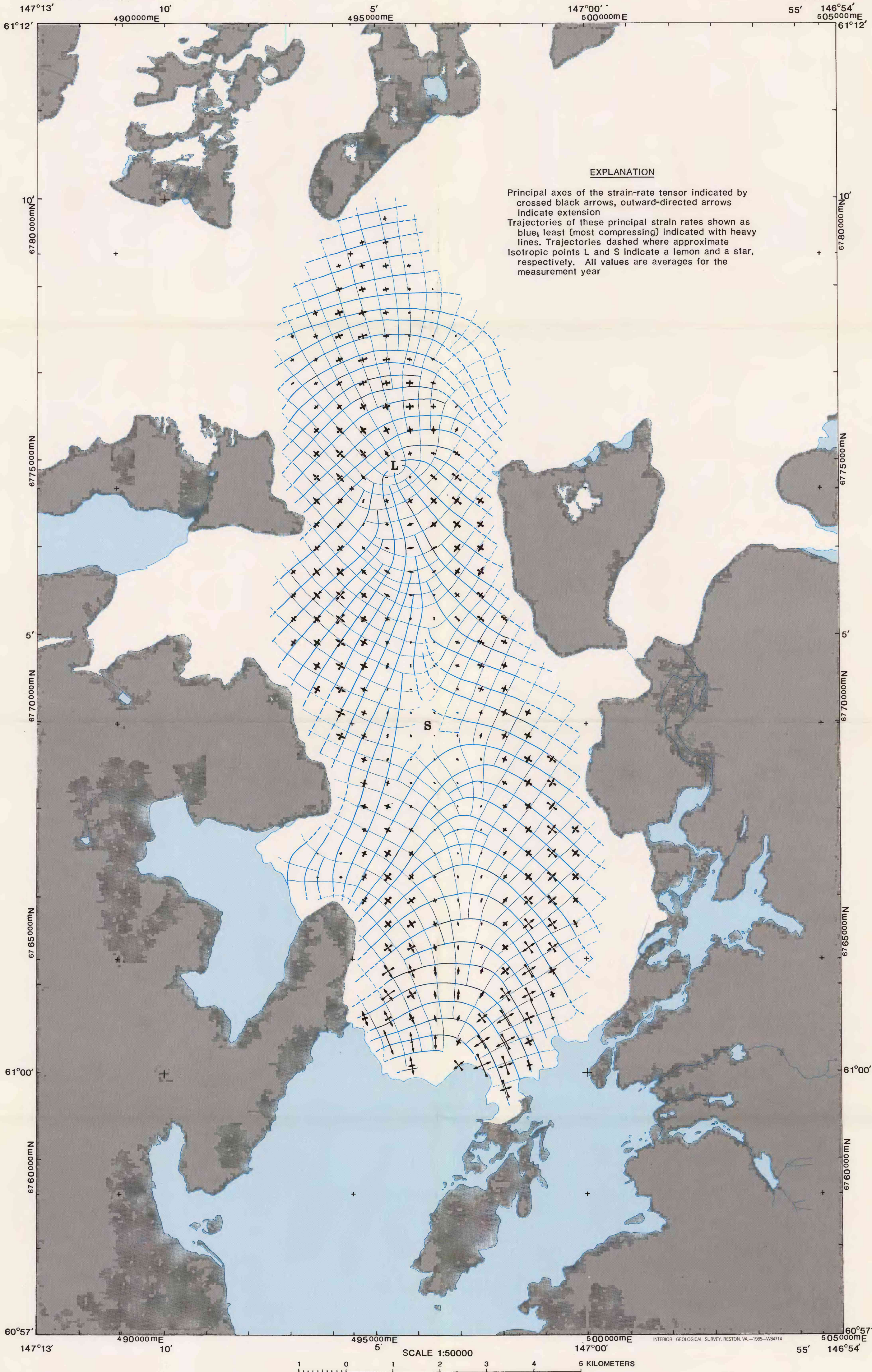
DIRECTION AND MAGNITUDE OF THE PRINCIPAL AXES OF THE STRAIN RATE TENSOR, AND TRAJECTORIES OF THESE AXES
