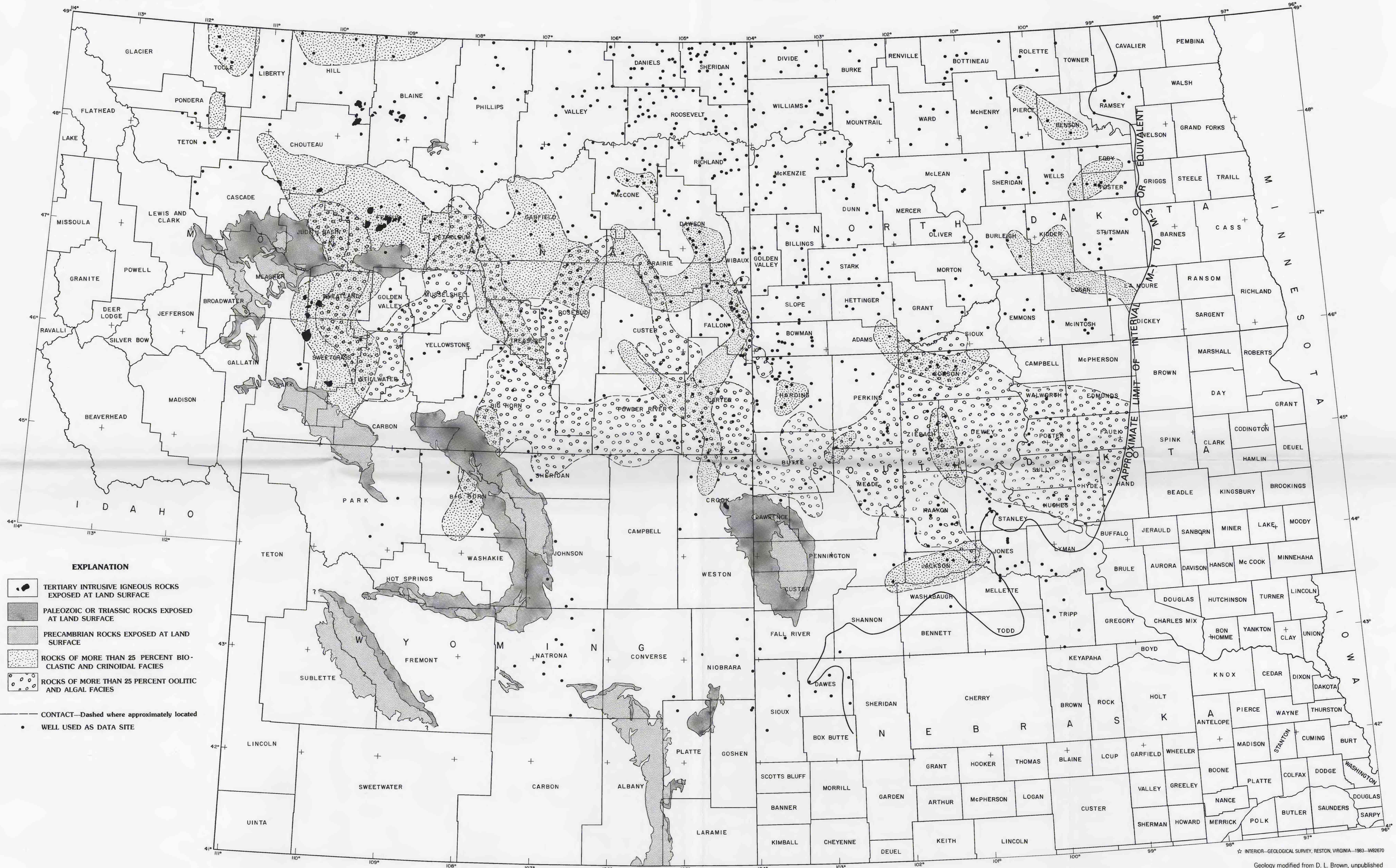
MAP SHOWING OOLITIC-ALGAL AND CRINOIDAL-BIOCLASTIC FACIES IN MADISON LIMESTONE INTERVAL M-1 TO M-3 AND EQUIVALENT ROCKS (MISSISSIPPIAN) IN PARTS OF MONTANA, NORTH DAKOTA, SOUTH DAKOTA, AND WYOMING
