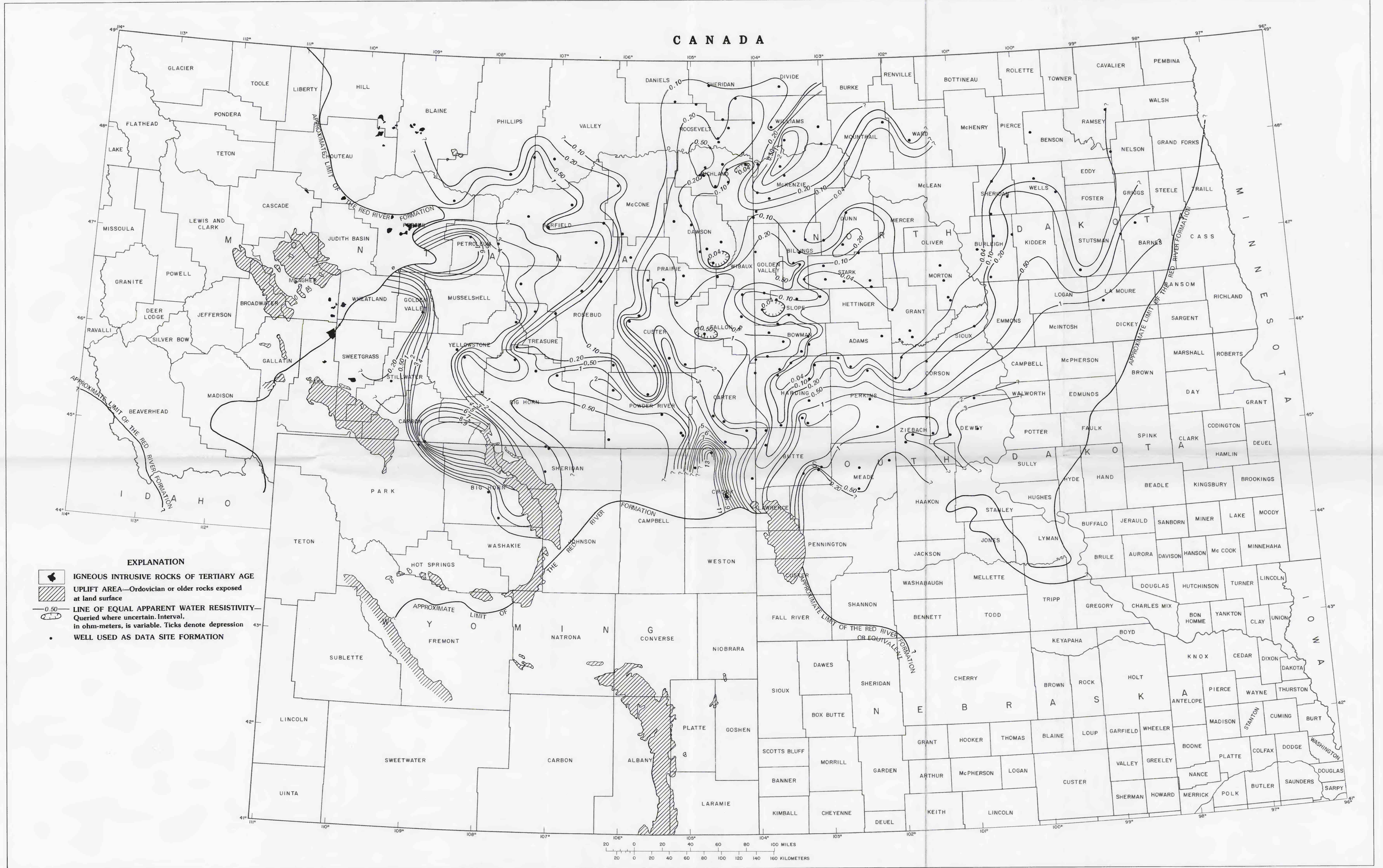
MAP SHOWING APPARENT WATER RESISTIVITY (R wa ) OF THE RED RIVER FORMATION (ORDOVICIAN) IN MONTANA, NORTH DAKOTA, SOUTH DAKOTA, AND WYOMING
