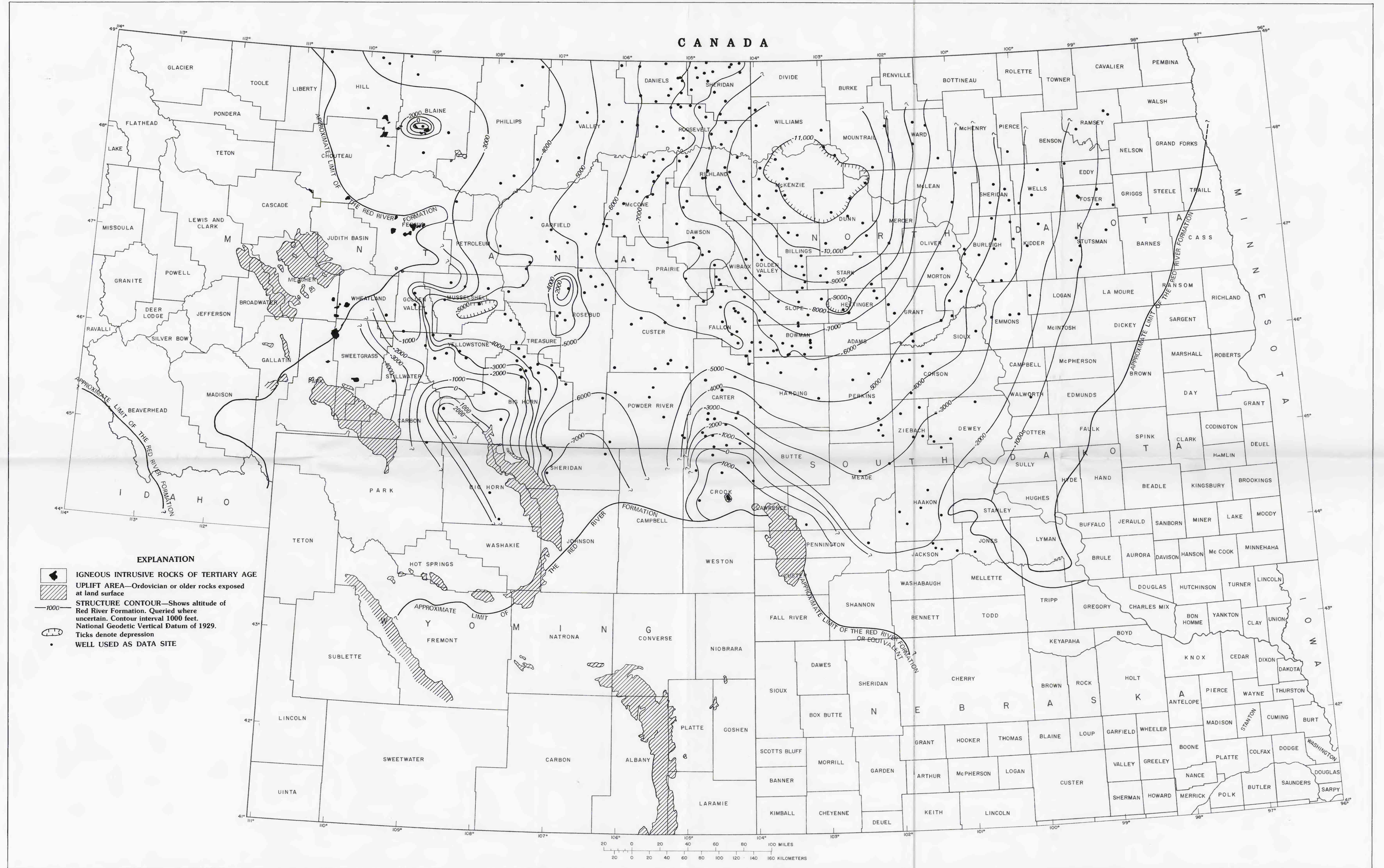
MAP SHOWING ALTITUDE AND CONFIGURATION OF THE TOP OF THE RED RIVER FORMATION (ORDOVICIAN) IN MONTANA, NORTH DAKOTA, SOUTH DAKOTA, AND WYOMING
