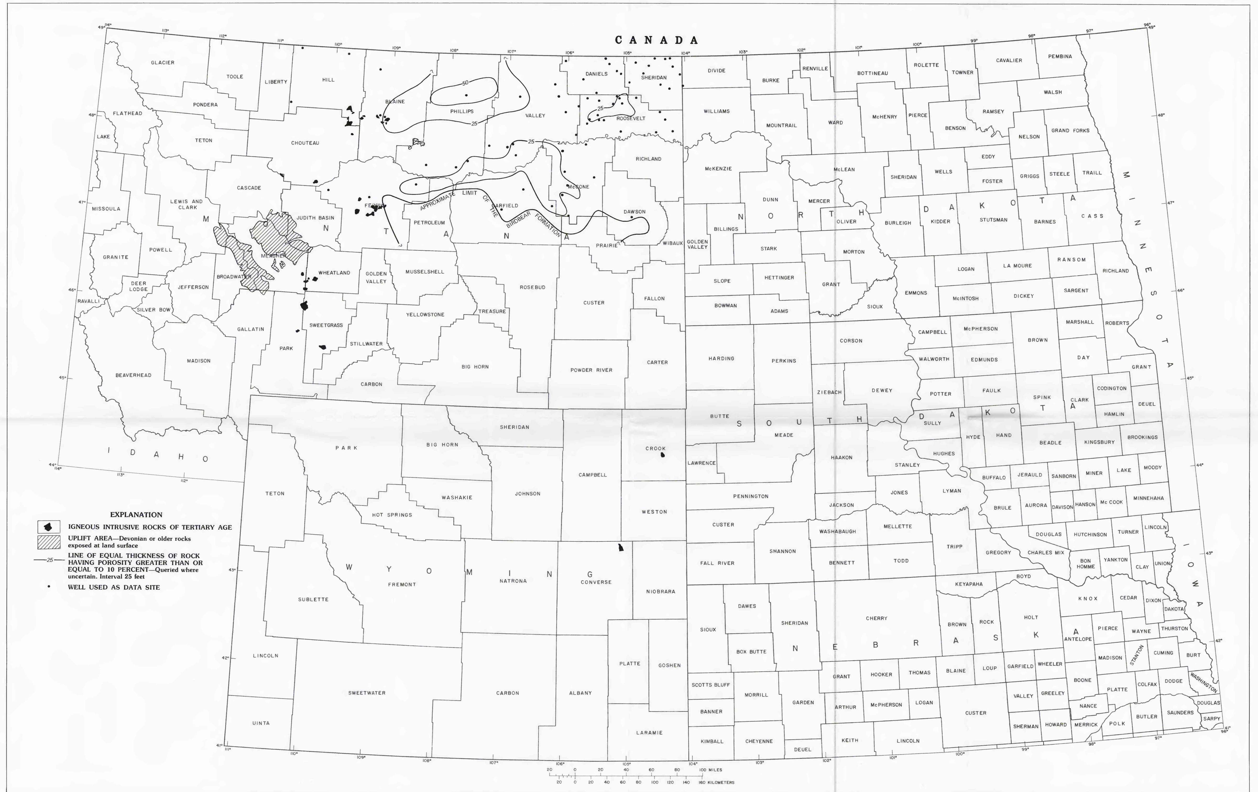
MAP SHOWING THICKNESS OF ROCK HAVING POROSITY GREATER THAN OR EQUAL TO TEN PERCENT IN THE BIRDBEAR FORMATION (UPPER DEVONIAN), IN PARTS OF MONTANA
