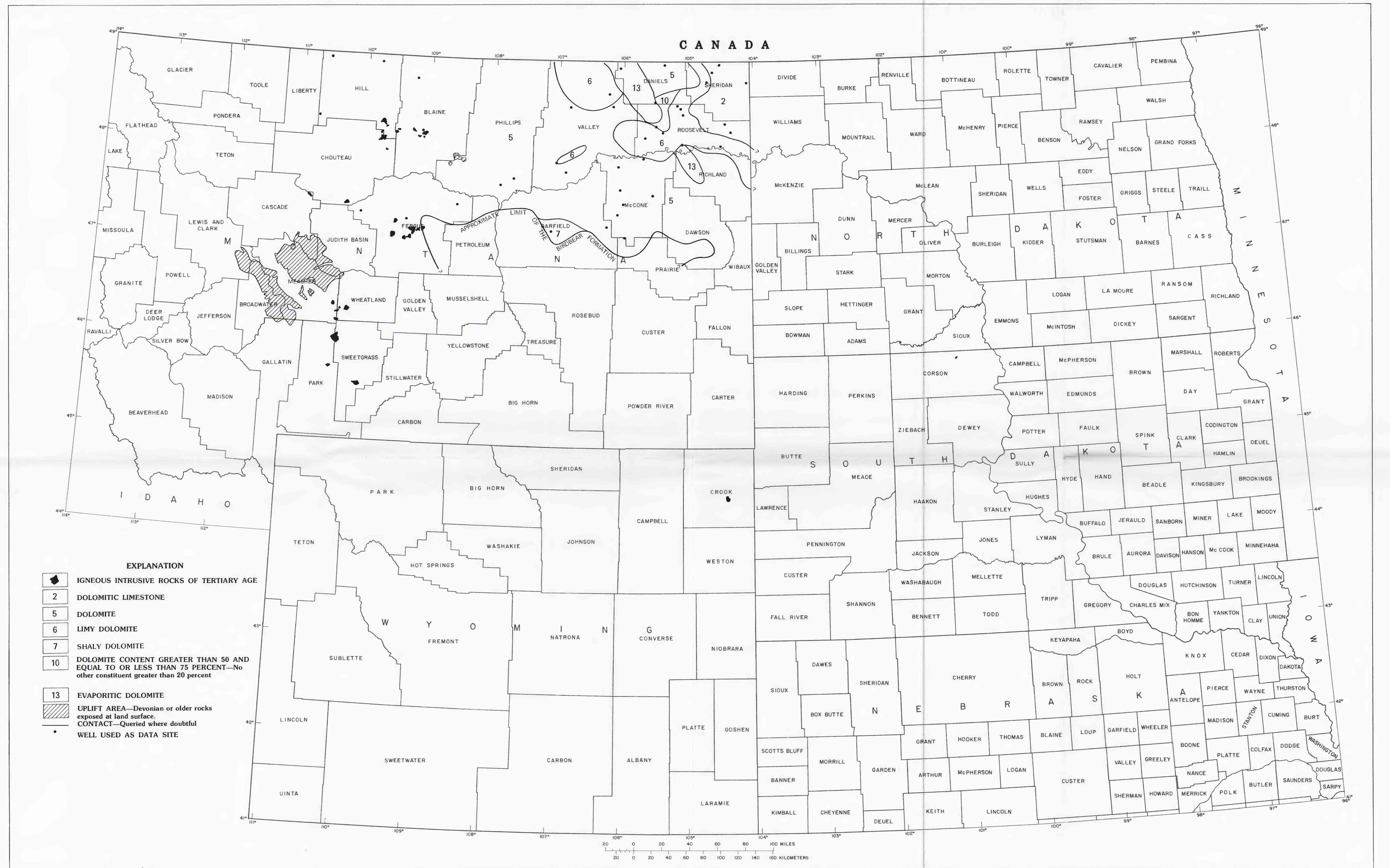
MAP SHOWING ROCK TYPES OF THE BIRDBEAR FORMATION (UPPER DEVONIAN), IN PARTS OF MONTANA
