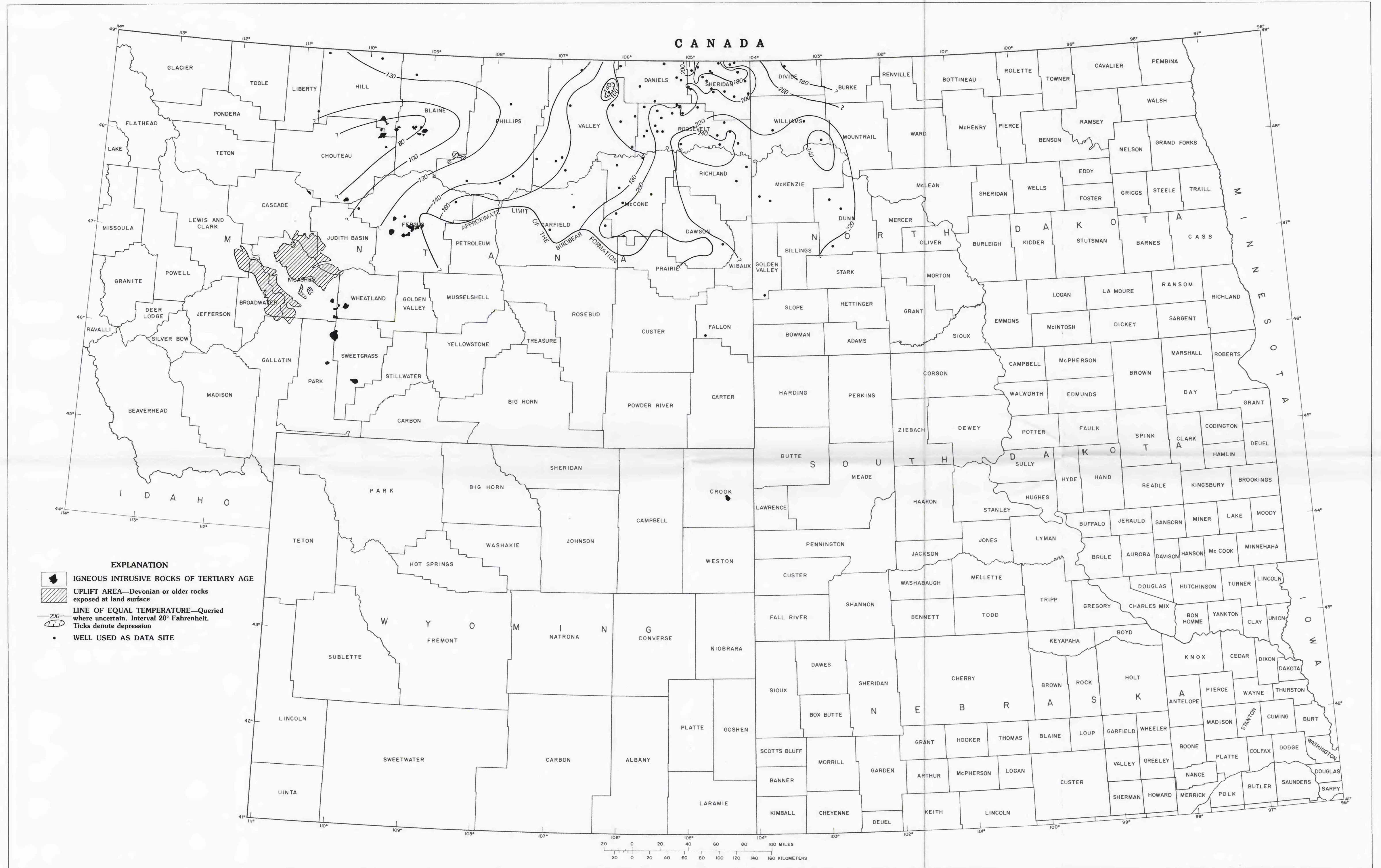
MAP SHOWING TEMPERATURE OF GROUND WATER IN THE BIRDBEAR FORMATION (UPPER DEVONIAN), IN DEGREES FAHRENHEIT, IN PARTS OF MONTANA AND NORTH DAKOTA
