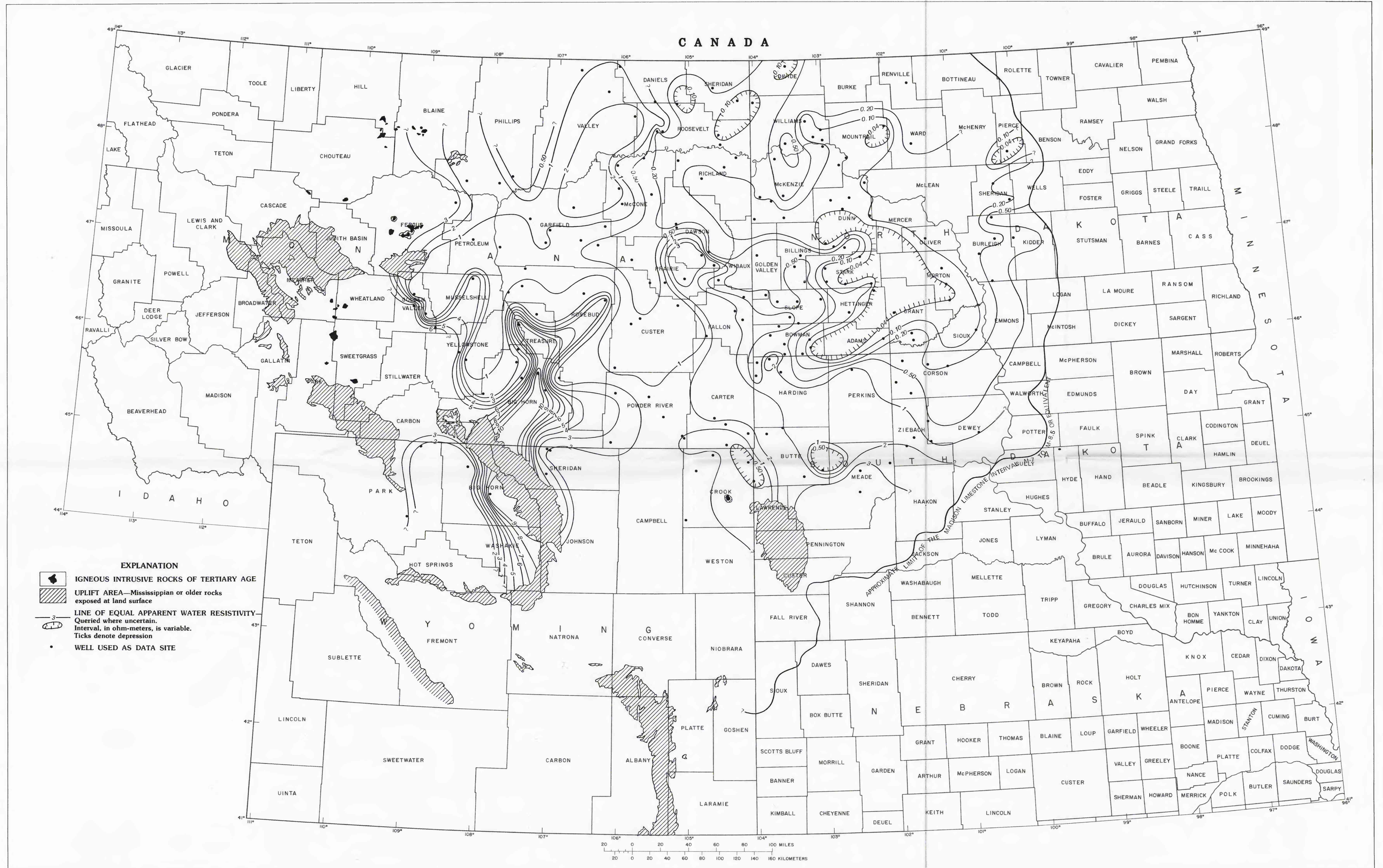
MAP SHOWING APPARENT WATER RESISTIVITY (R wa ) OF THE MADISON LIMESTONE INTERVAL M-7 TO M-8.5 (MISSISSIPPIAN), IN MONTANA, NORTH DAKOTA, SOUTH DAKOTA, AND WYOMING
