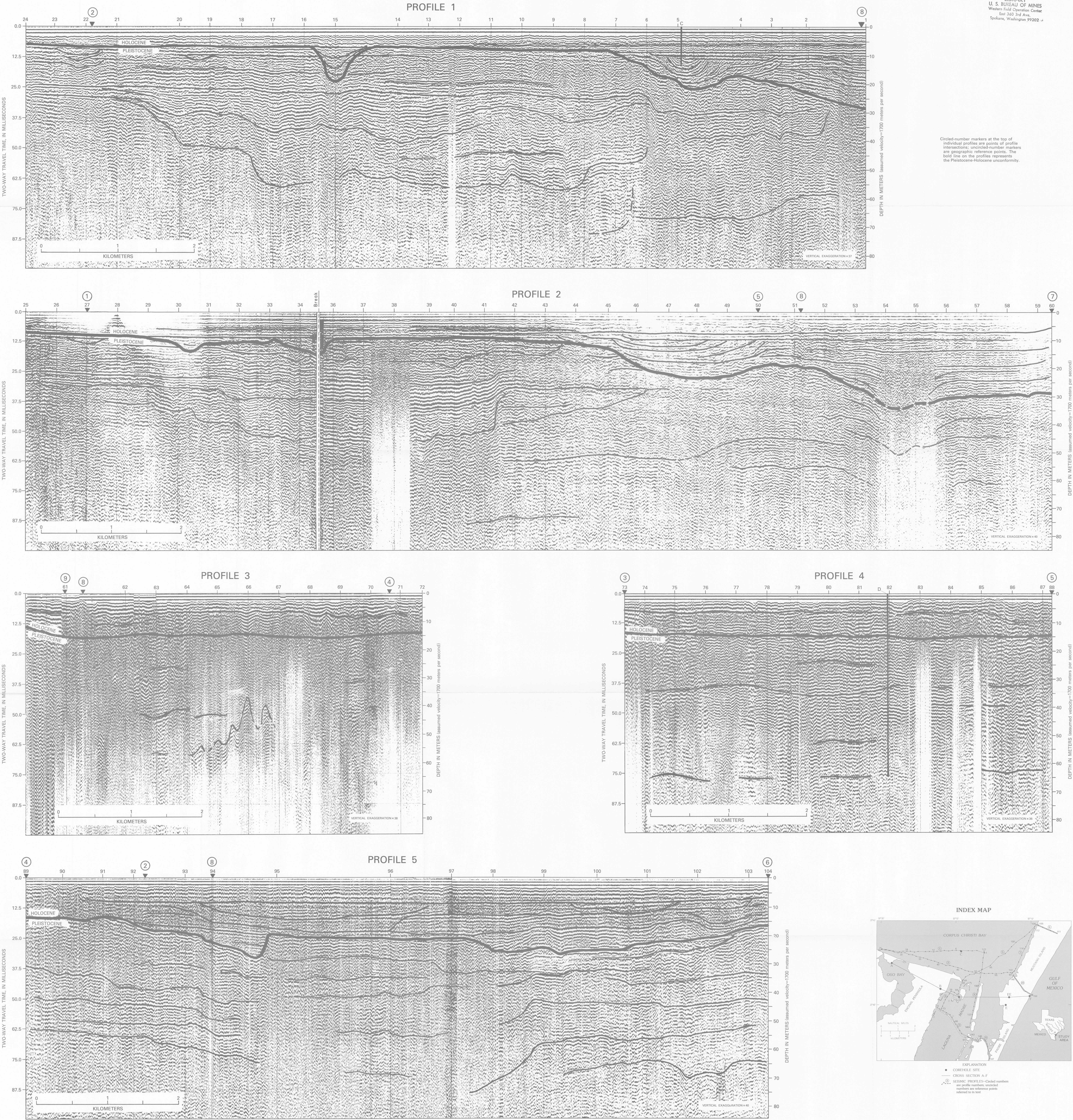
HIGH-RESOLUTION SEISMIC-REFLECTION PROFILES 1-5 OF THE MUSTANG ISLAND-CORPUS CHRISTI BAY AREA, SOUTH TEXAS GULF COAST
