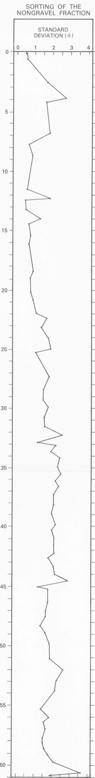
LITHOLOGIC AND SUPPLEMENTAL LOGS OF CORE EE, FROM THE MUSTANG ISLAND-CORPUS CHRISTI BAY AREA, SOUTH TEXAS GULF COAST
