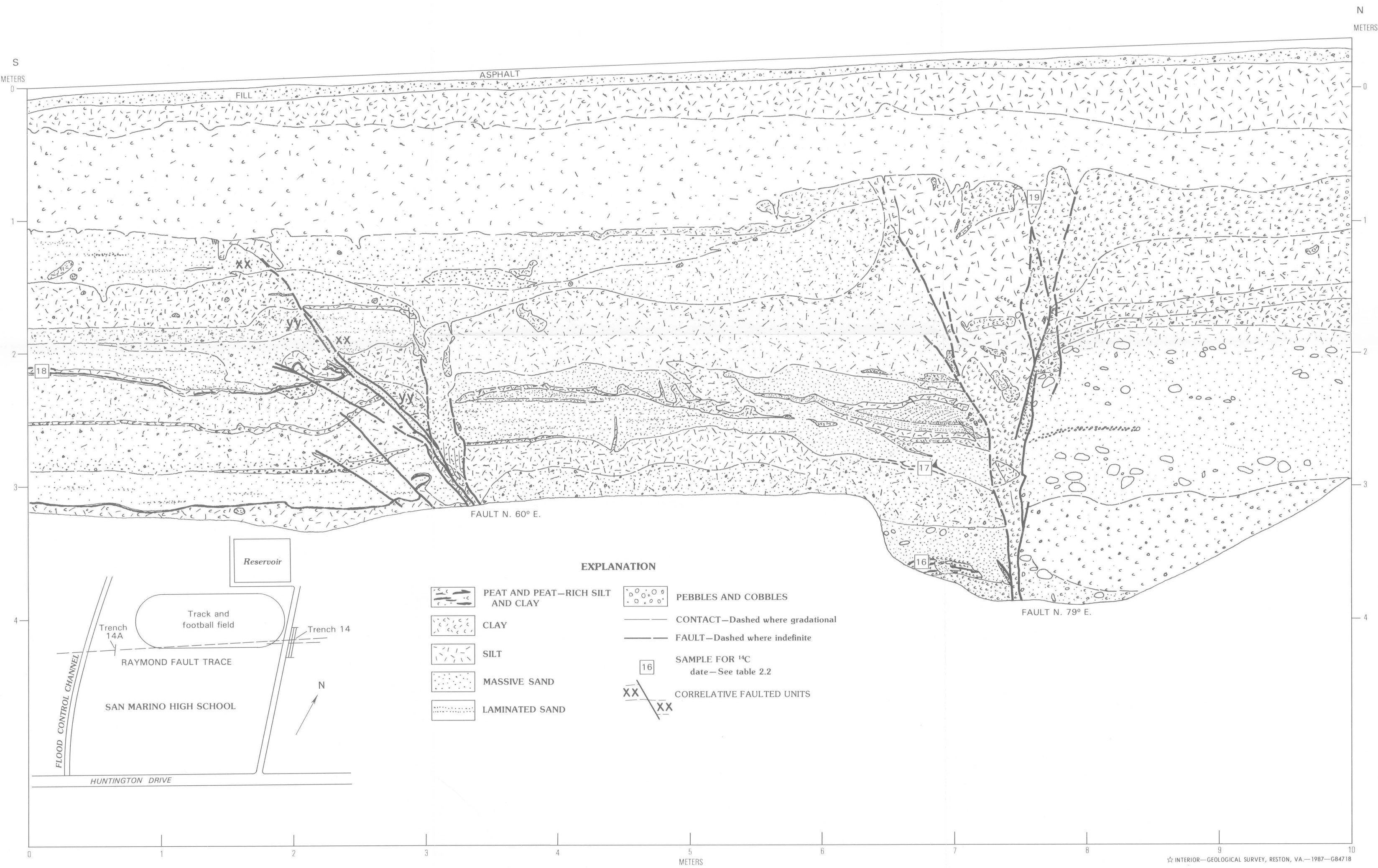
LOG OF TRENCH 14, SAN MARINO HIGH SCHOOL, SAN MARINO
