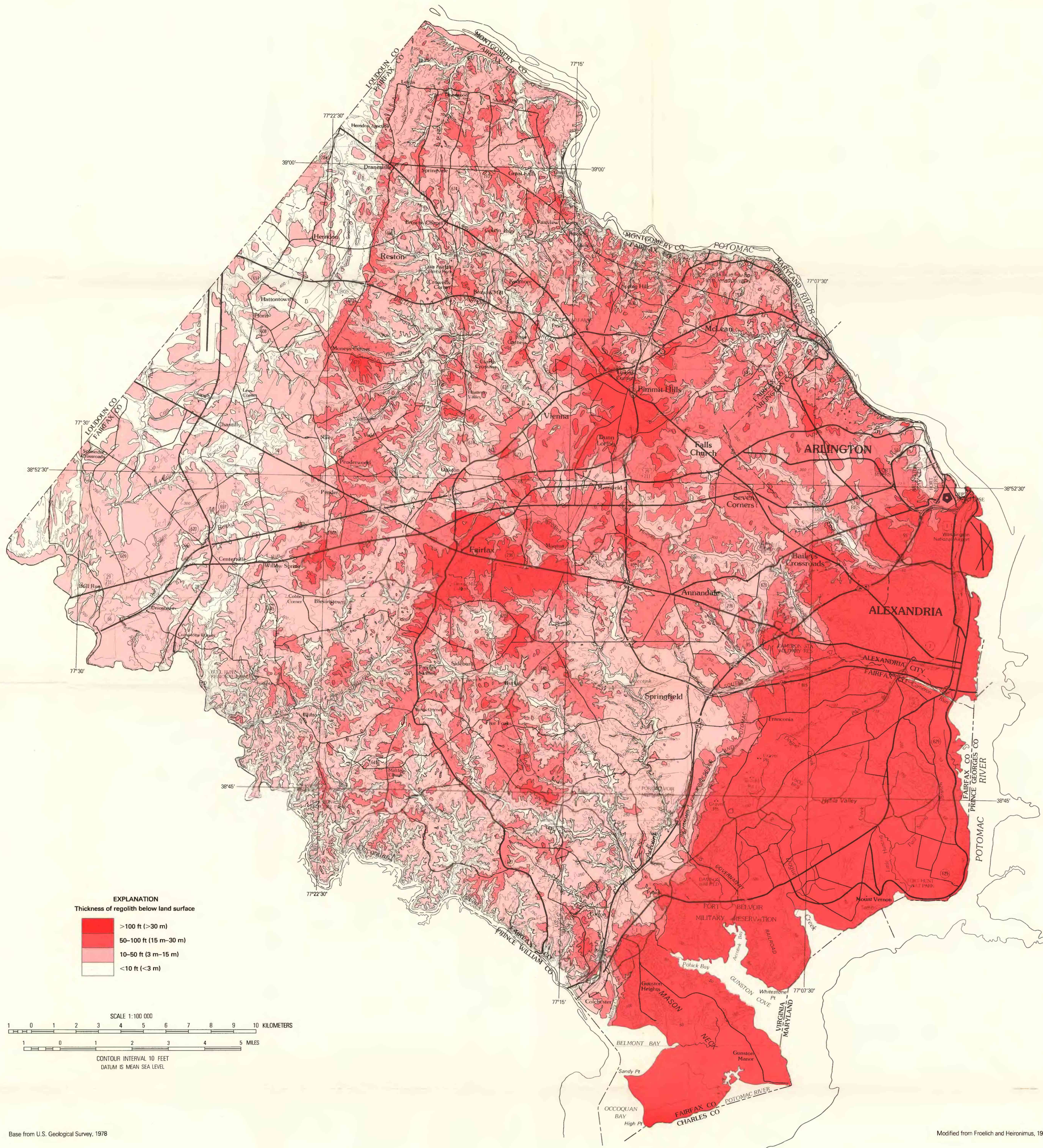
REGOLITH THICKNESS MAP OF FAIRFAX COUNTY, VIRGINIA
