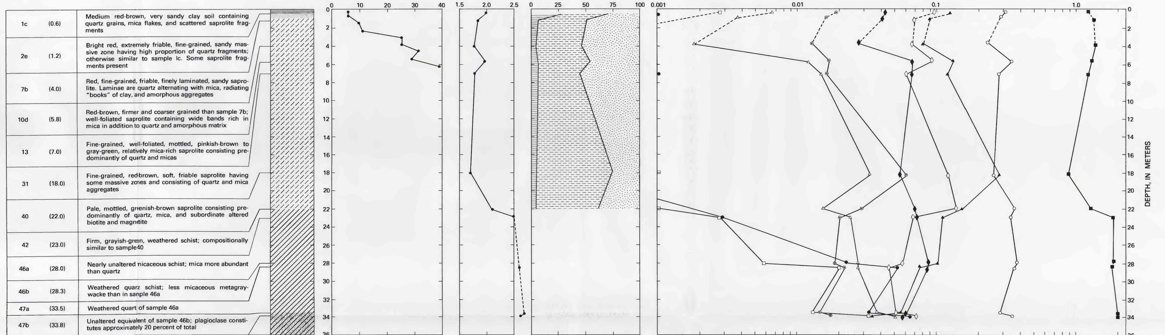
B. METAGRAYWACKE (CORE SITE F3) OF THE PETERS CREEK SCHIST
