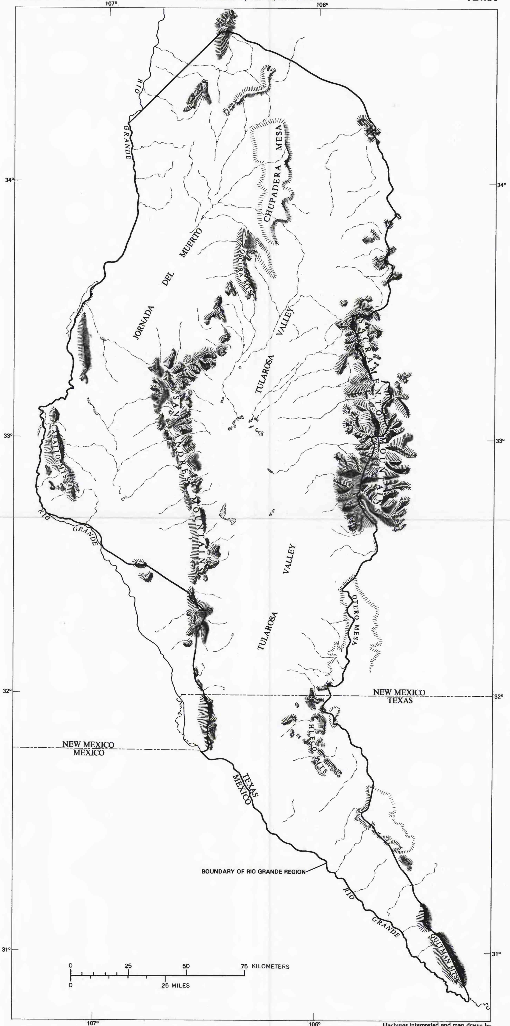
MAP SHOWING PHYSIOGRAPHIC FEATURES OF THE RIO GRANDE REGION, NEW MEXICO AND TEXAS
