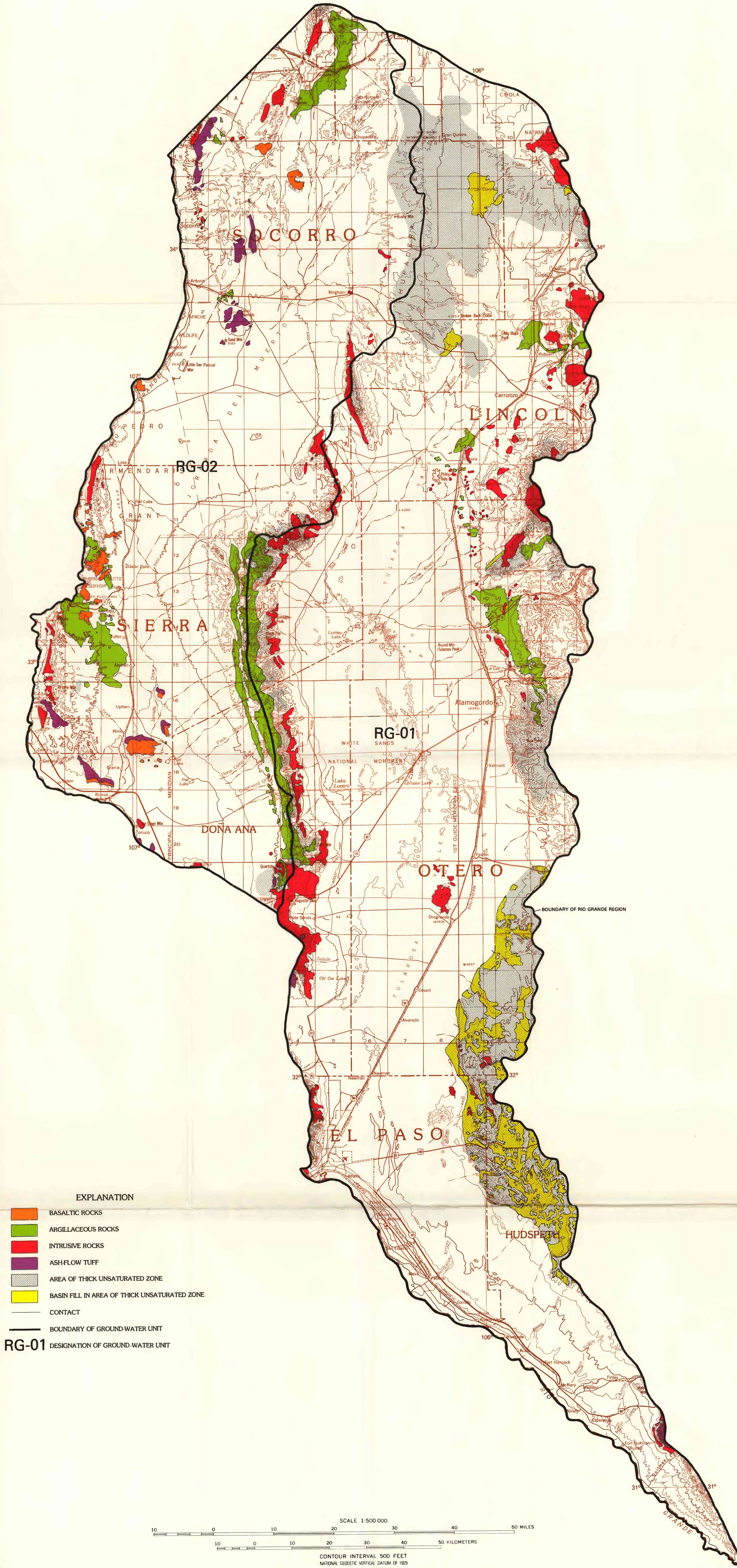
MAP SHOWING POTENTIAL HOST ROCKS AND AREAS OF THICK UNSATURATED ZONES, RIO GRANDE REGION, NEW MEXICO AND TEXAS
