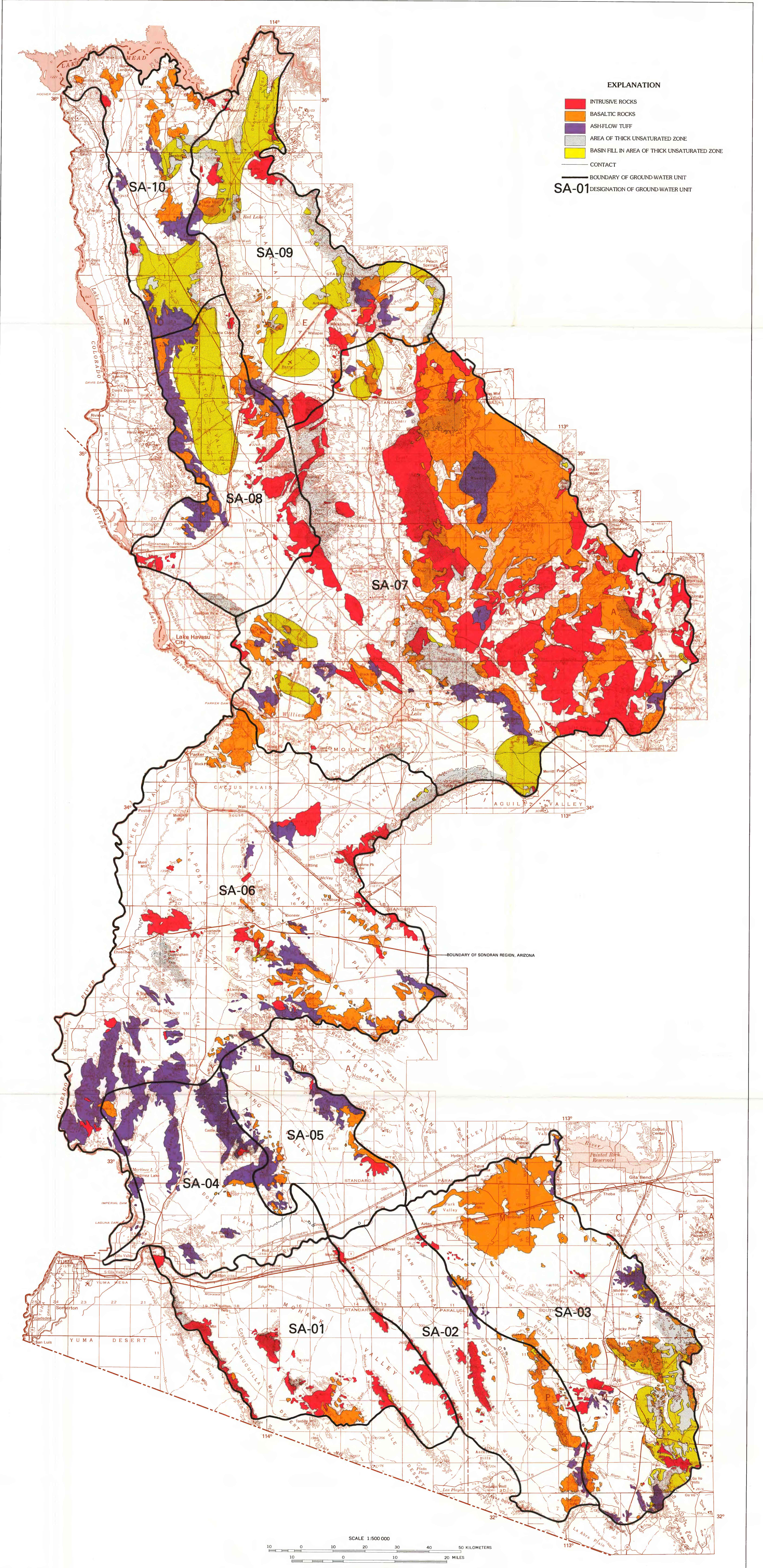
MAP SHOWING POTENTIAL HOST ROCKS AND AREAS OF THICK UNSATURATED ZONES, SONORAN REGION, ARIZONA
