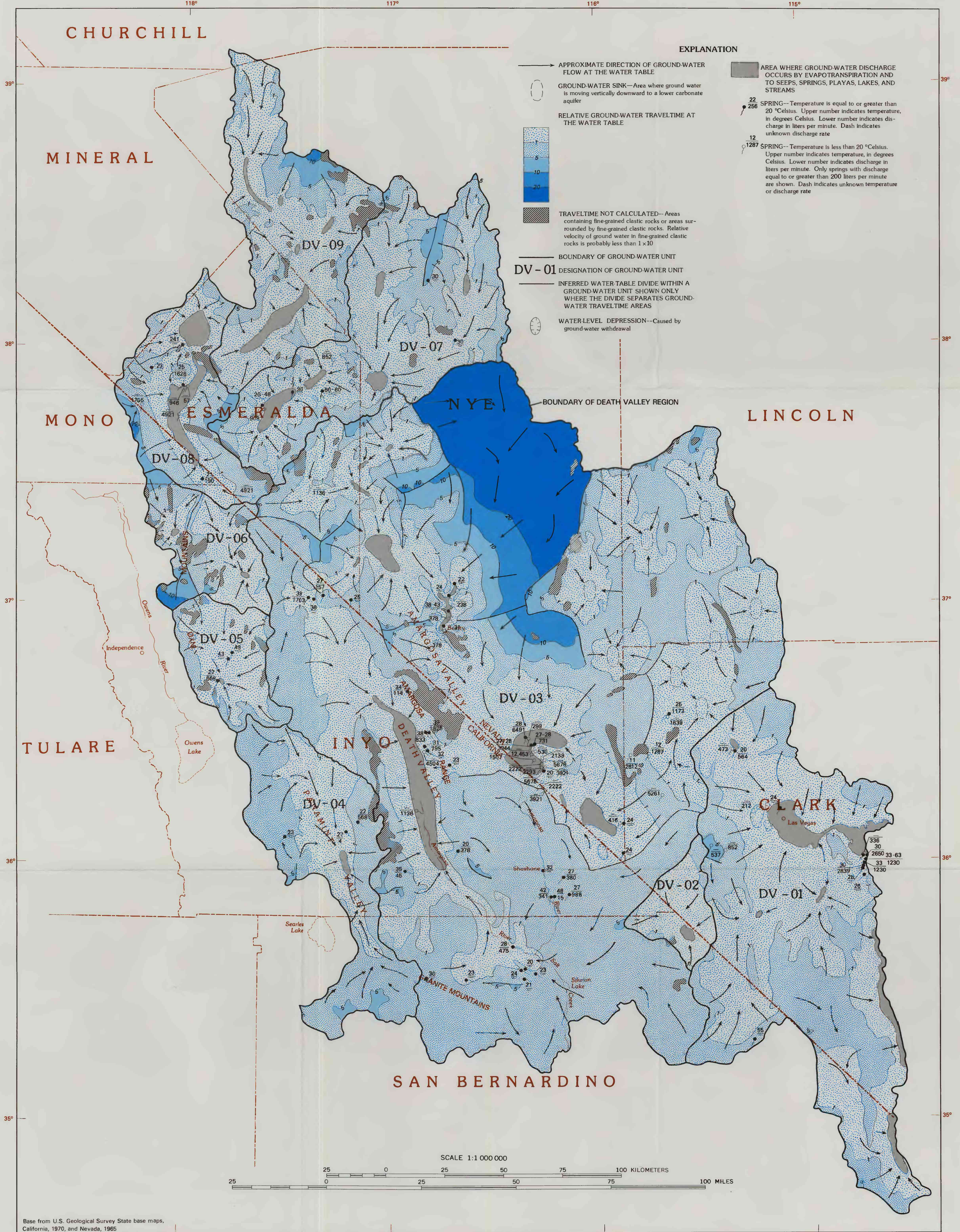
MAP SHOWING RELATIVE GROUND-WATER TRAVELTIME, FLOW PATHS, AND NATURAL DISCHARGE AREAS, DEATH VALLEY REGION, NEVADA AND CALIFORNIA
