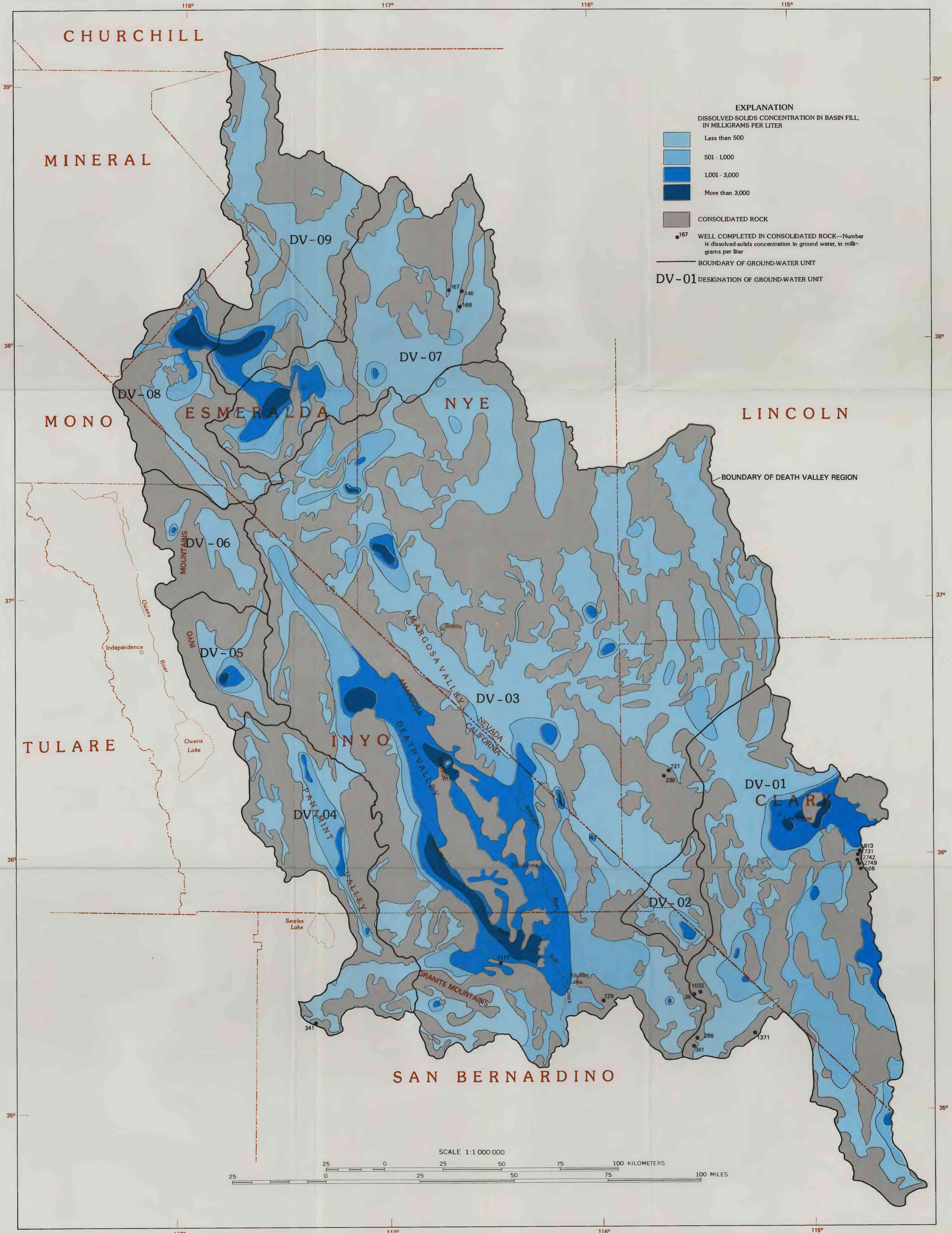
MAP SHOWING DISSOLVED-SOLIDS CONCENTRATION IN GROUND WATER, DEATH VALLEY REGION, NEVADA AND CALIFORNIA
