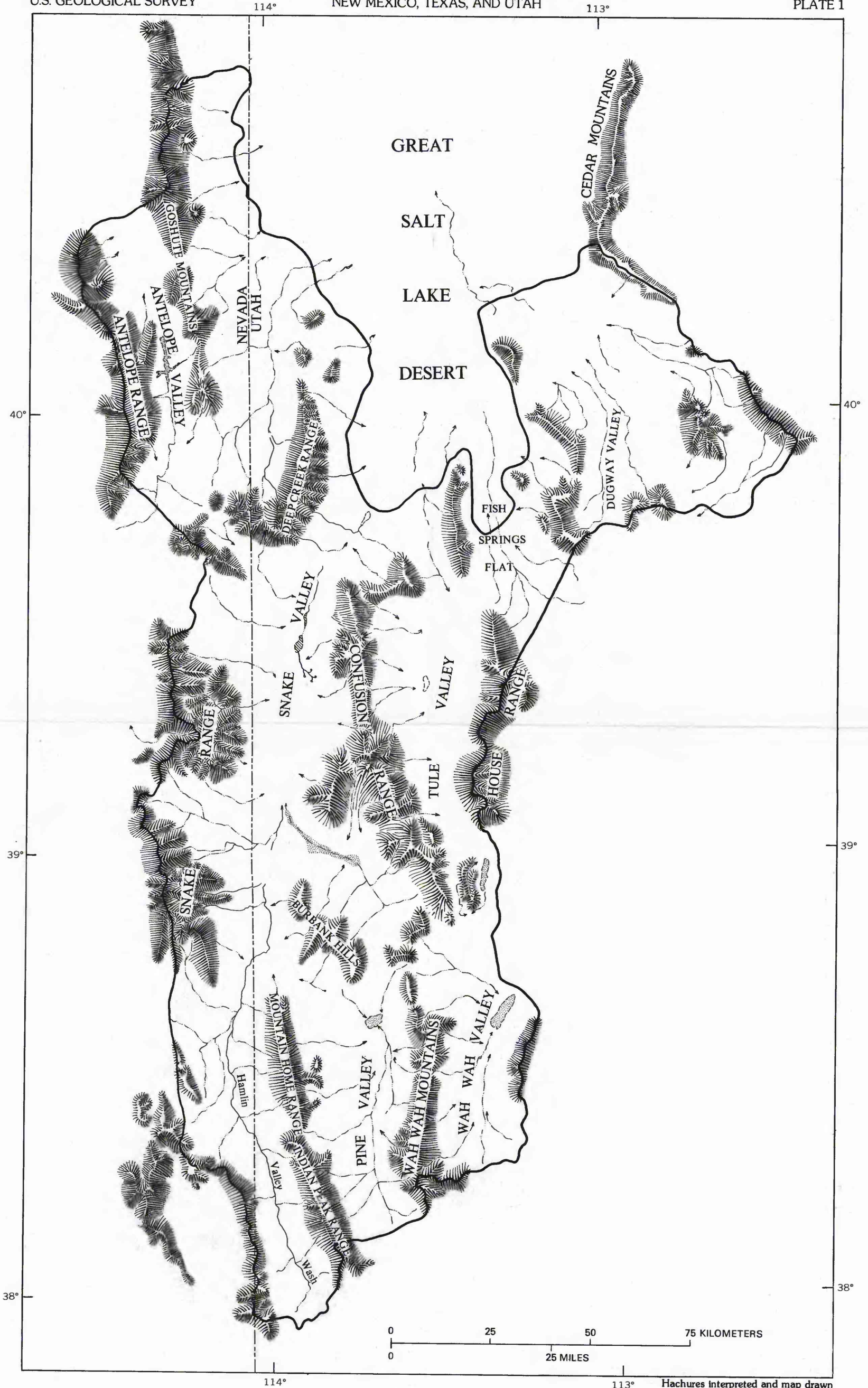
MAP SHOWING PHYSIOGRAPHIC FEATURES OF THE BONNEVILLE REGION, UTAH AND NEVADA
