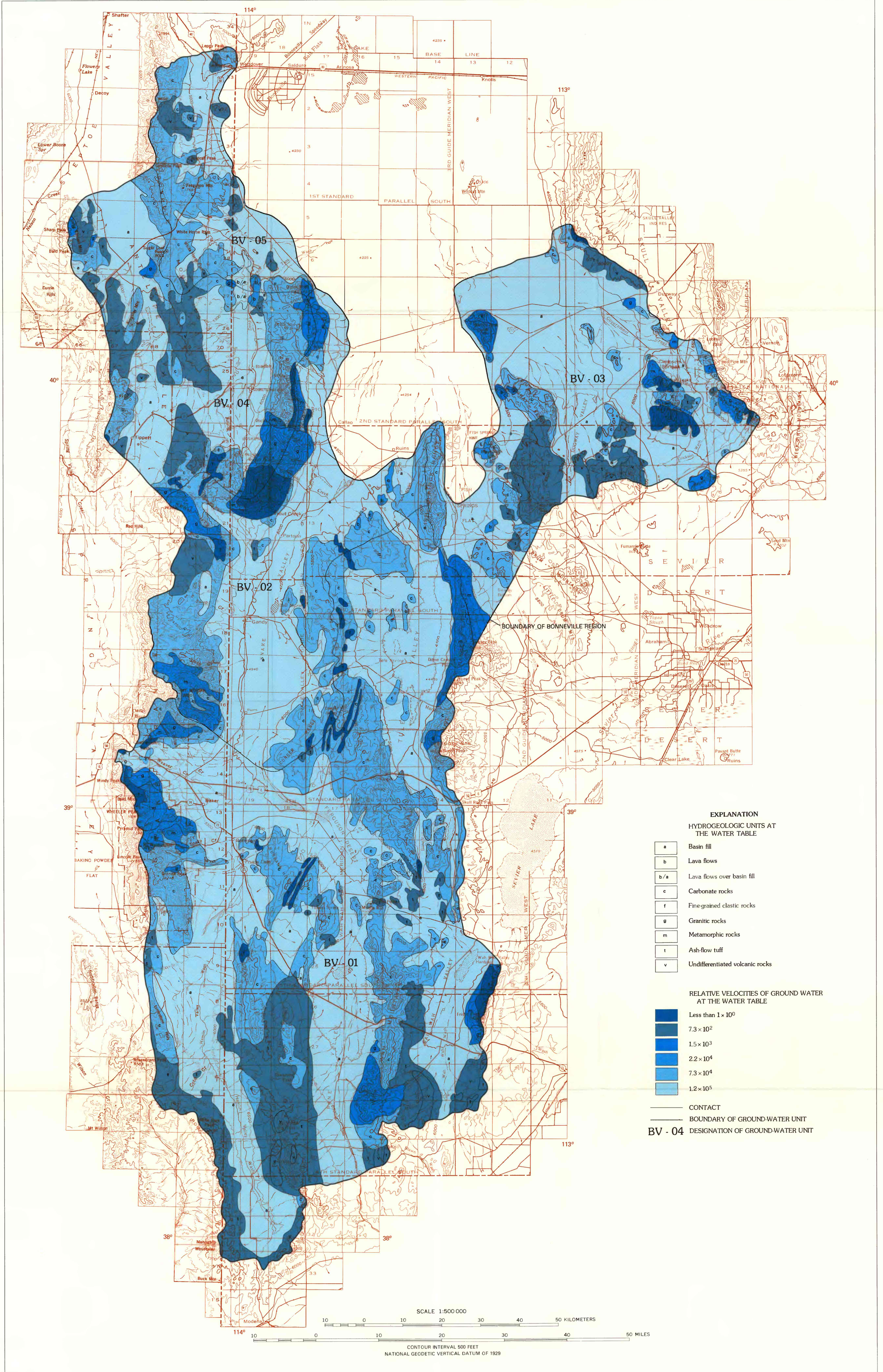
MAP SHOWING HYDROGEOLOGIC UNITS AND RELATIVE VELOCITIES OF GROUND WATER AT THE WATER TABLE, BONNEVILLE REGION, UTAH AND NEVADA
