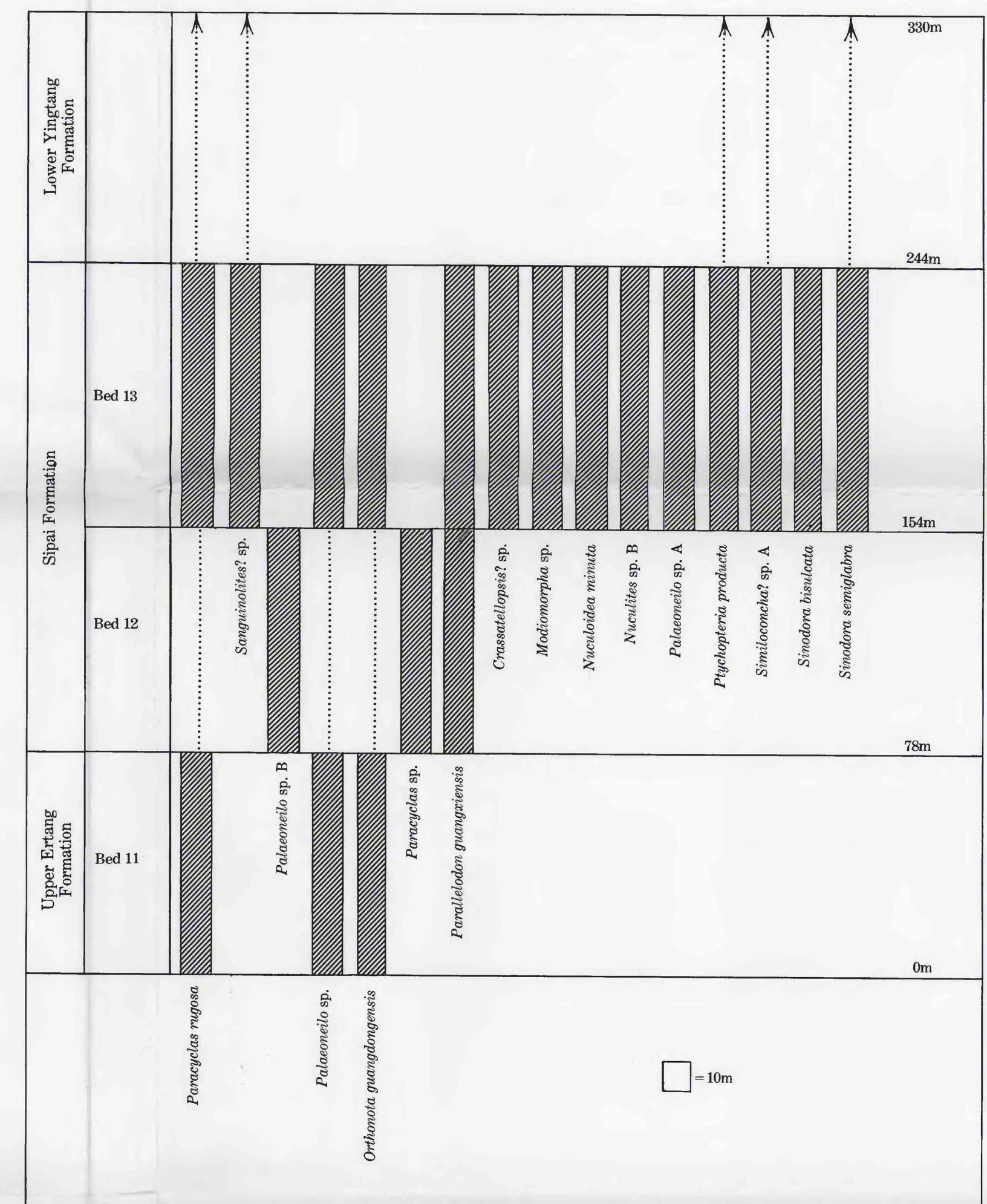
C SIPAII AND UPPER ERTANG FORMATIONS AT SECTION 3
