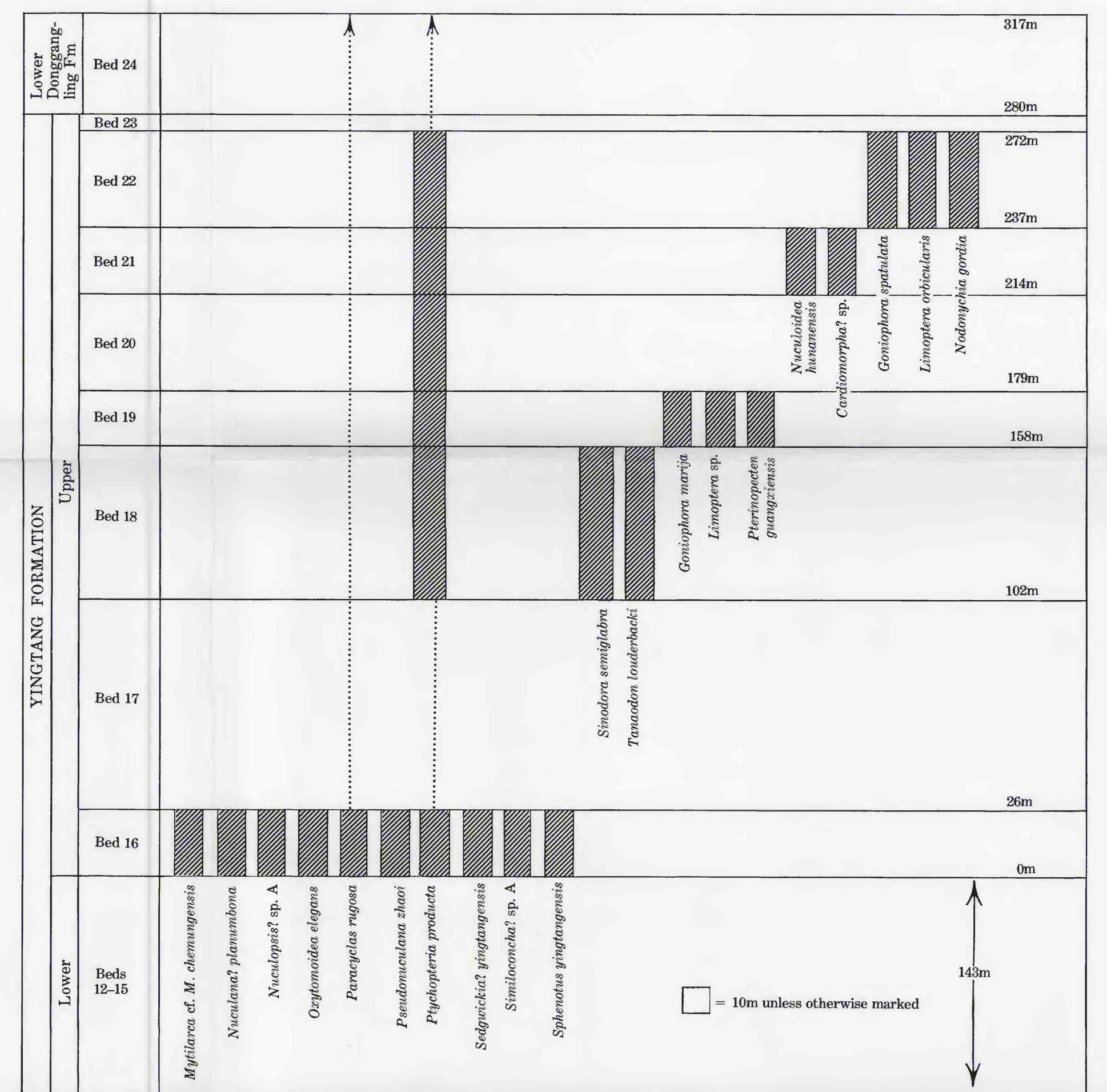
D YINGTANG FORMATION AT SECTION 5
