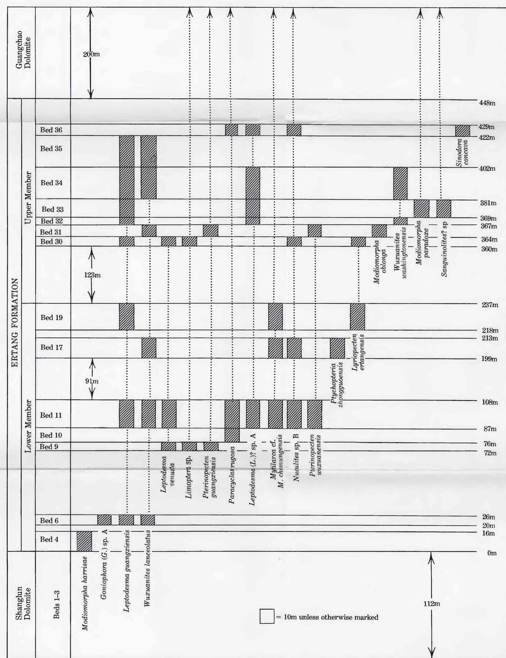
B ERTANG FORMATION AT SECTION 4
