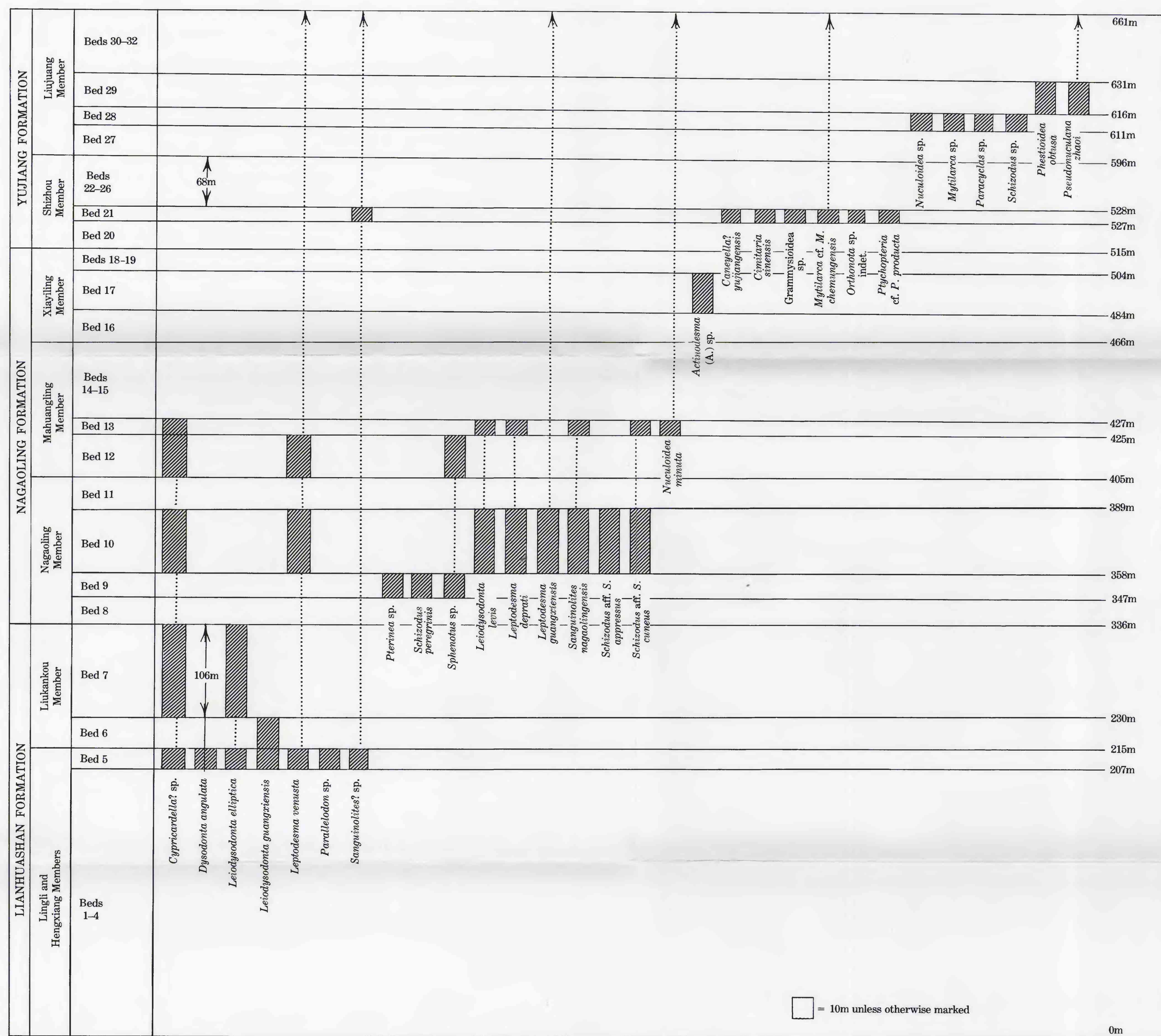
A LIANHUASHAN, NAGAOLING, AND YUJIANG FORMATIONS AT SECTION 1
